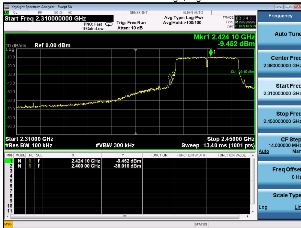
802.11n-HT40: Band Edge, Left Side
