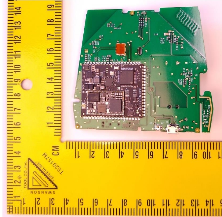
Figure 7: Sensor Relay (ALF-000045 / ALF-000046) BOTTOM Layer, No Cans
