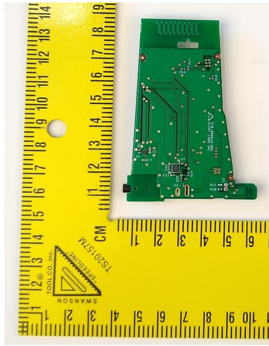
Figure 3: Flowie-O (ALF-000044) BOTTOM Layer
