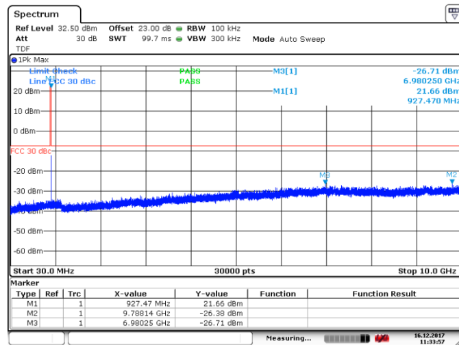
Figure 8.3-5: Conducted spurious emissions outside restricted band, High channel
