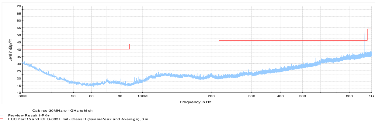
Figure 8.3-14: Cabinet Radiated spurious emissions 30 MHz to 1 GHz, High channel
