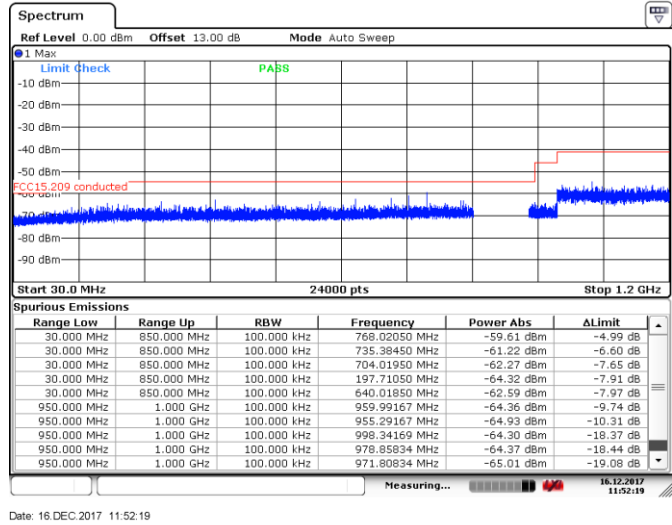
Figure 8.3-7: Conducted spurious emission of restricted band 30 MHz to 1.2 GHz, mid channel
