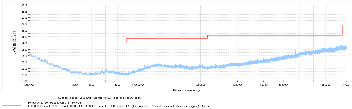
Figure 8.3-12: Cabinet Radiated spurious emissions 30 MHz to 1 GHz, Low channel
