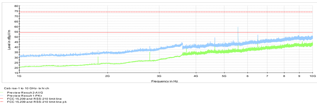
Figure 8.3-17: Cabinet Radiated spurious emissions 1 to10 GHz, High channel
