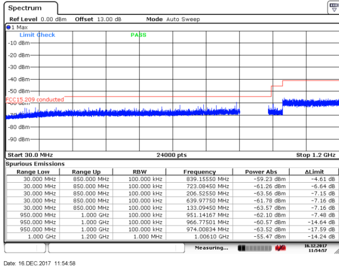
Figure 8.3-6: Conducted spurious emission of restricted band 30 MHz to 1.2 GHz, low channel
