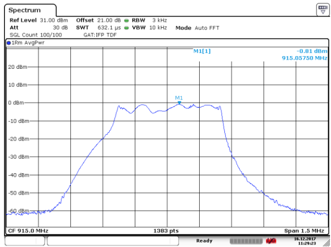
Figure 8.4-2: PSD plot on mid channel
