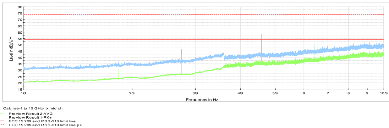
Figure 8.3-16: Cabinet Radiated spurious emissions 1 to10 GHz, Mid channel
