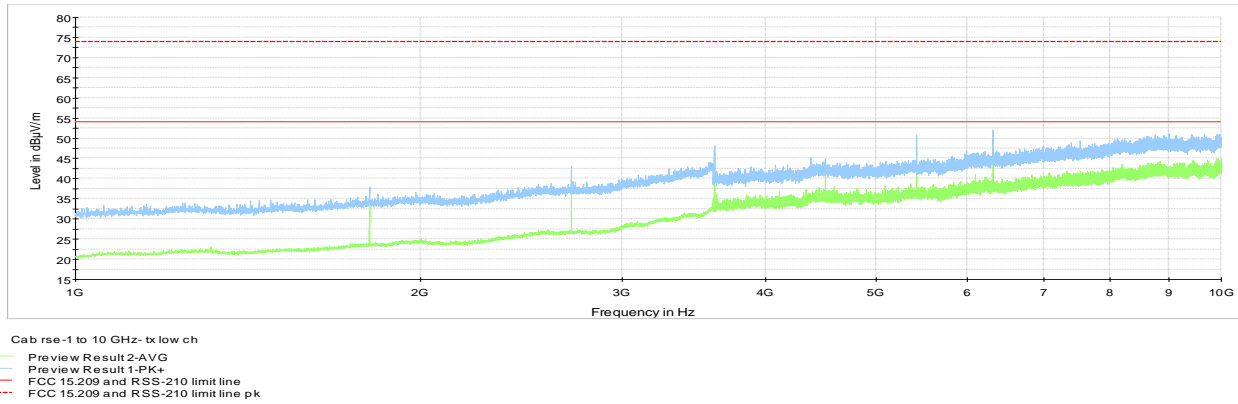
Figure 8.3-15: Cabinet Radiated spurious emissions 1 to10 GHz, Low channel
