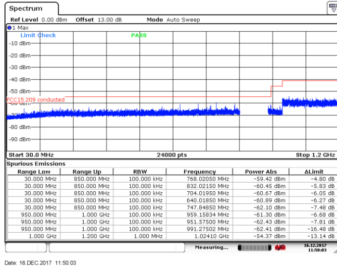
Figure 8.3-8: Conducted spurious emissions of restricted band 30 MHz to 1.2 GHz, High channel
