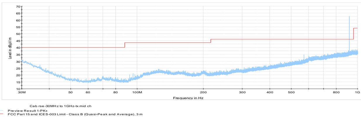
Figure 8.3-13: Cabinet Radiated spurious emissions 30 MHz to 1 GHz, Mid channel
