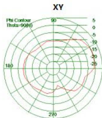
Radiation Pattern 2450MHz
