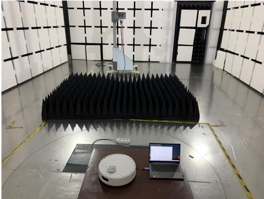
Conducted Measurement
