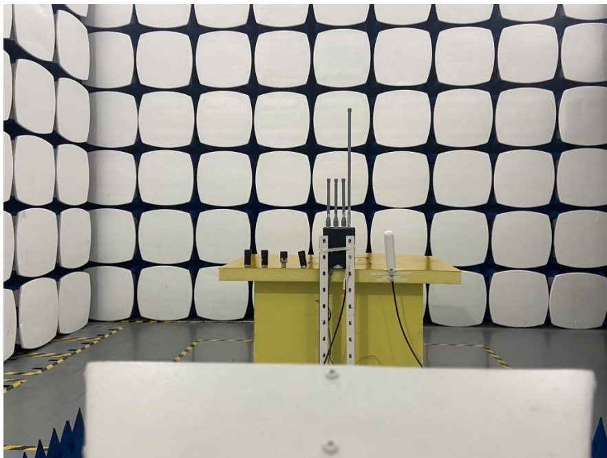
1GHz – 18GHz for Mode 1, Mode 2 & Mode 5
