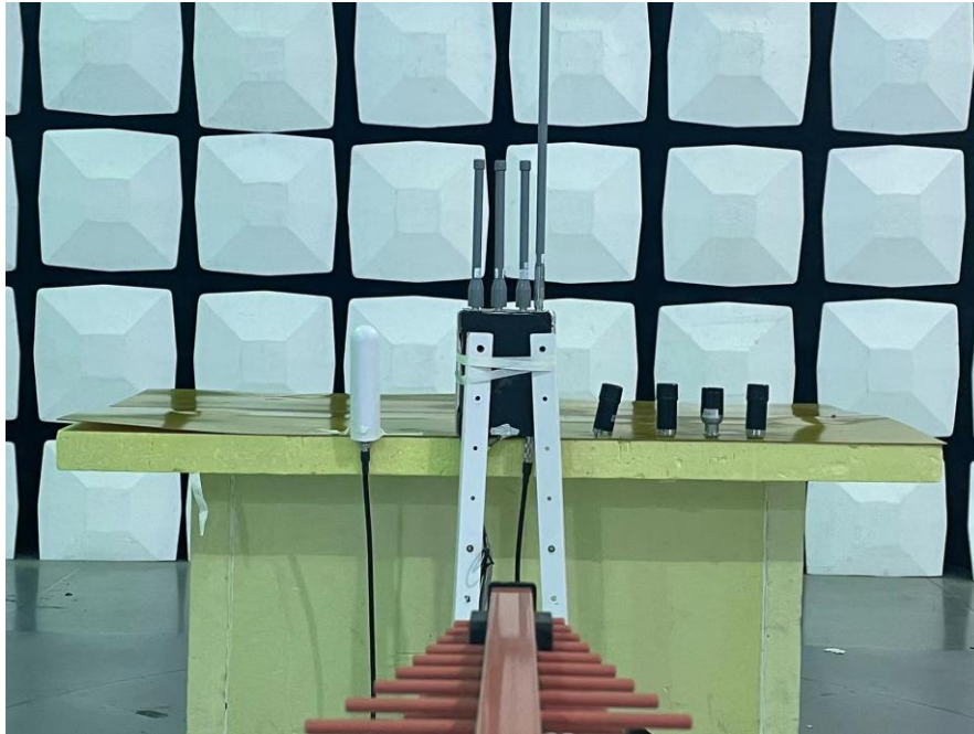
Below 1GHz for Mode 1, Mode 2 & Mode 5
