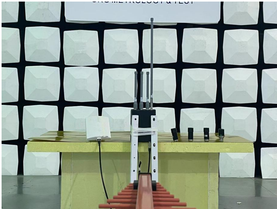
Below 1GHz for Mode 3
