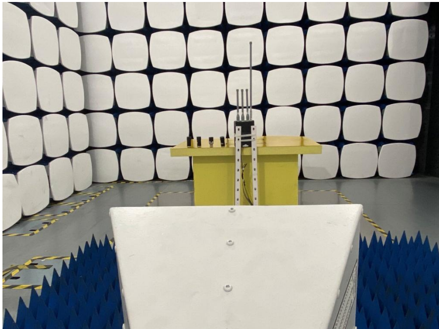
1GHz – 18GHz for Mode 4
