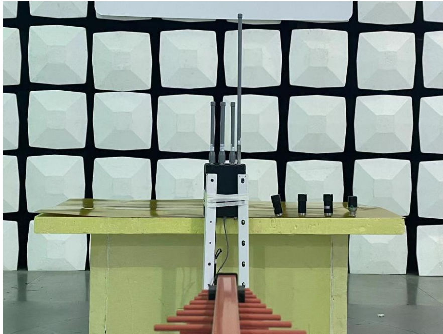
Below 1GHz for Mode 4
