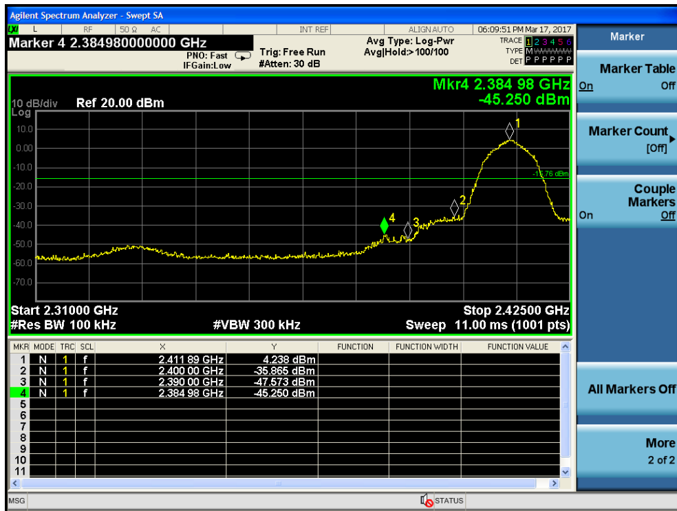
CH: 802.11b-Low
