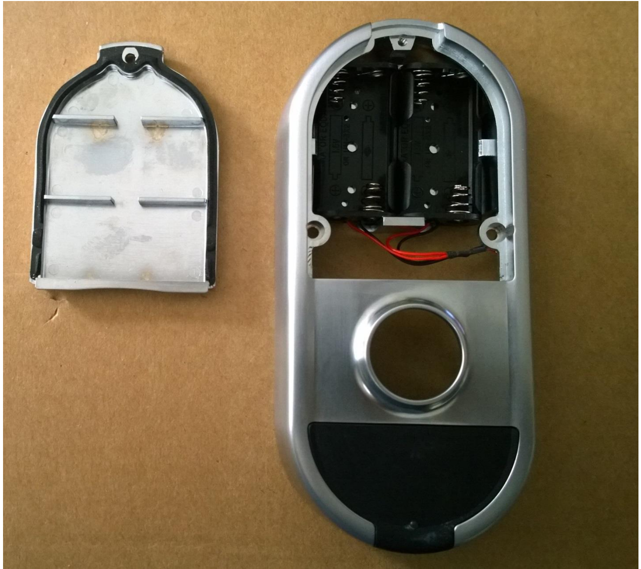
Battery Compartment
