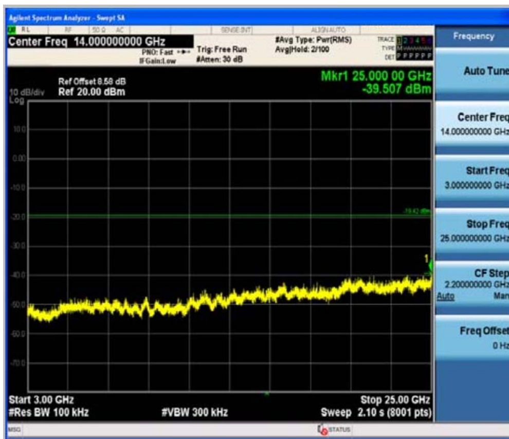
TX 802.11g Mode CH01
