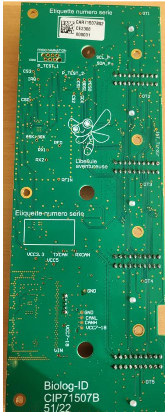
CAR_71507B (RFID) Bottom view
