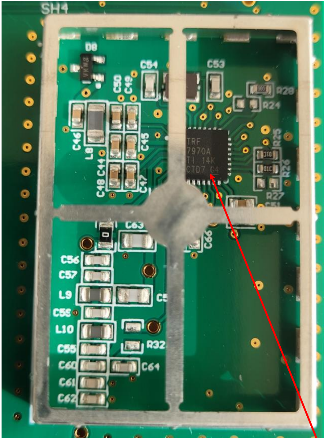
TRF7970A on CAR_71507B (RFID board)
