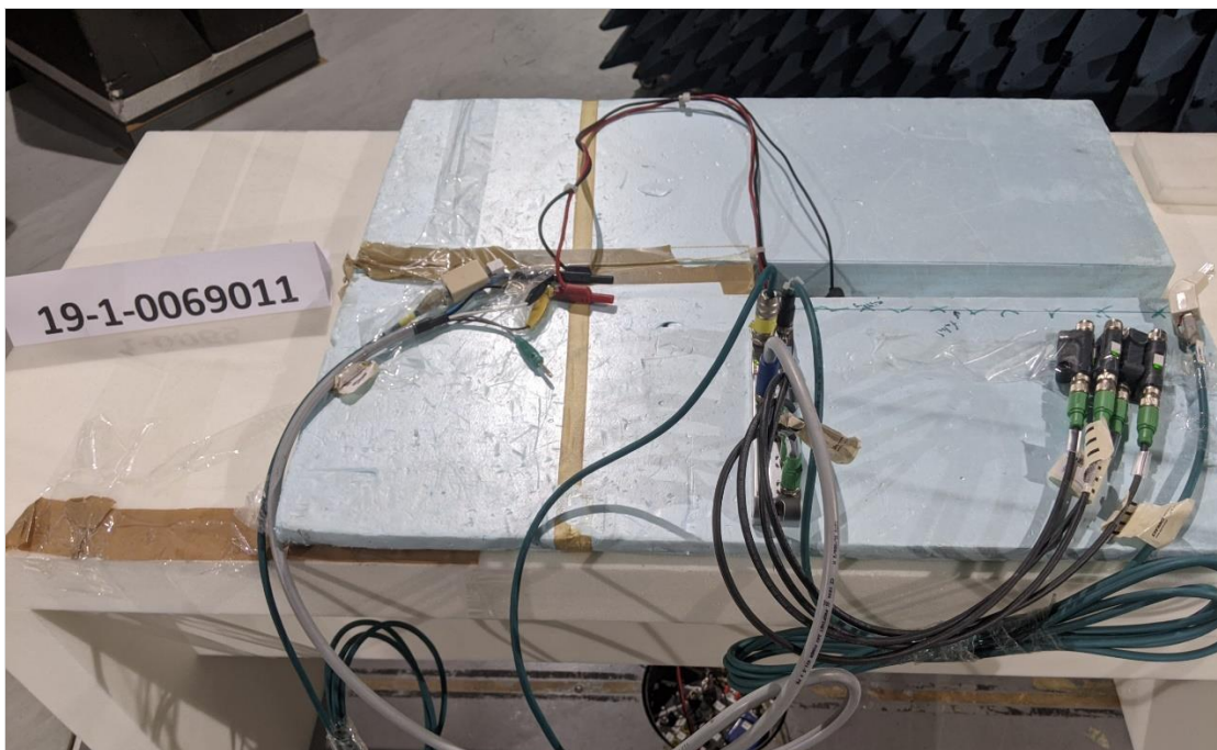
Photograph 2: EUT Test Setup in the semi anechoic chamber, Radiated interference field strength
