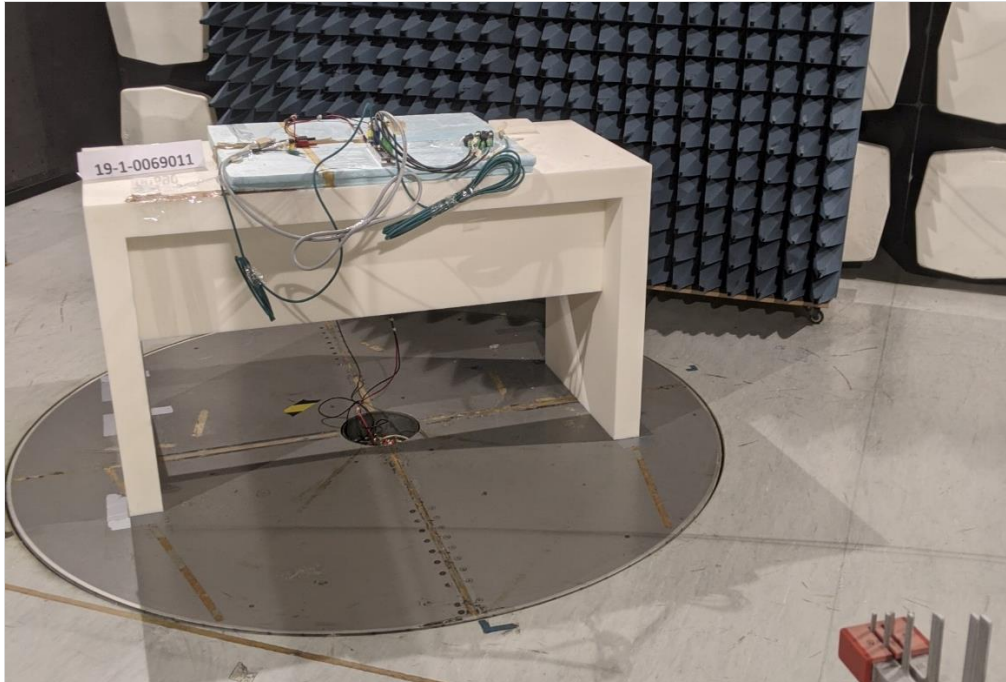
Photograph 1: EUT Test Setup in the semi anechoic chamber, Radiated interference field strength
