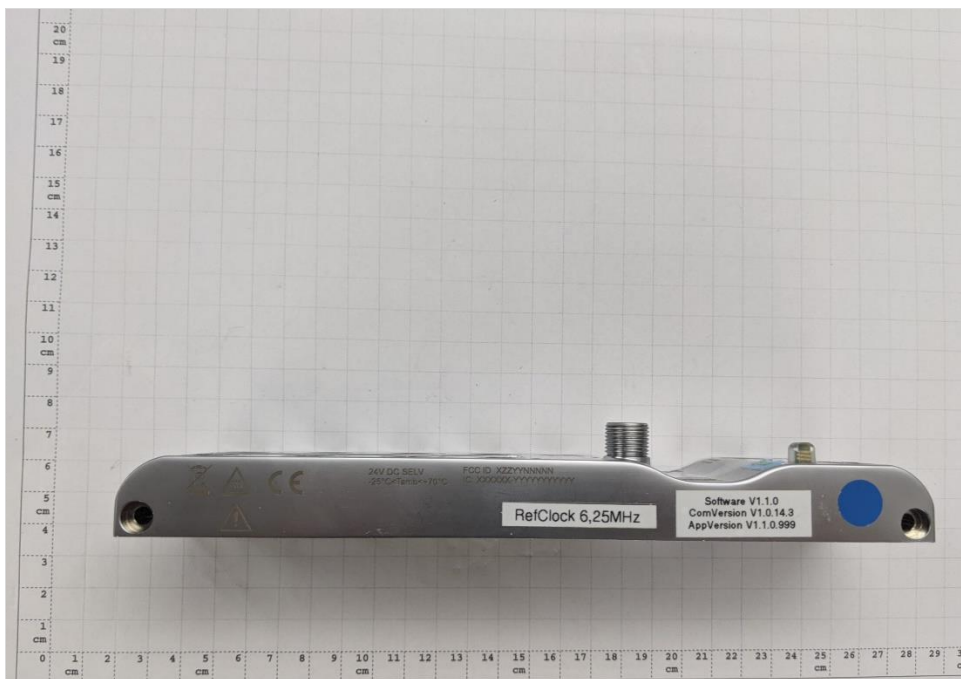
Photograph 4: EUT 1_Right side view
