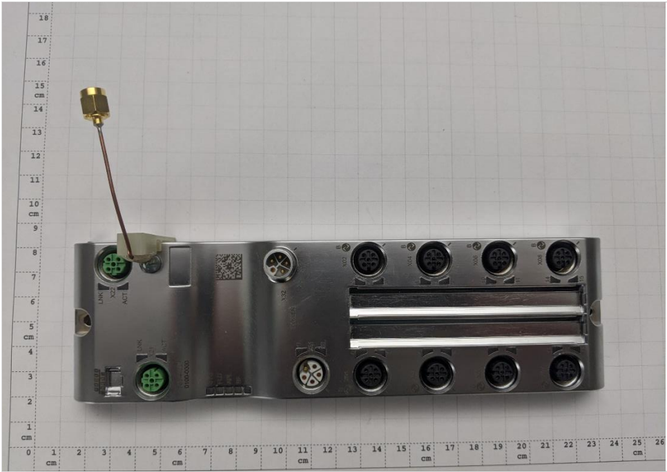
Photograph 7: EUT 2_Top side view
