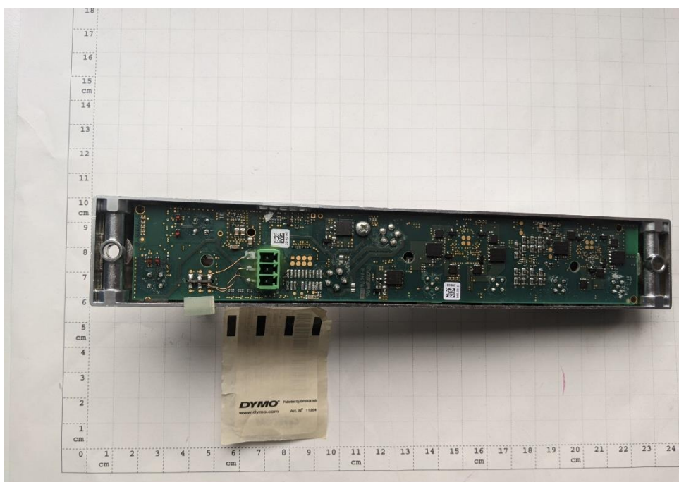
Photograph 8: EUT 2_Bottom side view
