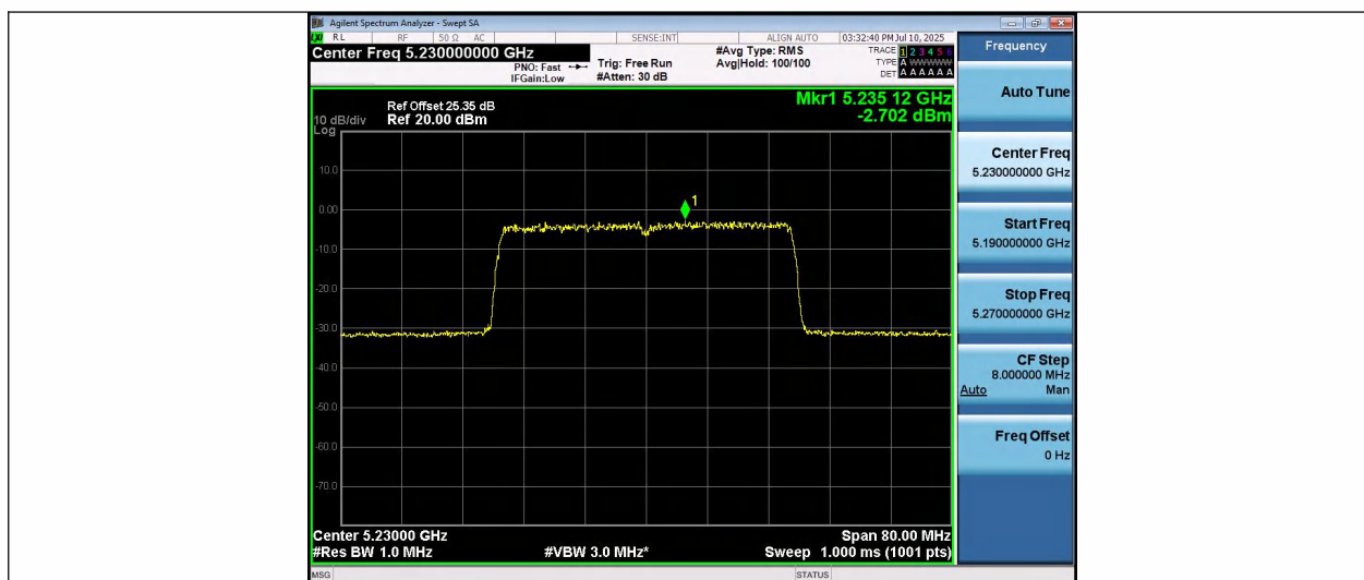
11AX40SISO-Ant1-5230-PASS
