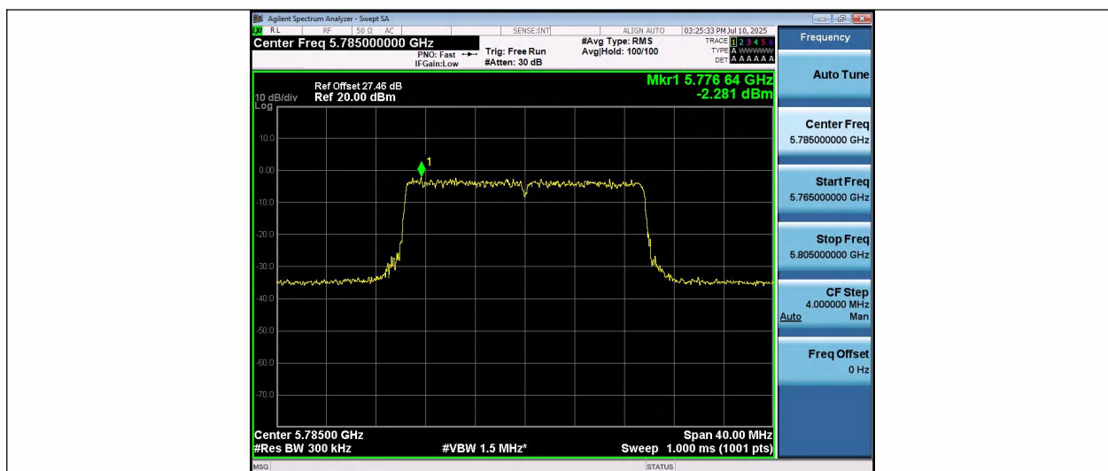
11AX20SISO-Ant1-5785-PASS
