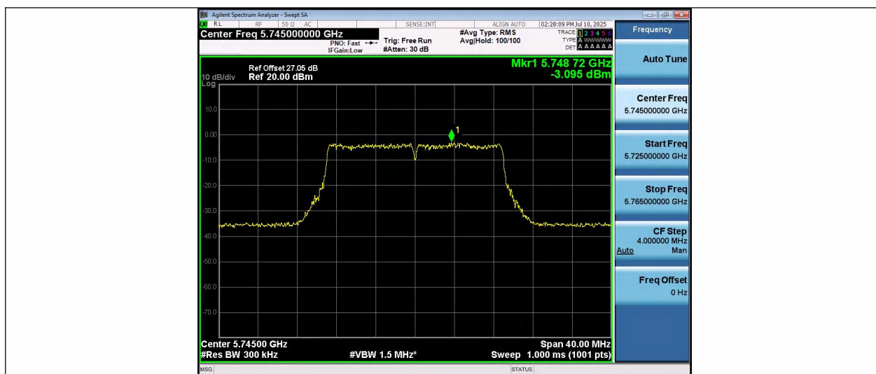
11N20SISO-Ant1-5745-PASS
