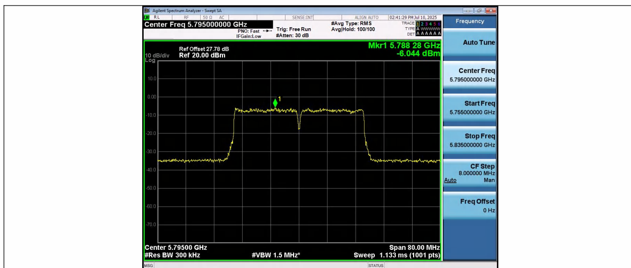
11N40SISO-Ant1-5795-PASS
