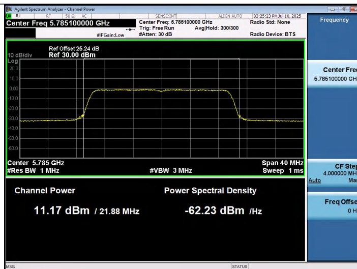
11AX20SISO-Ant1-5785-PASS
