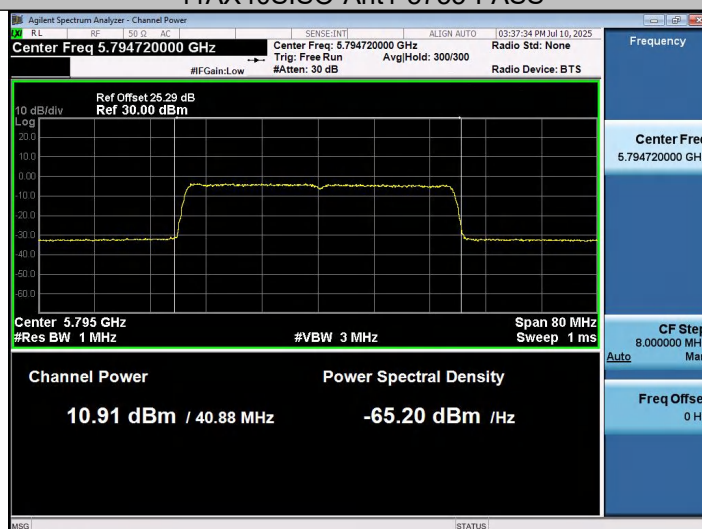
11AX40SISO-Ant1-5795-PASS
