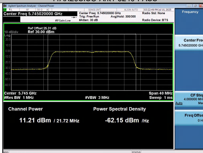
11AX20SISO-Ant1-5745-PASS
