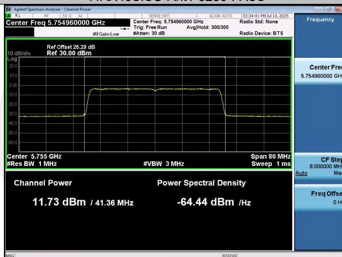
11AX40SISO-Ant1-5755-PASS
