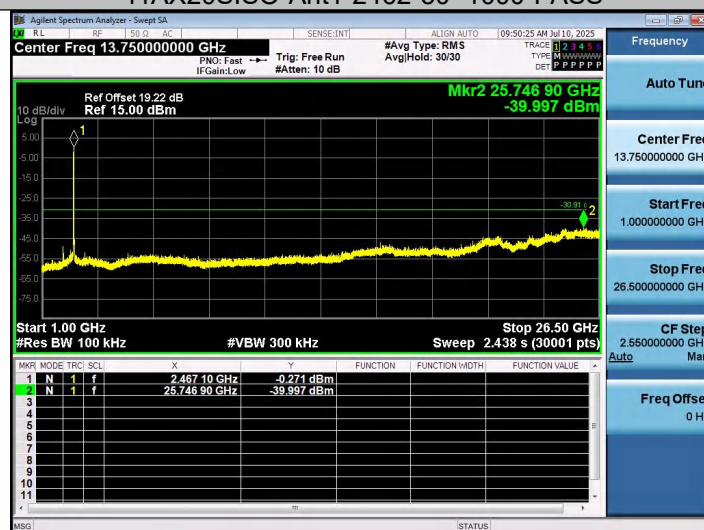
11AX20SISO-Ant1-2462-1000~26500-PASS
