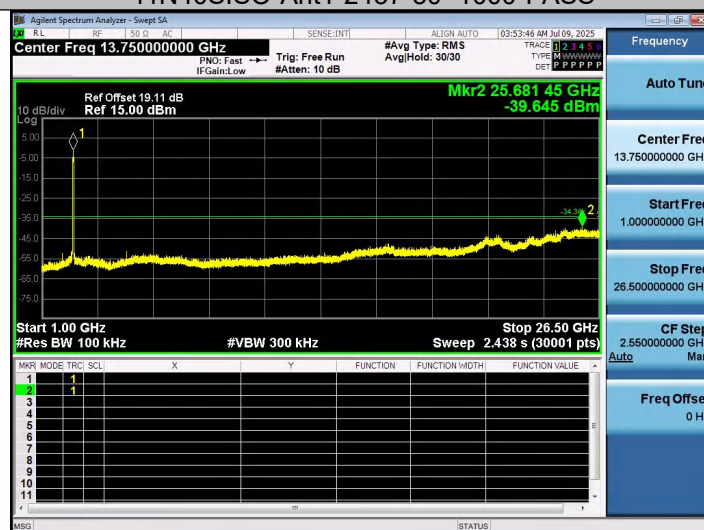
11N40SISO-Ant1-2437-1000~26500-PASS
