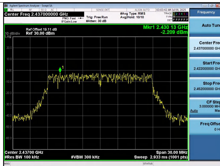
11N20SISO-Ant1-2437-0~Reference-PASS
