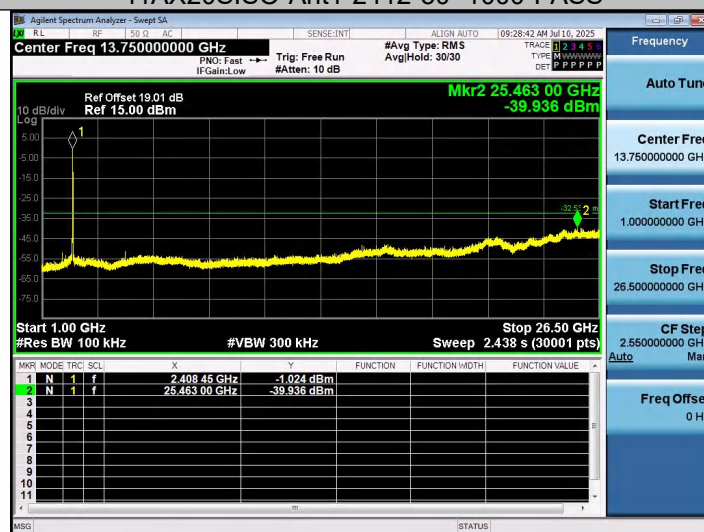
11AX20SISO-Ant1-2412-1000~26500-PASS
