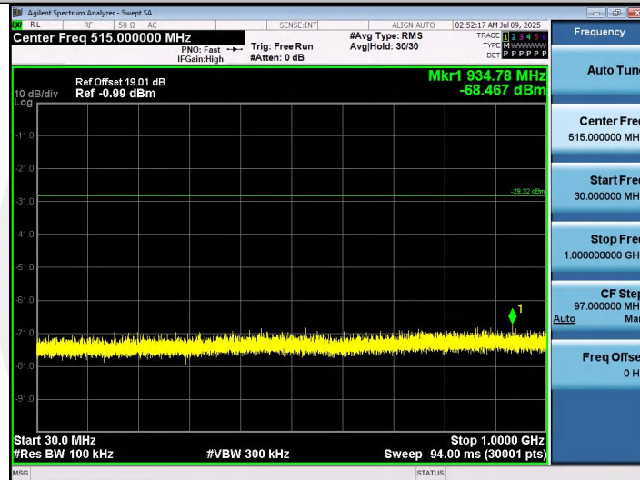
11N20SISO-Ant1-2412-30~1000-PASS
