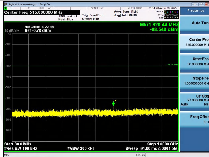
11N20SISO-Ant1-2462-30~1000-PASS
