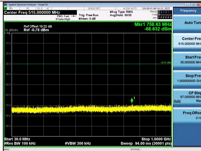
11AX20SISO-Ant1-2462-30~1000-PASS
