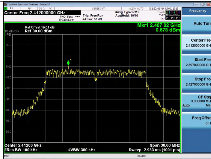
11N20SISO-Ant1-2412-0~Reference-PASS
