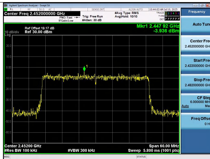
11AX40SISO-Ant1-2452-0~Reference-PASS
