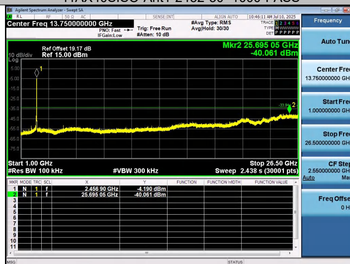
11AX40SISO-Ant1-2452-1000~26500-PASS
