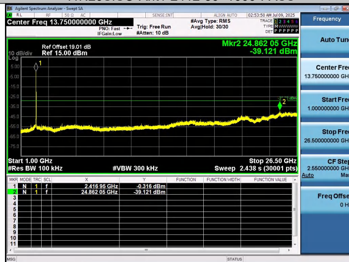
11N20SISO-Ant1-2412-1000~26500-PASS
