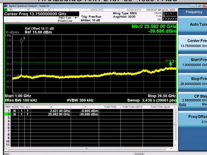
11AX20SISO-Ant1-2437-1000~26500-PASS
