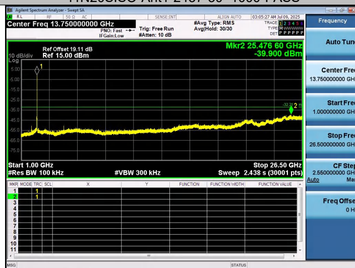
11N20SISO-Ant1-2437-1000~26500-PASS
