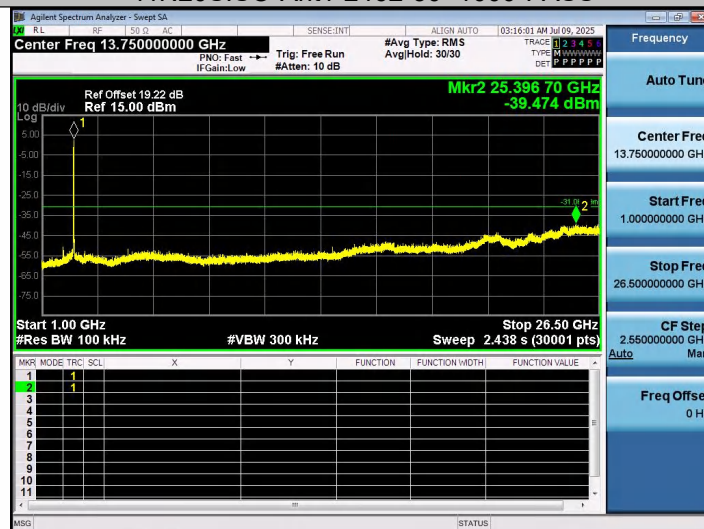
11N20SISO-Ant1-2462-1000~26500-PASS
