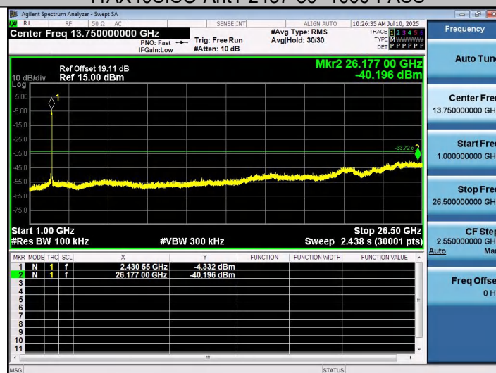
11AX40SISO-Ant1-2437-1000~26500-PASS
