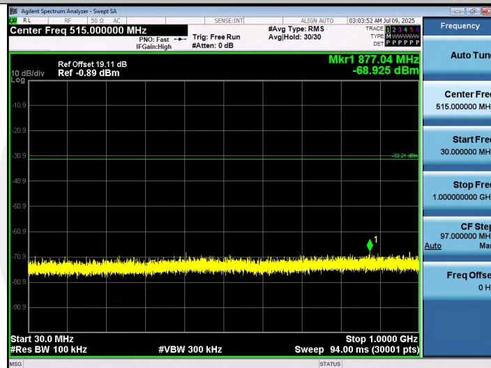
11N20SISO-Ant1-2437-30~1000-PASS
