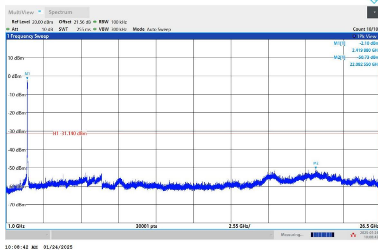
11AX40SISO_Ant1_2452_0~Reference
