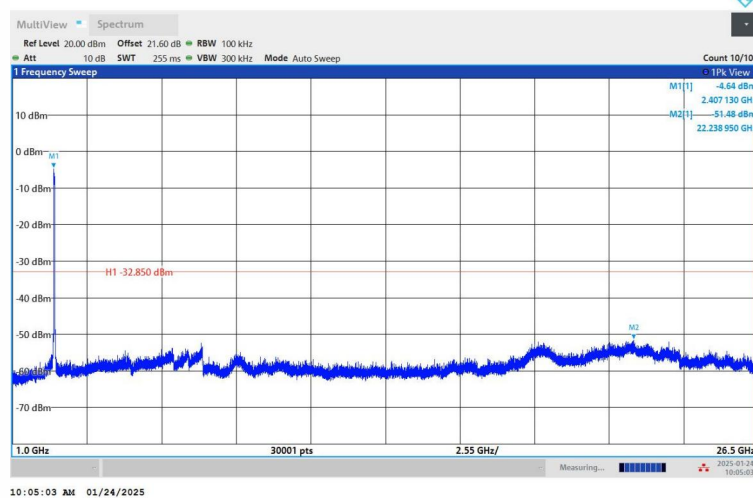
11AX40SISO_Ant1_2437_0~Reference
