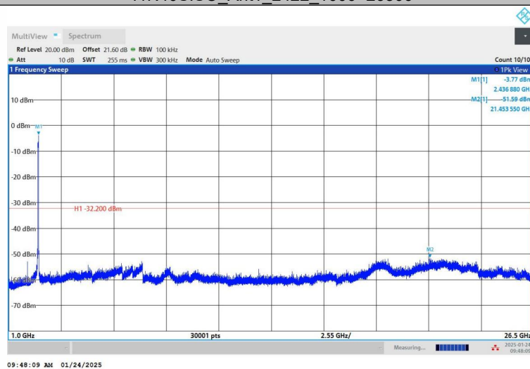
11N40SISO_Ant1_2437_0~Reference
