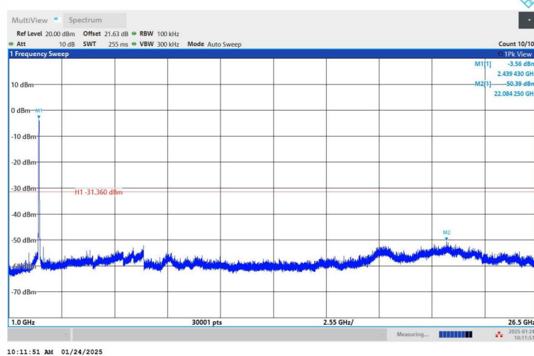
11AX40SISO_Ant1_2452_1000~26500
