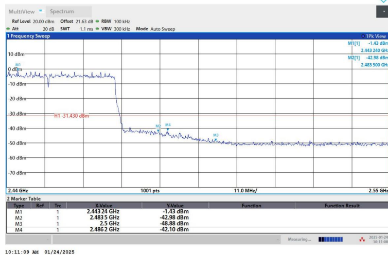
11AX40SISO_Ant1_High_2452
