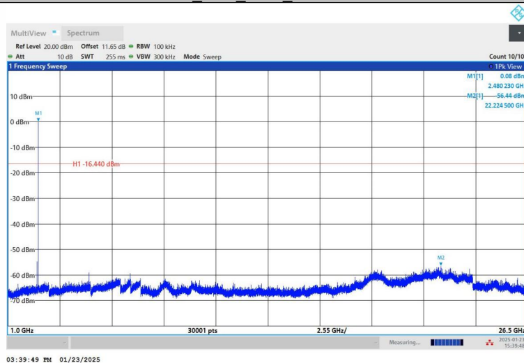
3DH5_Ant1_2480_1000~26500
