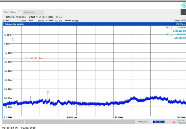
2DH5_Ant1_2441_0~Reference
