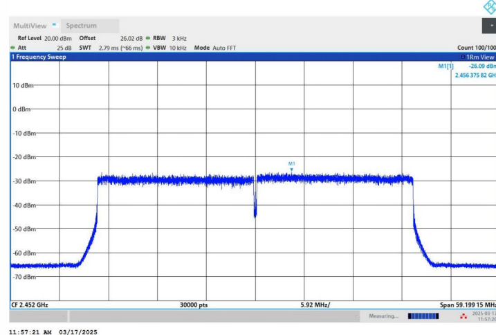
11AX40SISO-Ant1-2452-PASS
