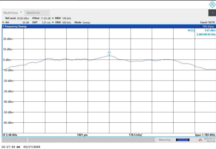
BLE_2M-Ant1-2480-PASS
