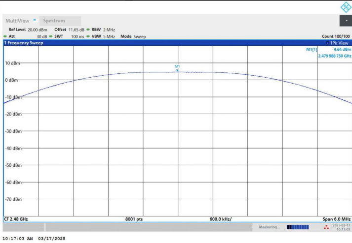
BLE_2M-Ant1-2480-PASS
