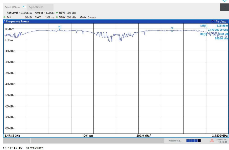
3DH5-Ant1-Hop_2480-PASS
