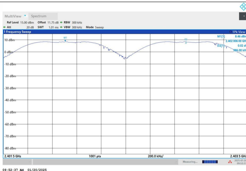
DH5-Ant1-Hop_2402-PASS
