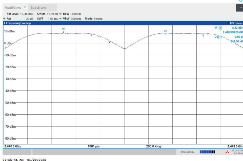
DH5-Ant1-Hop_2441-PASS
