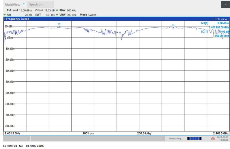
3DH5-Ant1-Hop_2402-PASS
