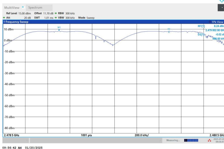
DH5-Ant1-Hop_2480-PASS
