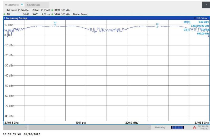
2DH5-Ant1-Hop_2402-PASS
