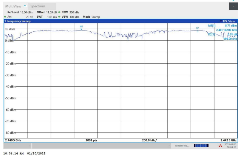
2DH5-Ant1-Hop_2441-PASS
