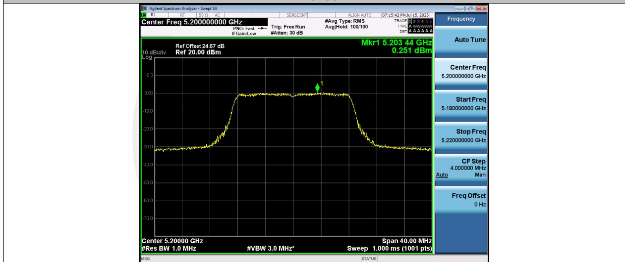
11A-Ant1-5200-PASS
