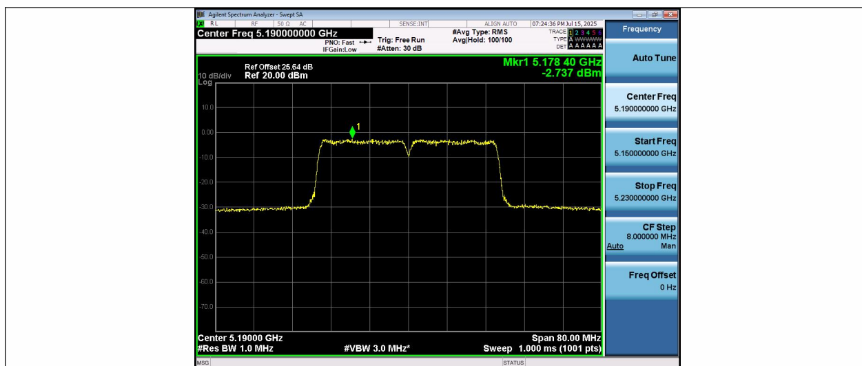
11N40SISO-Ant1-5190-PASS
