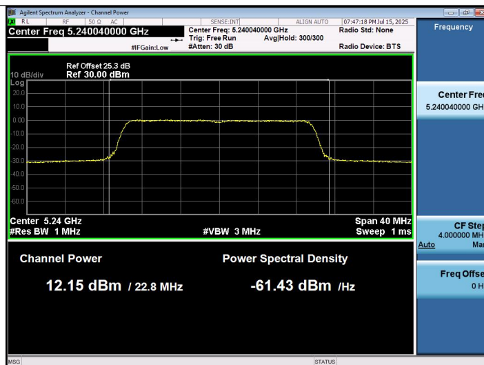
11AX20SISO-Ant1-5240-PASS
