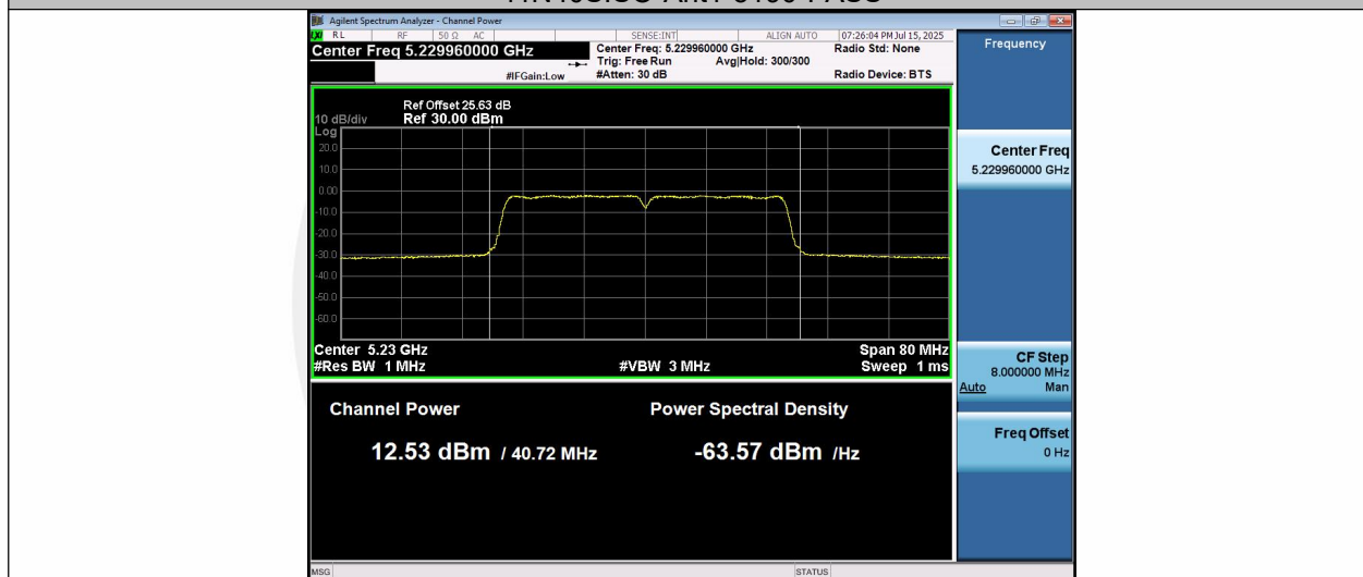
11N40SISO-Ant1-5230-PASS
