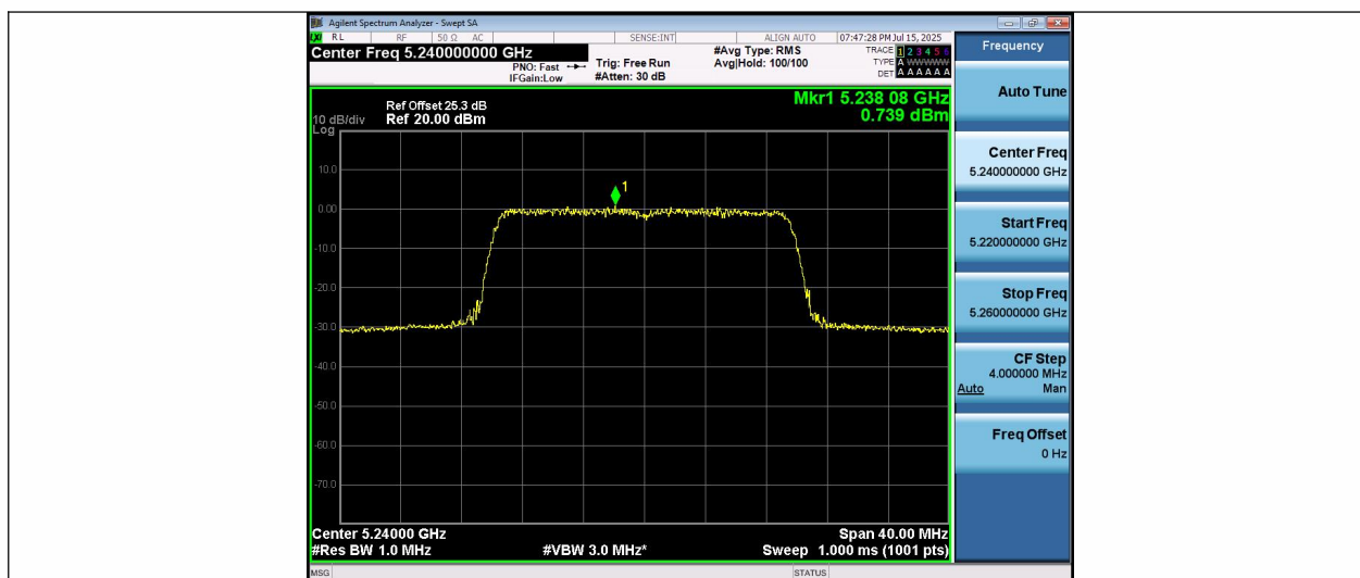
11AX20SISO-Ant1-5240-PASS
