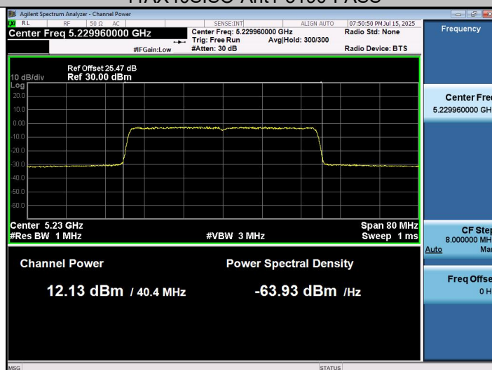
11AX40SISO-Ant1-5230-PASS
