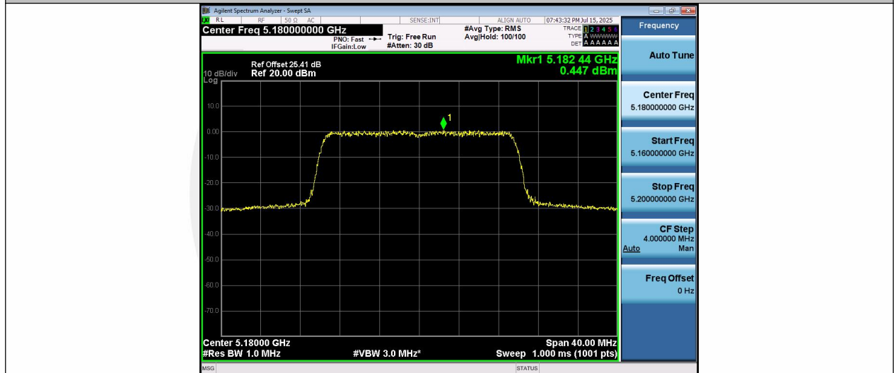
11AX20SISO-Ant1-5180-PASS
