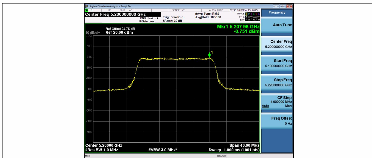
11AC20SISO-Ant1-5200-PASS
