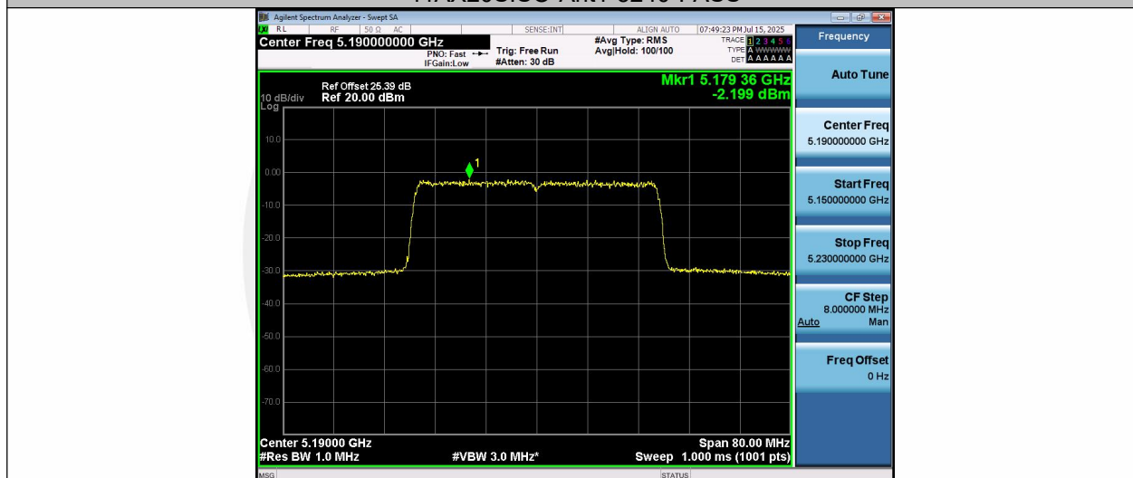
11AX40SISO-Ant1-5190-PASS
