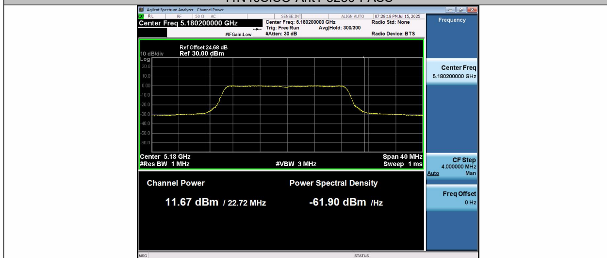
11AC20SISO-Ant1-5180-PASS
