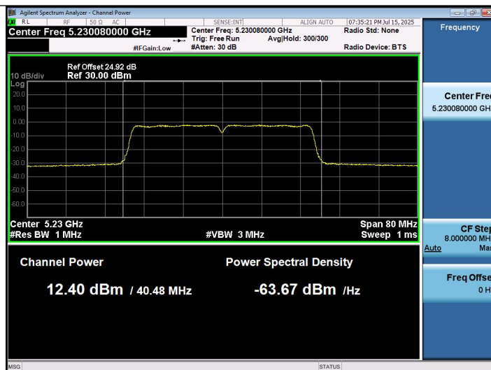
11AC40SISO-Ant1-5230-PASS
