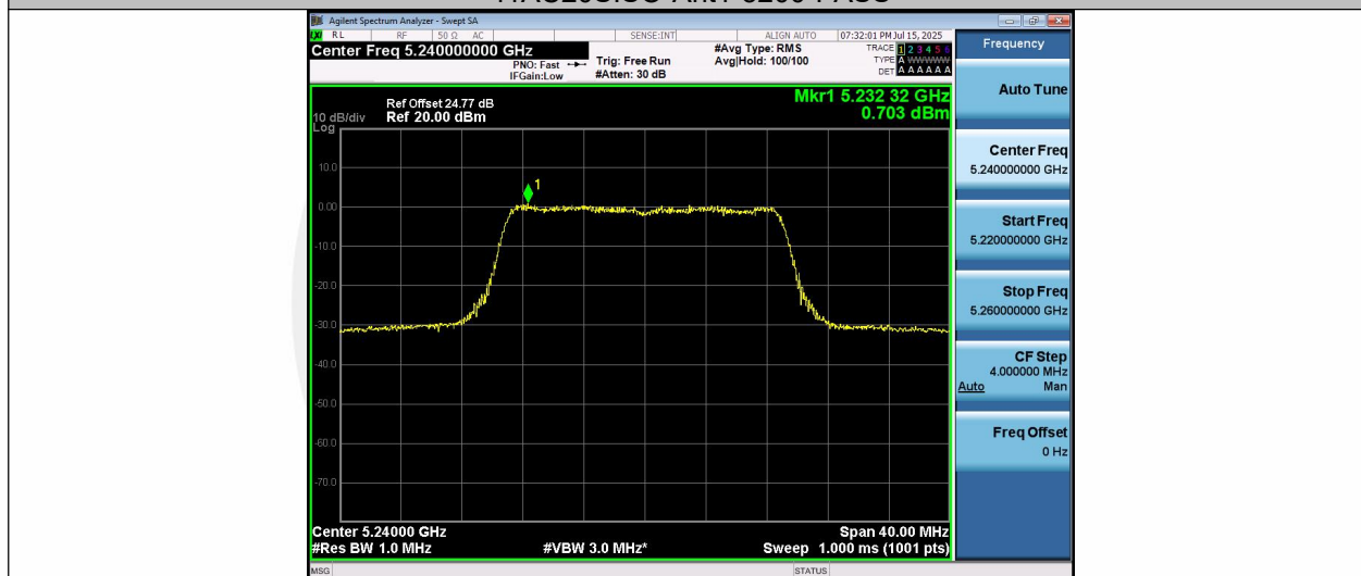
11AC20SISO-Ant1-5240-PASS
