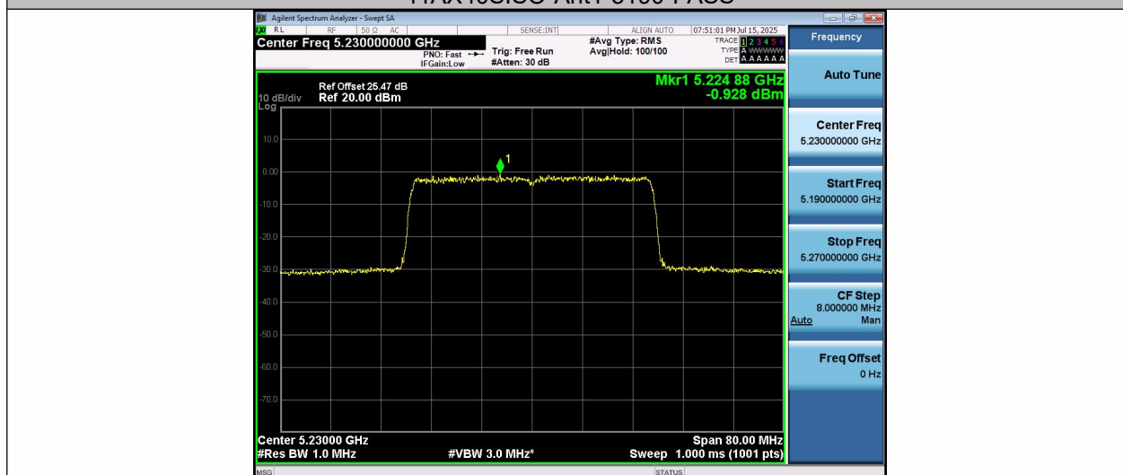
11AX40SISO-Ant1-5230-PASS
