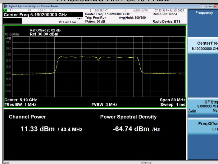
11AC40SISO-Ant1-5190-PASS
