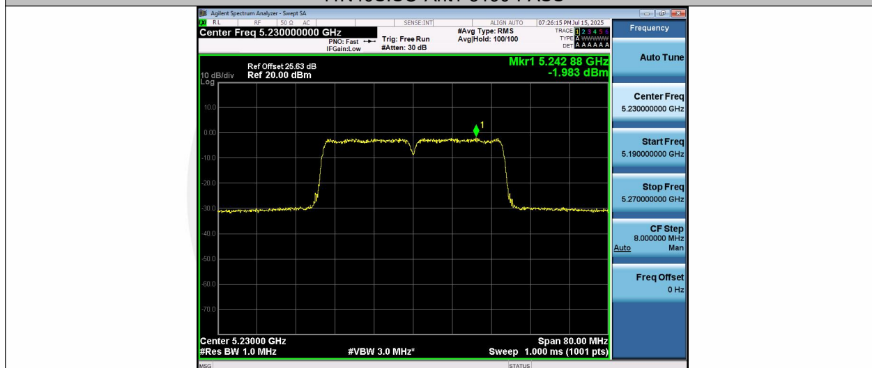
11N40SISO-Ant1-5230-PASS
