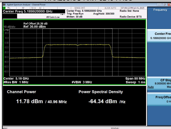
11AX40SISO-Ant1-5190-PASS
