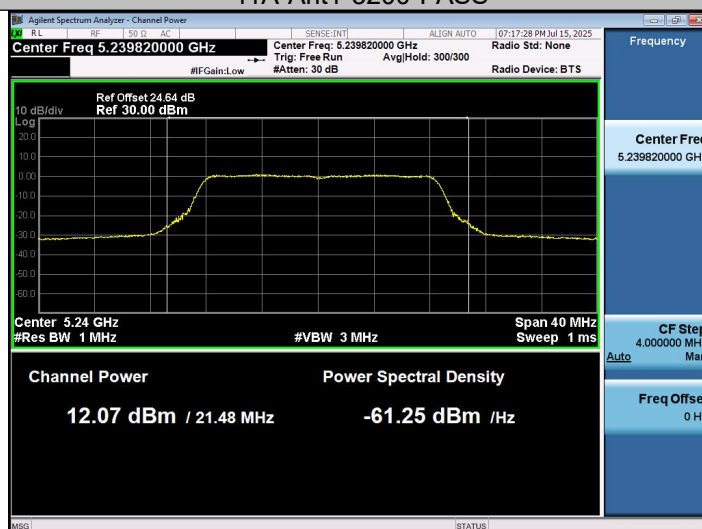
11A-Ant1-5240-PASS
