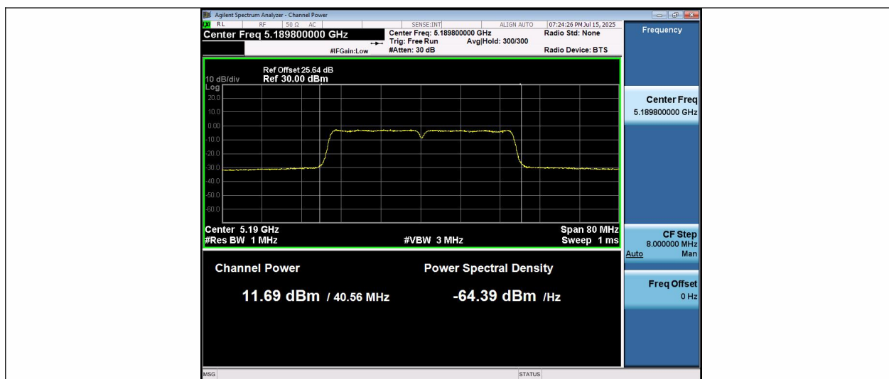
11N40SISO-Ant1-5190-PASS
