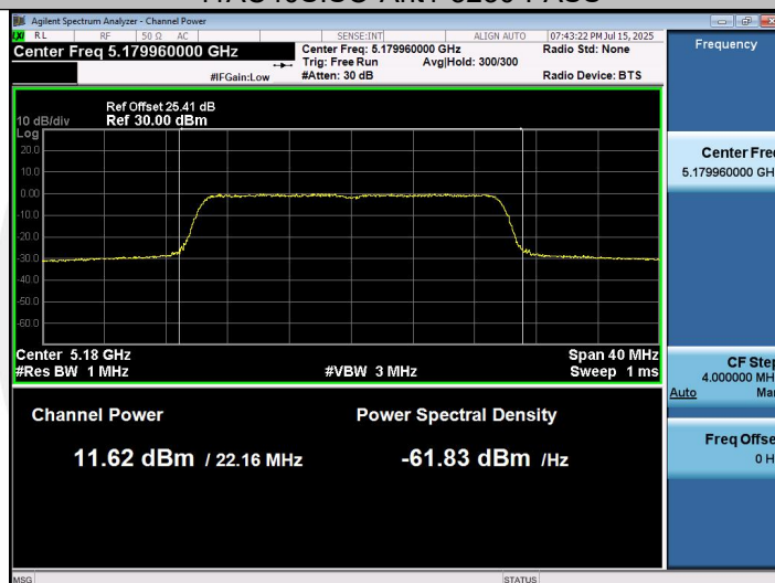
11AX20SISO-Ant1-5180-PASS
