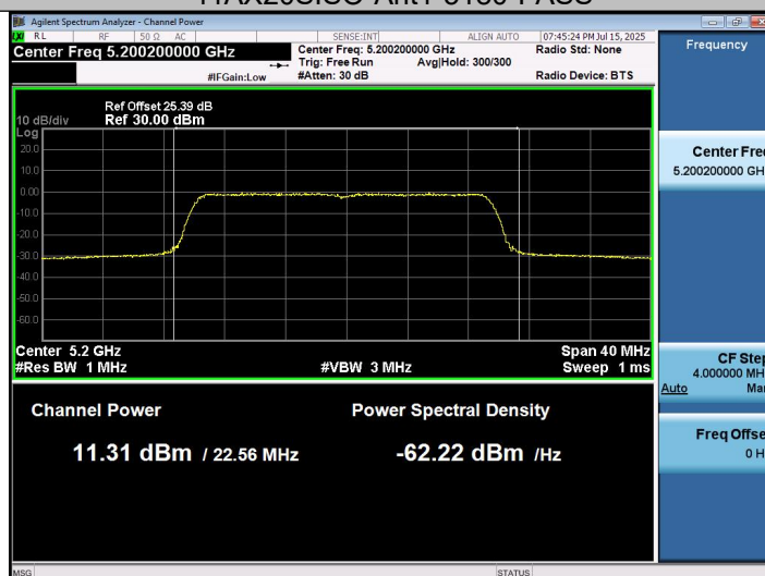
11AX20SISO-Ant1-5200-PASS
