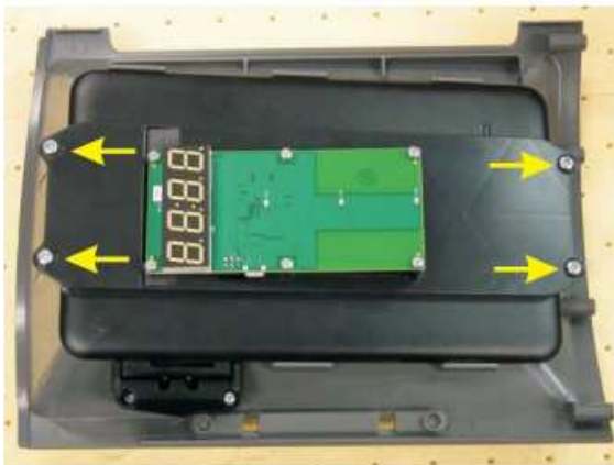
Place the Tablet Mount over the Tablet and secure with the screws.
