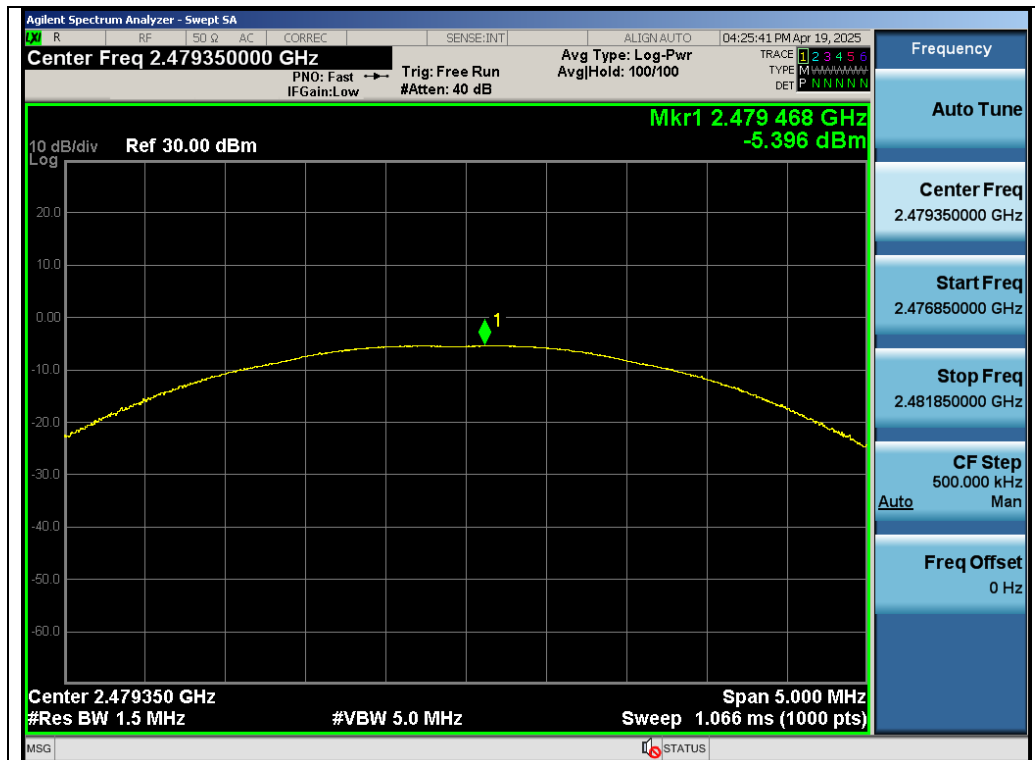
Test_Graph_SRD 2.4G_ANT0_2479.35_Peak Power
