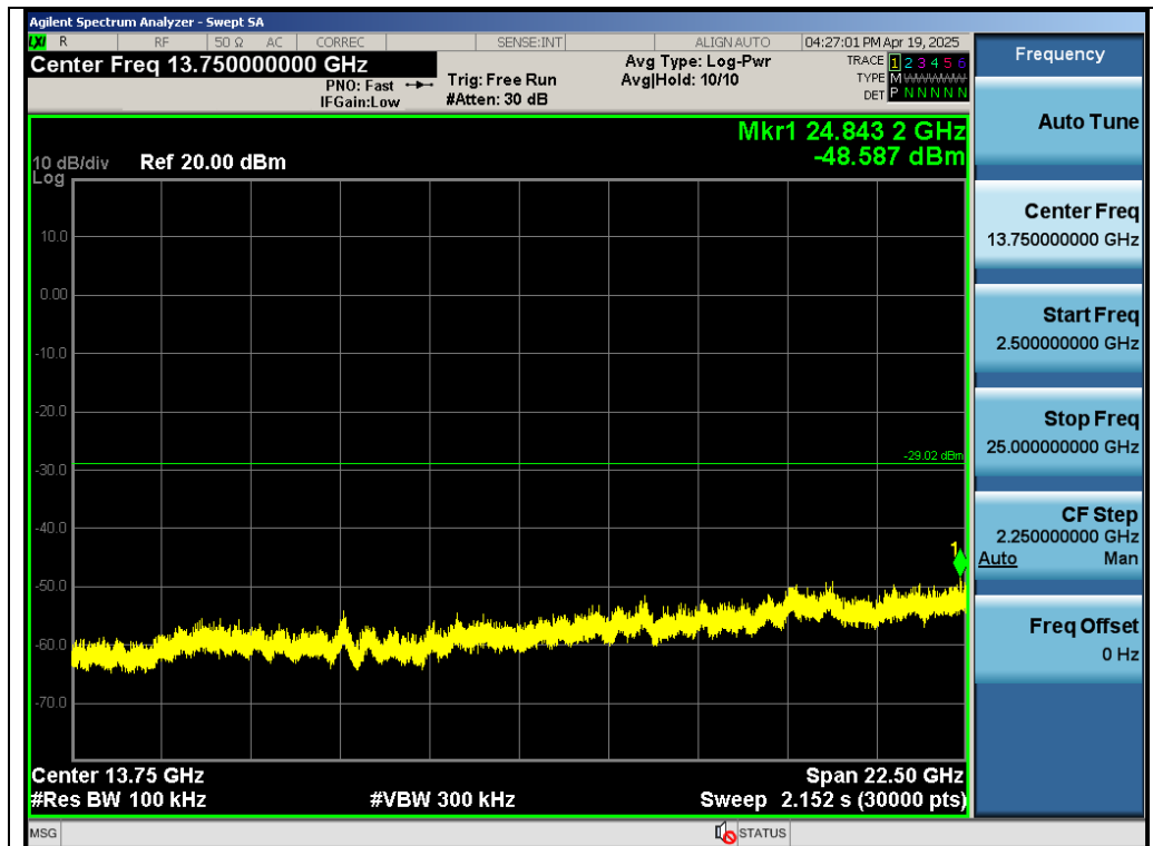
Test_Graph_SRD 2.4G_ANT0_2479.35_Higher Band Emissions
