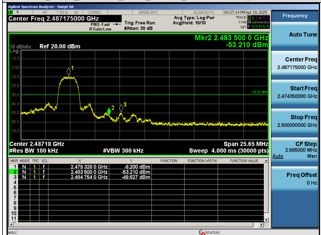
Test_Graph_SRD 2.4G_ANT0_2479.35_Higher Band Edge Emissions
