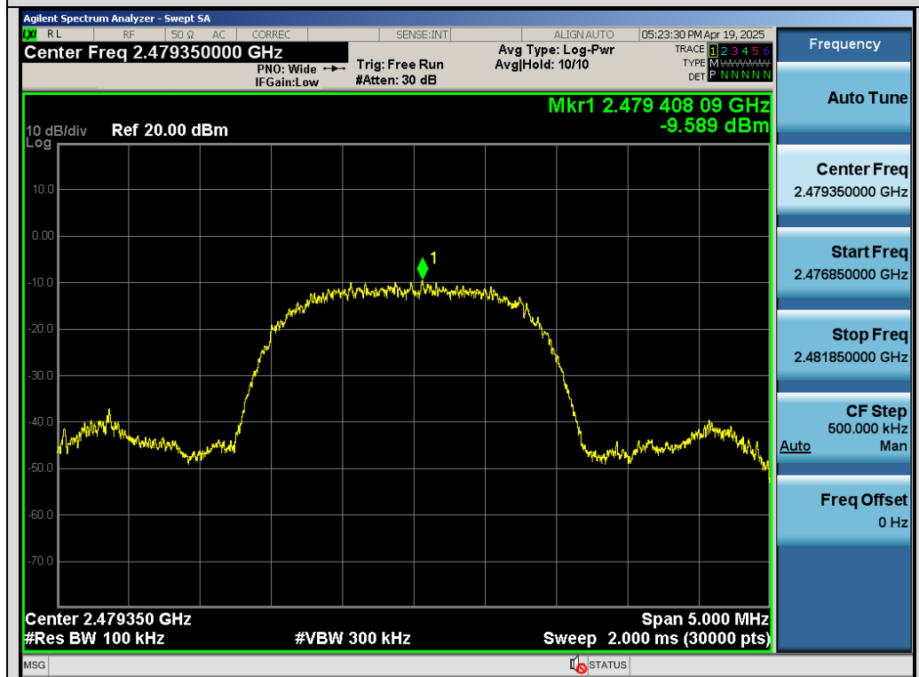
Test_Graph_SRD 2.4G_ANT1_2479.35_Reference Level
