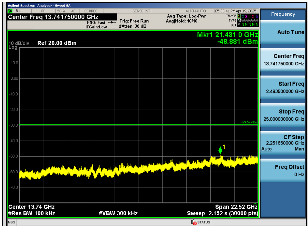
Test_Graph_SRD 2.4G_ANT1_2443.35_Higher Band Emissions
