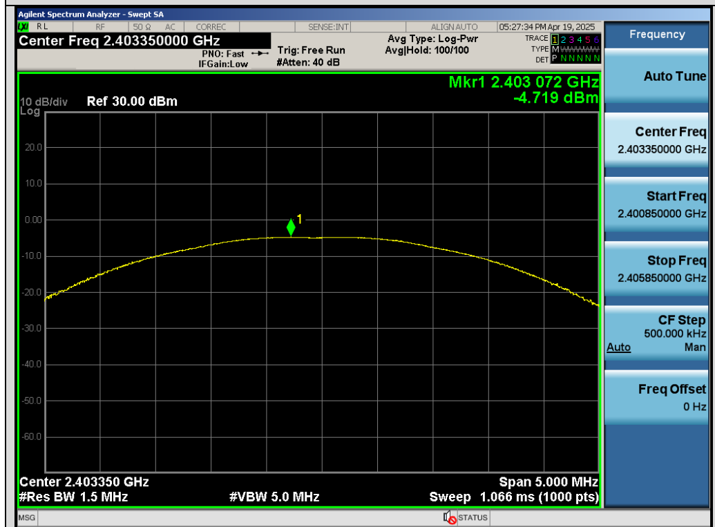
Test_Graph_SRD 2.4G_ANT1_2403.35_Peak Power
