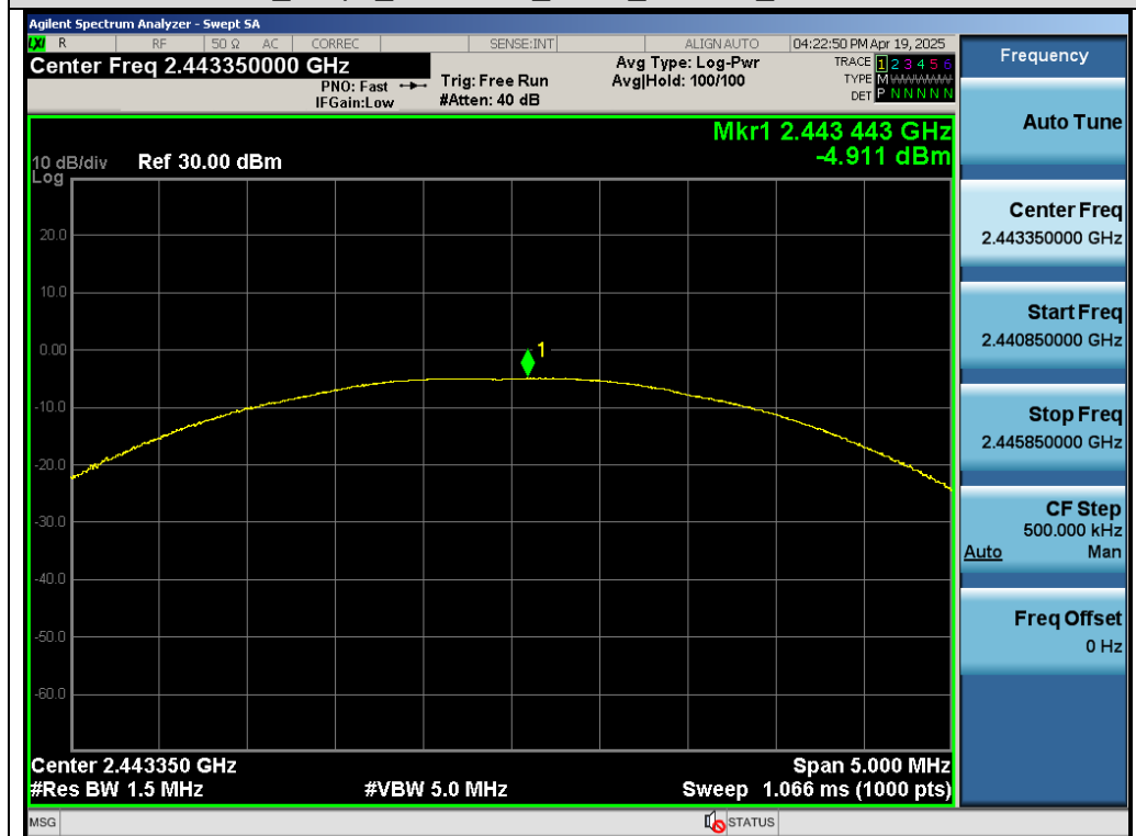
Test_Graph_SRD 2.4G_ANT0_2443.35_Peak Power
