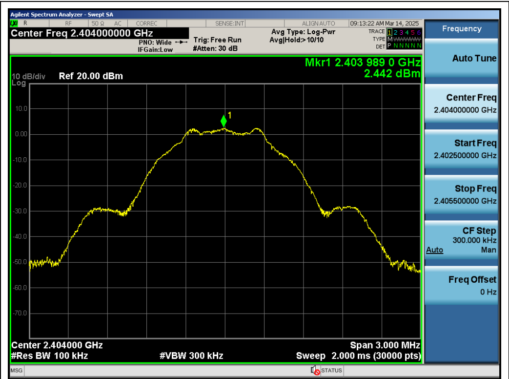
Test_Graph_SRD_ANT1_2404_GFSK_Reference Level
