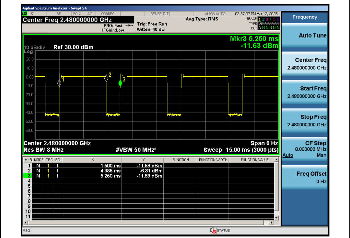
EDR-π /4-DQPSK-ANT1-2480
