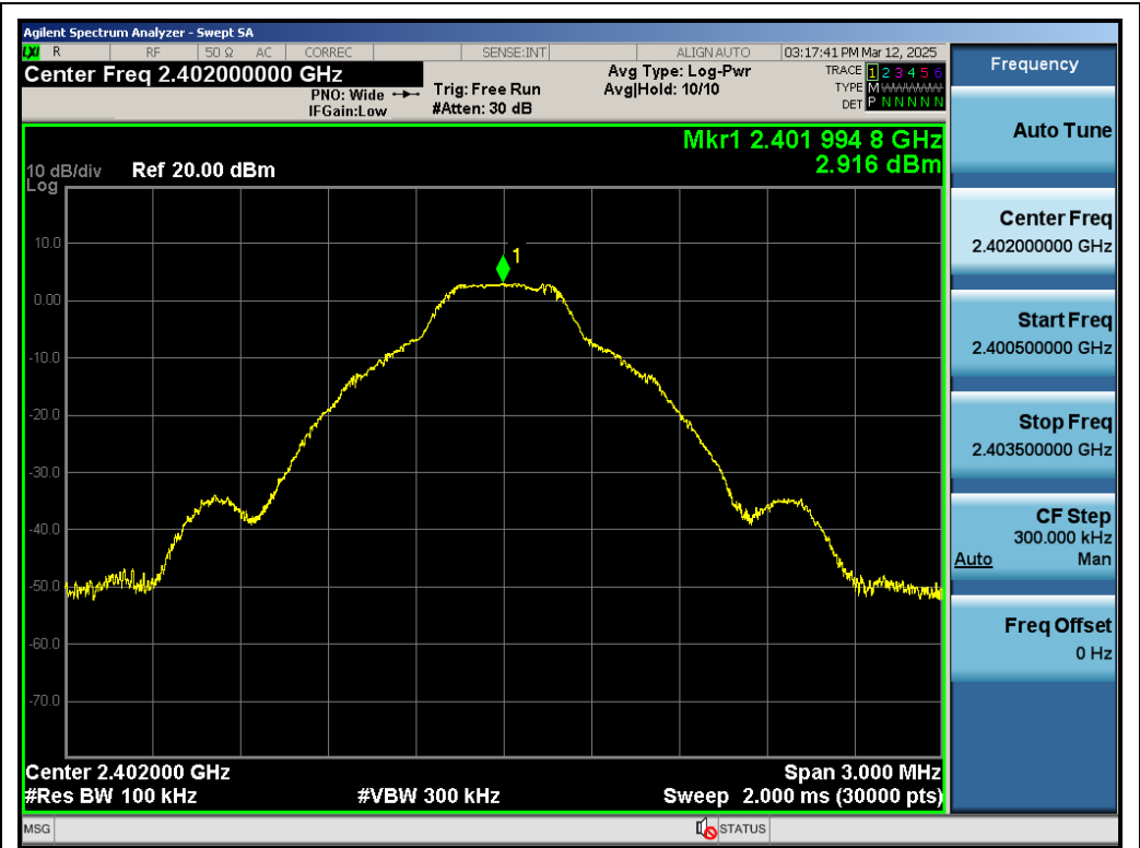
Test_Graph_BR_ANT1_2402_1Mbps_Reference Level
