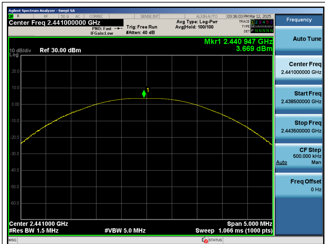
Test_Graph_EDR_ANT1_2441_2Mbps_Peak Power
