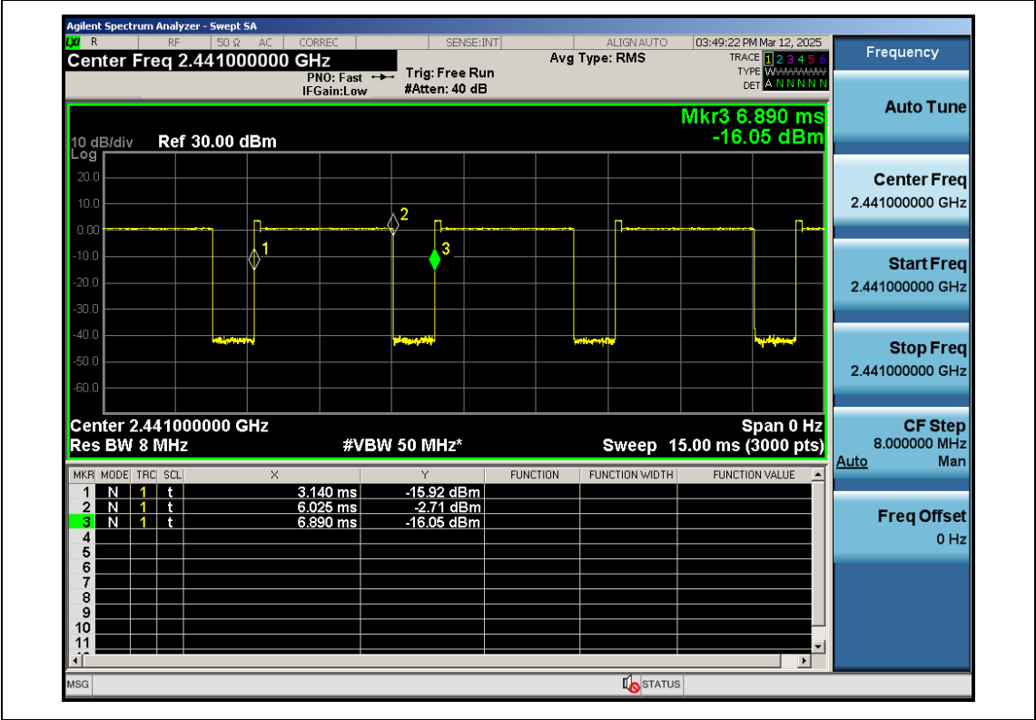
EDR-8DPSK-ANT1-2441
