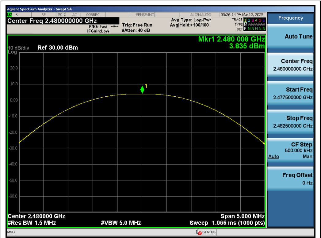
Test_Graph_BR_ANT1_2480_1Mbps_Peak Power
