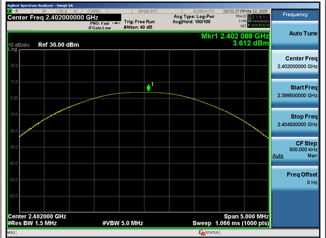
Test_Graph_EDR_ANT1_2402_2Mbps_Peak Power
