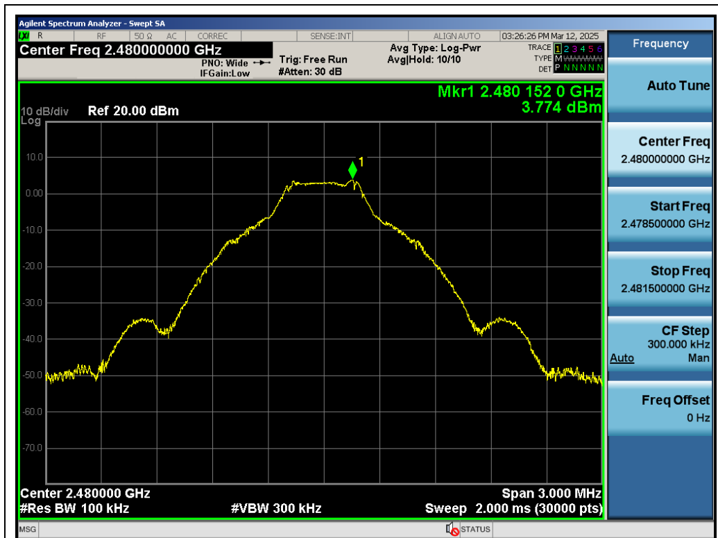
Test_Graph_BR_ANT1_2480_1Mbps_Reference Level
