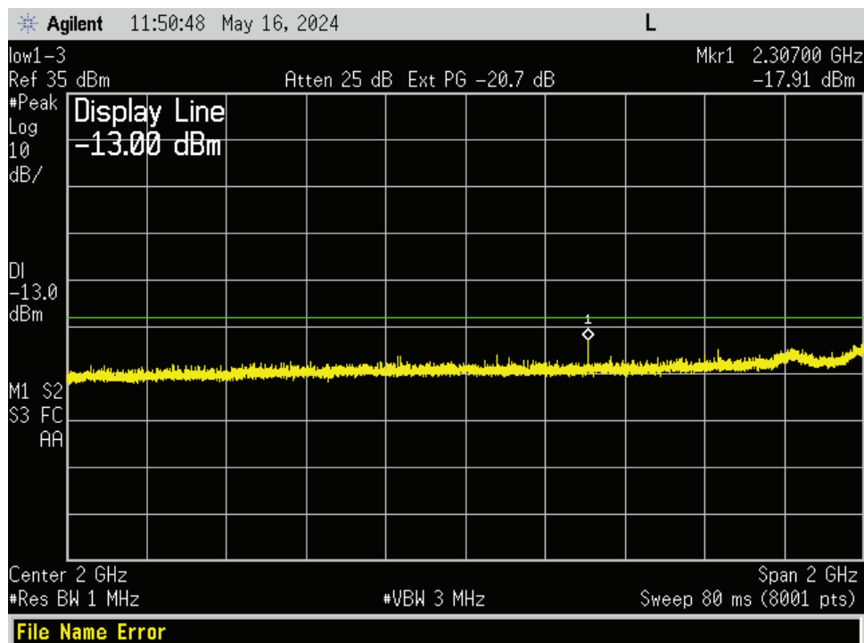
Figure 324. 769 MHz, 1 - 3 GHz
