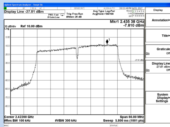
802.11n(HT40)- Low channel Reference
