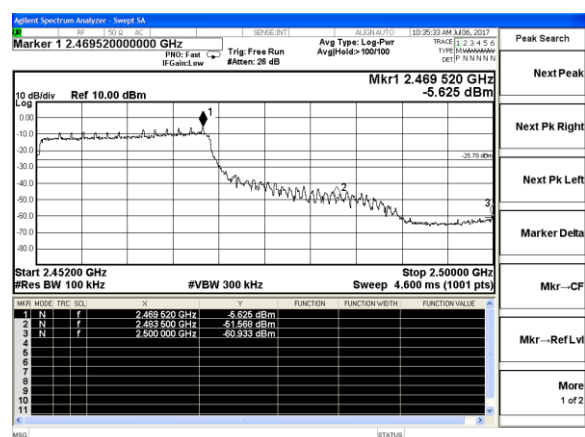
802.11n(HT40)-High channel
