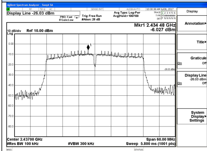
802.11n-HT40 Middle channel Reference
