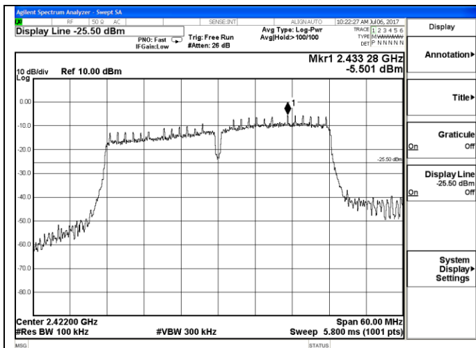
802.11n-HT40 Low channel Reference
