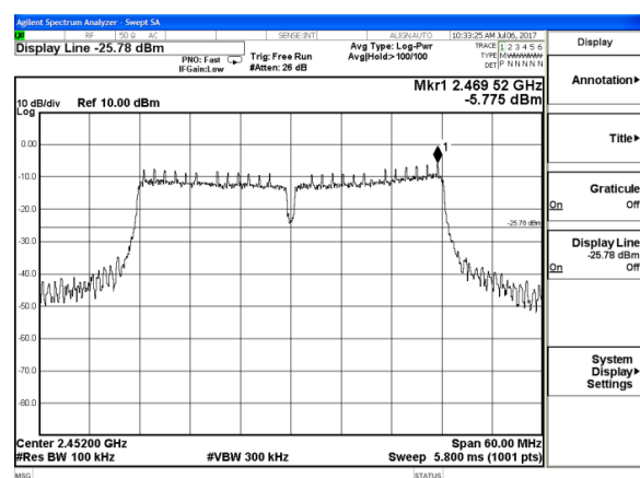
802.11n(HT40)-High channel Reference
