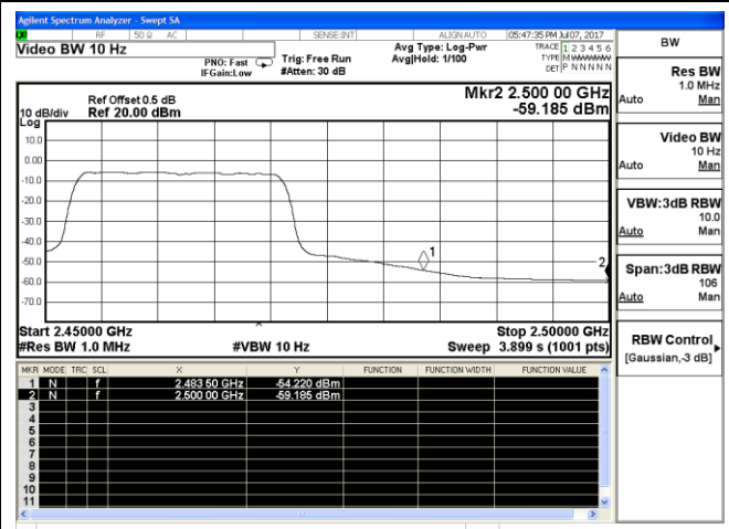
Channel 11 / 2462 MHz – Average
