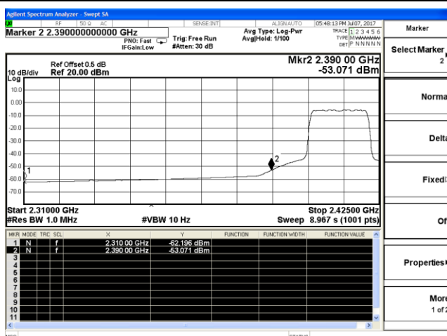
Channel 1 / 2412 MHz – Average
