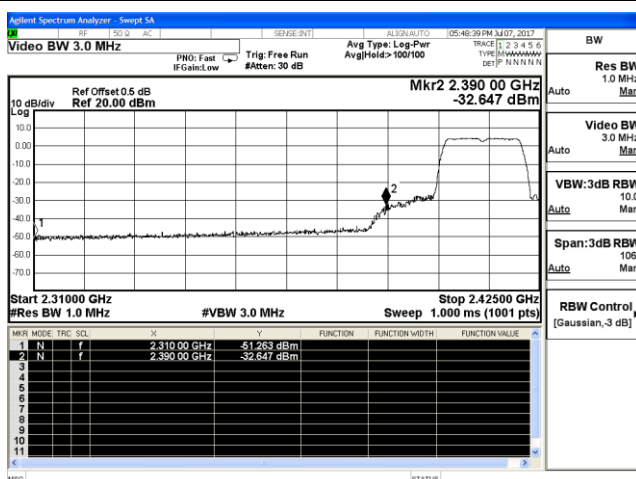
Channel 1 / 2412 MHz – Peak
