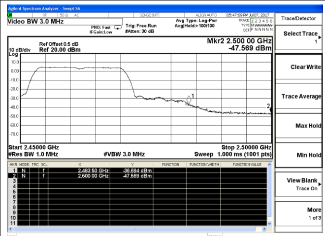
Channel 11 / 2462 MHz – Peak
