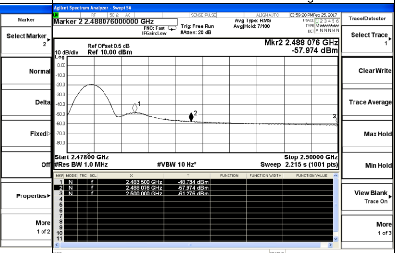
Channel 78 / 2480 MHz –Average
