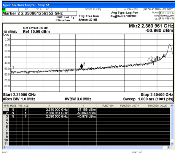
Channel 0 / 2402 MHz –Peak
