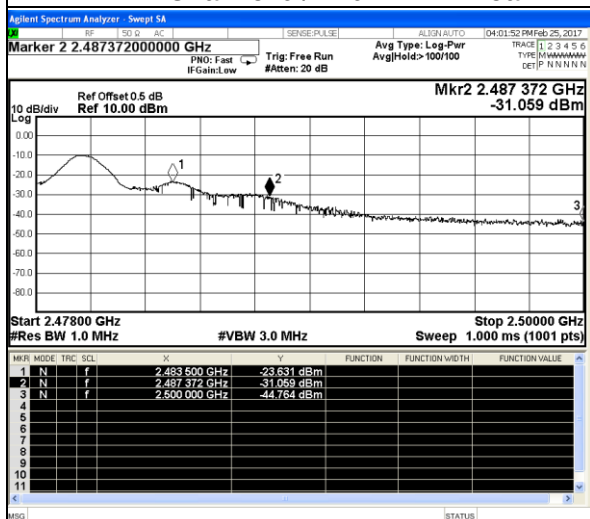
Channel 78 / 2480 MHz –Peak
