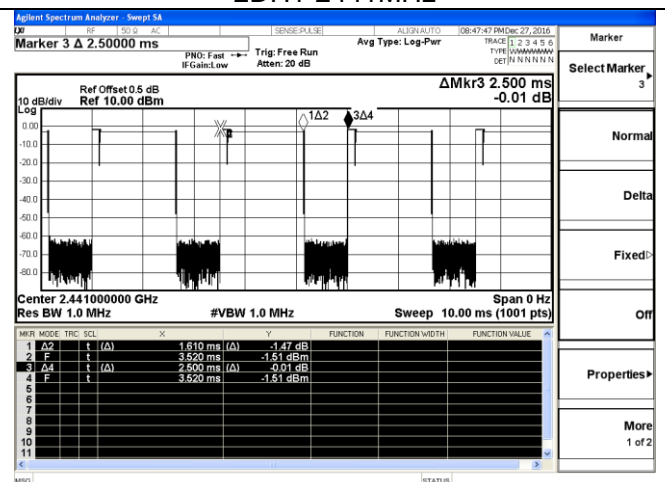
2DH3-2441MHz
