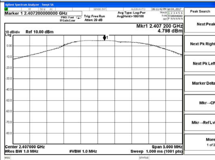
Channel 0 / 2407 MHz
