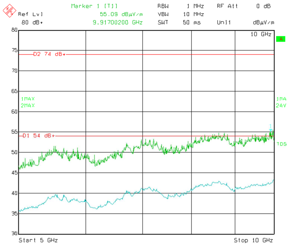
Figure 8.4-17: Radiated spurious emissions, low channel, antenna in horizontal polarization, frequency range 5 to 10 GHz
