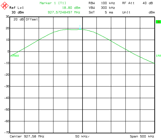
Figure 8.3-3: Output power on high channel
