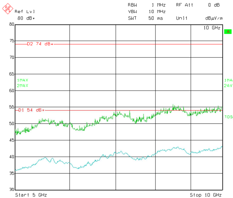
Figure 8.4-18: Radiated spurious emissions, low channel, antenna in vertical polarization, frequency range 5 to 10 GHz
