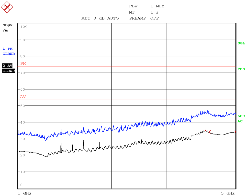
Figure 8.4-13: Radiated spurious emissions, mid channel, antenna in horizontal polarization, frequency range 1 to 5 GHz
