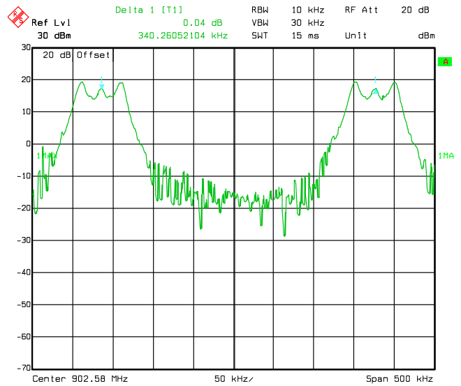
Figure 8.2-4: Carrier frequency separation
