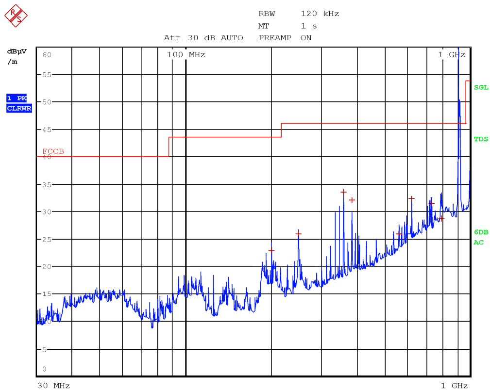
Figure 8.4-7: Radiated spurious emissions, mid channel, antenna in horizontal polarization, frequency range 30 to 1000 MHz
