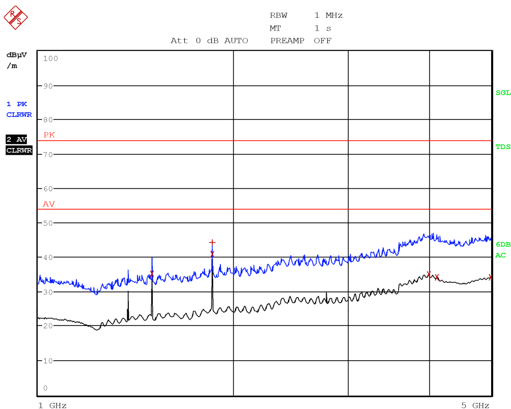
Figure 8.4-16: Radiated spurious emissions, high channel, antenna in vertical polarization, frequency range 1 to 5 GHz
