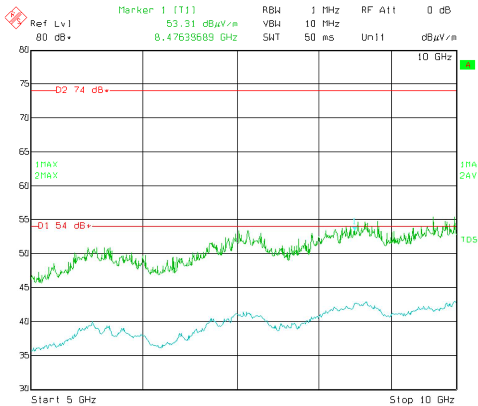
Figure 8.4-20: Radiated spurious emissions, mid channel, antenna in vertical polarization, frequency range 5 to 10 GHz
