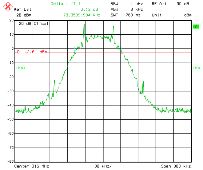
Figure 8.2-2: 20 dB bandwidth on mid channel
