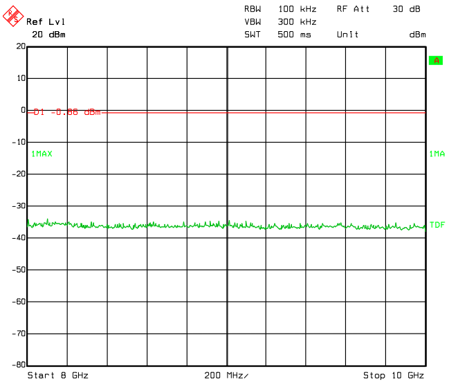
Figure 8.4-2: Conducted spurious emissions, low channel
