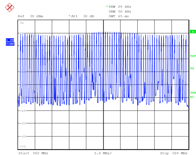
Figure 8.2-5: Number of hopping channels
