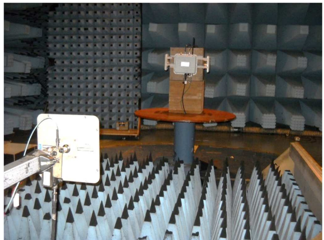
Figure 9.1-4: Radiated emissions above 1 GHz
