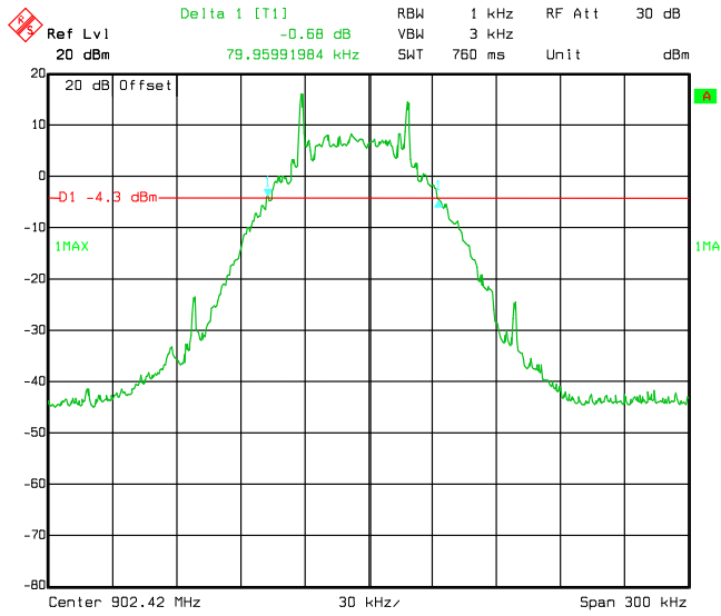
Figure 8.2-1: 20 dB bandwidth on low channel
