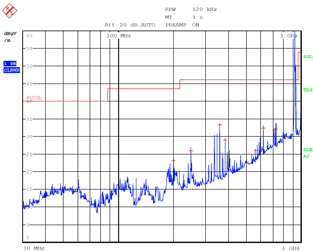
Figure 8.4-7: Radiated spurious emissions, high channel, antenna in horizontal polarization, frequency range 30 to 1000 MHz
