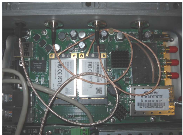
Figure 9.2-1: EUT photos
