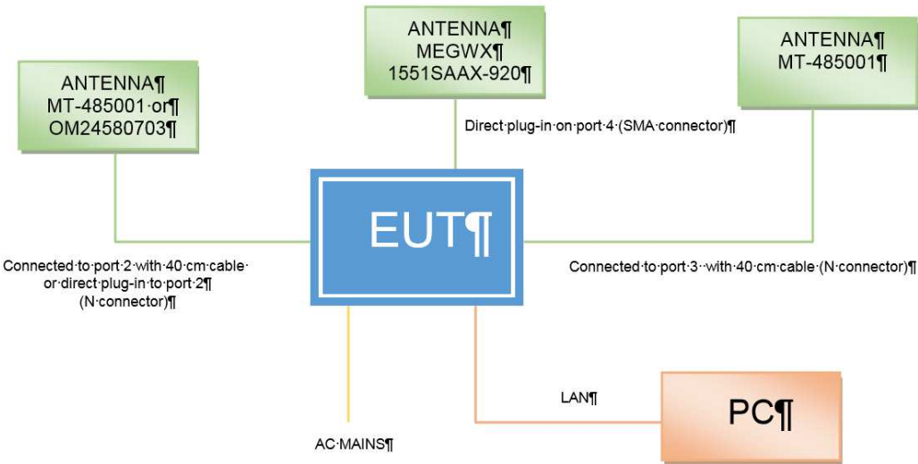
Figure 3.6-1: Setup diagram
