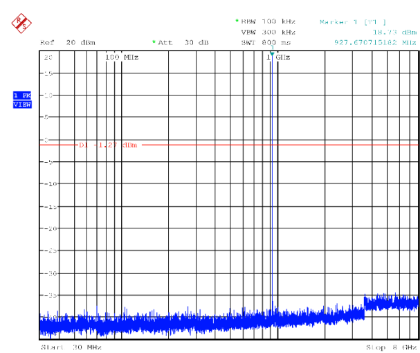
Figure 8.4-5: Conducted spurious emissions, high channel
