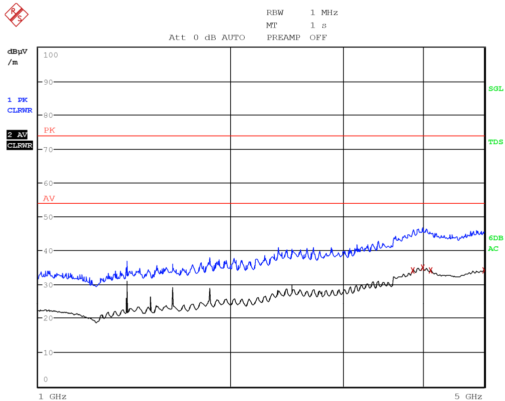
Figure 8.4-15: Radiated spurious emissions, high channel, antenna in horizontal polarization, frequency range 1 to 5 GHz
