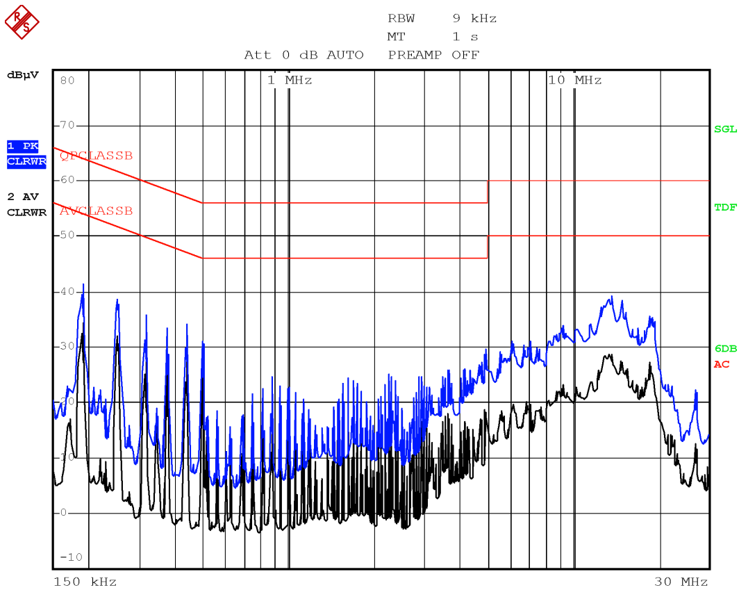
Plot 8.1-2: Conducted emissions on neutral line
