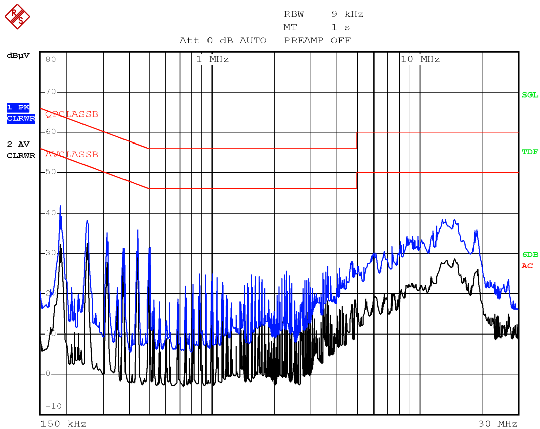
Plot 8.1-1: Conducted emissions on phase line
