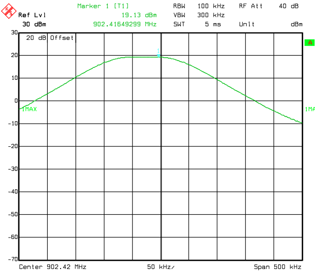
Figure 8.3-1: Output power on low channel
