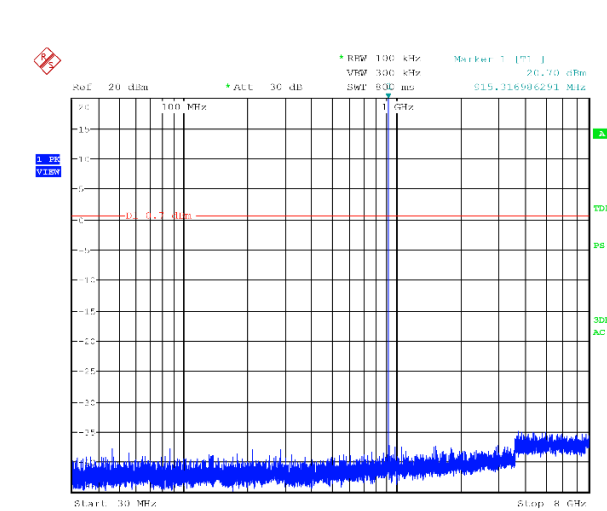
Figure 8.4-3: Conducted spurious emissions, mid channel
