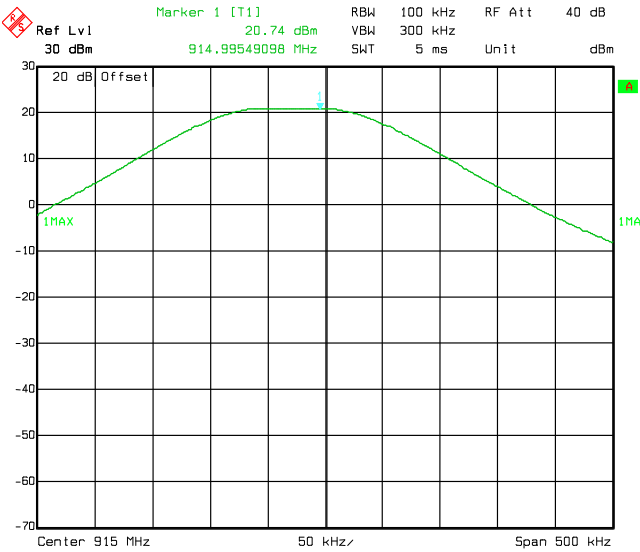
Figure 8.3-2: Output power on mid channel
