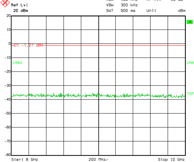
Figure 8.4-6: Conducted spurious emissions, high channel
