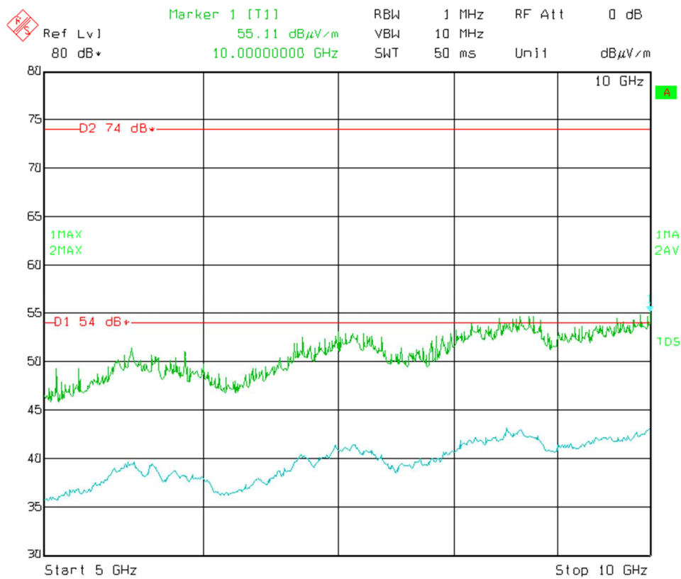
Figure 8.4-19: Radiated spurious emissions, mid channel, antenna in horizontal polarization, frequency range 5 to 10 GHz
