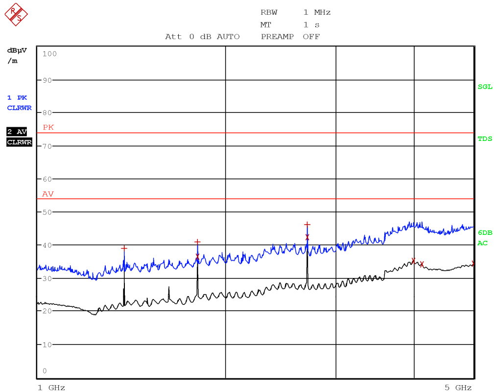
Figure 8.4-12: Radiated spurious emissions, low channel, antenna in vertical polarization, frequency range 1 to 5 GHz
