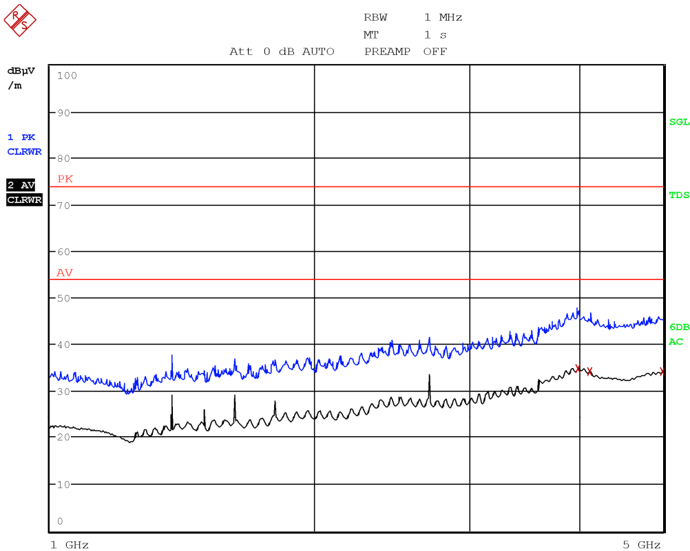
Figure 8.4-11: Radiated spurious emissions, low channel, antenna in horizontal polarization, frequency range 1 to 5 GHz
