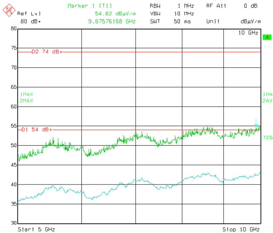
Figure 8.4-22: Radiated spurious emissions, high channel, antenna in vertical polarization, frequency range 5 to 10 GHz
