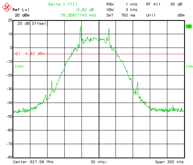
Figure 8.2-3: 20 dB bandwidth on high channel
