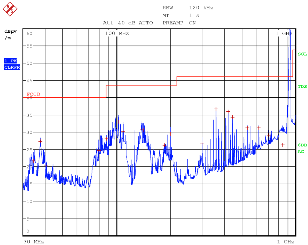
Figure 8.4-10: Radiated spurious emissions, high channel, antenna in vertical polarization, frequency range 30 to 1000 MHz
