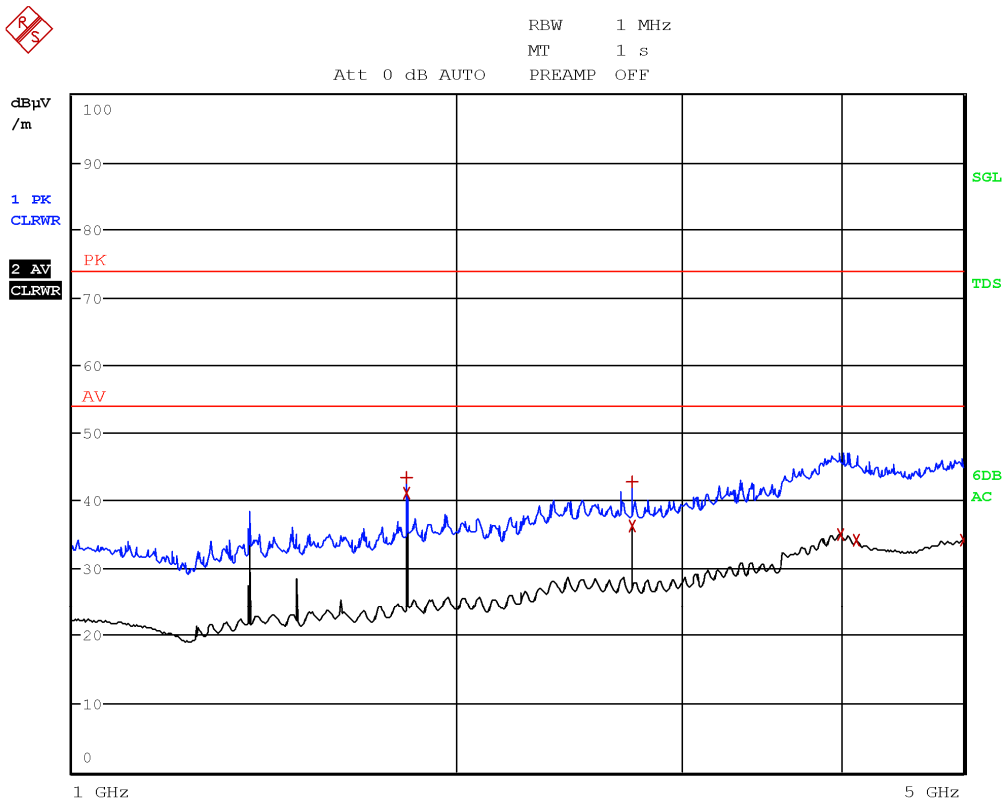
Figure 8.4-14: Radiated spurious emissions, mid channel, antenna in vertical polarization, frequency range 1 to 5 GHz
