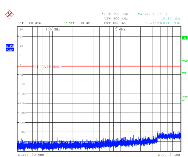
Figure 8.4-1: Conducted spurious emissions, low channel
