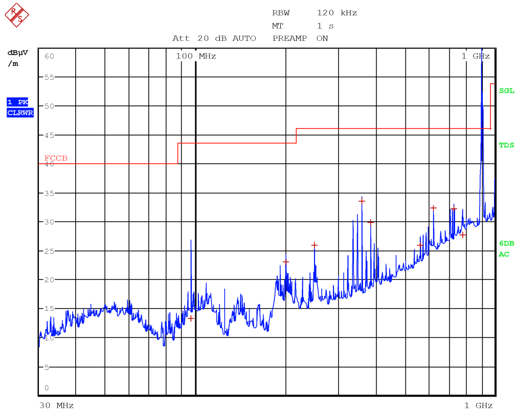
Figure 8.4-7: Radiated spurious emissions, low channel, antenna in horizontal polarization, frequency range 30 to 1000 MHz
