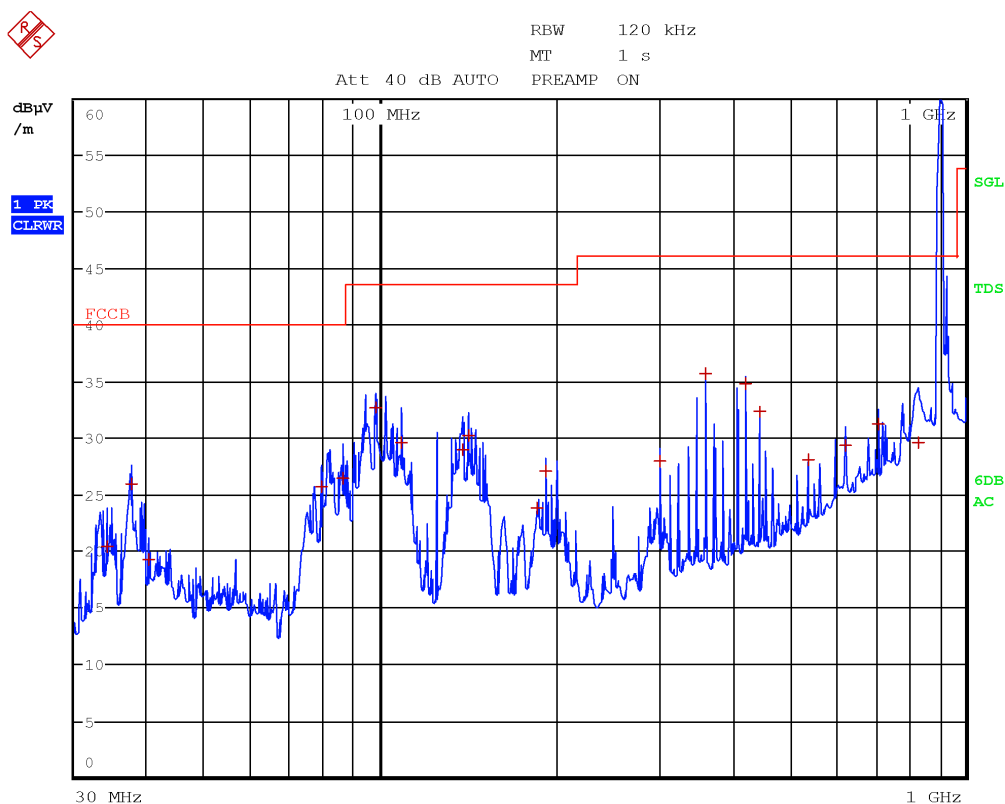
Figure 8.4-8: Radiated spurious emissions, low channel, antenna in vertical polarization, frequency range 30 to 1000 MHz
