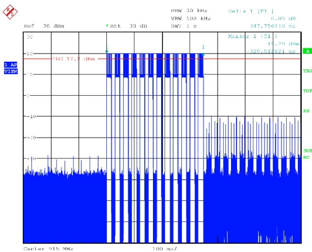
Figure 8.2-6: Dwell time
