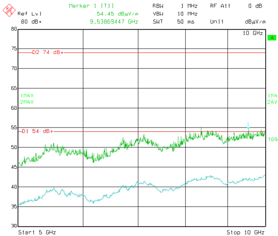
Figure 8.4-21: Radiated spurious emissions, high channel, antenna in horizontal polarization, frequency range 5 to 10 GHz
