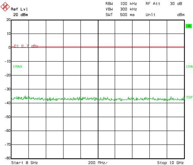
Figure 8.4-4: Conducted spurious emissions, mid channel
