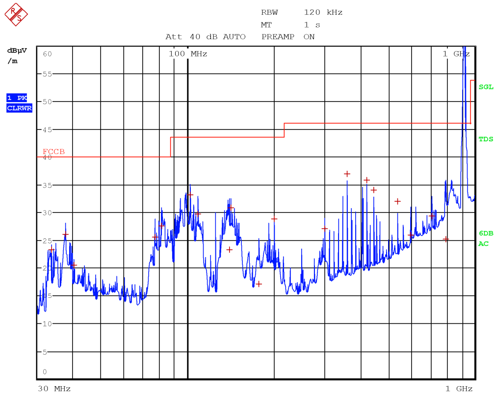
Figure 8.4-9: Radiated spurious emissions, mid channel, antenna in vertical polarization, frequency range 30 to 1000 MHz
