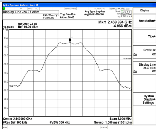
Channel 19 / 2440 MHz
