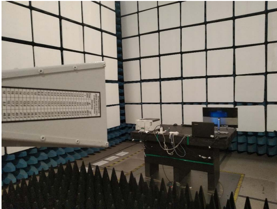
Above 1 GHz(AC Adapter)
