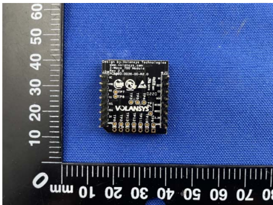
ZWAVE MODULE REAR VIEW ---2# circuit
