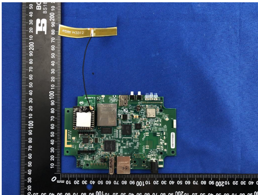
MAIN BOARD TOP VIEW WITHOUT FILTER (WITH SHIELDING)
