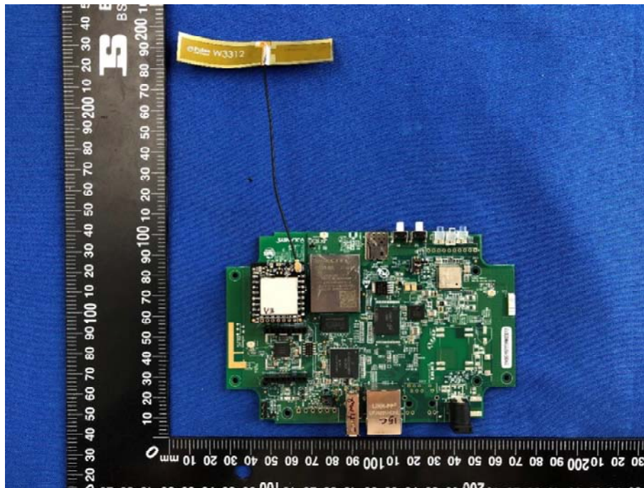
MAIN BOARD TOP VIEW WITH FILTER (WITH SHIELDING)
