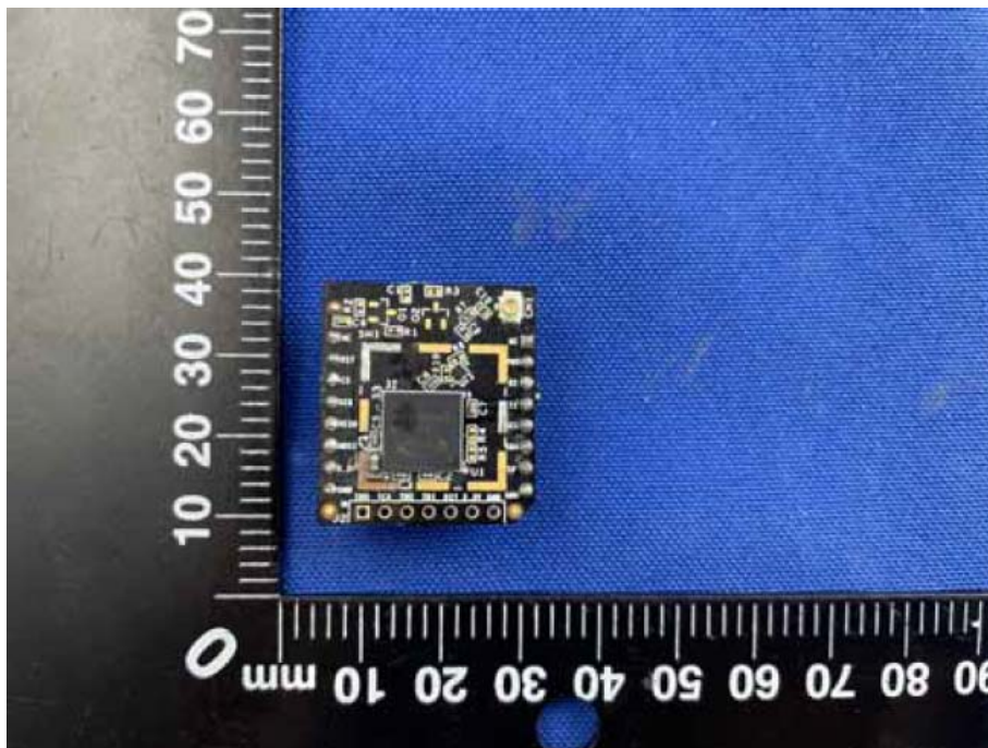
ZWAVE MODULE TOP VIEW ---1# circuit:
