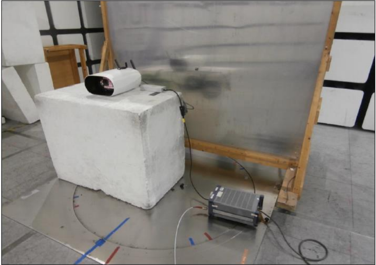
Figure 1 Conducted Disturbance at Mains Terminals
