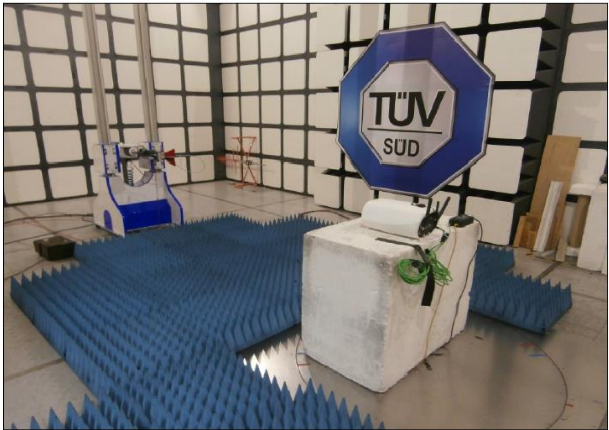
Figure 3 Radiated Disturbance 1GHz – 18GHz
