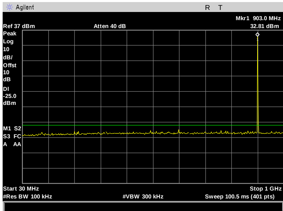
Figure 50.Part 90M_Lowband_902.75MHz_500KHz_25dBm_30MHz-1GHz_Port 2
