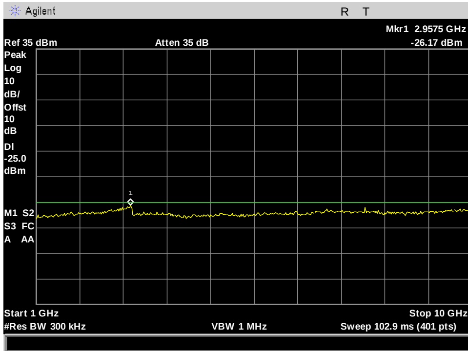
Figure 47.Part 90M_Dense_Mid Ch_915.75MHz_500KHz_-25dBm_1-10GHz_Port 2
