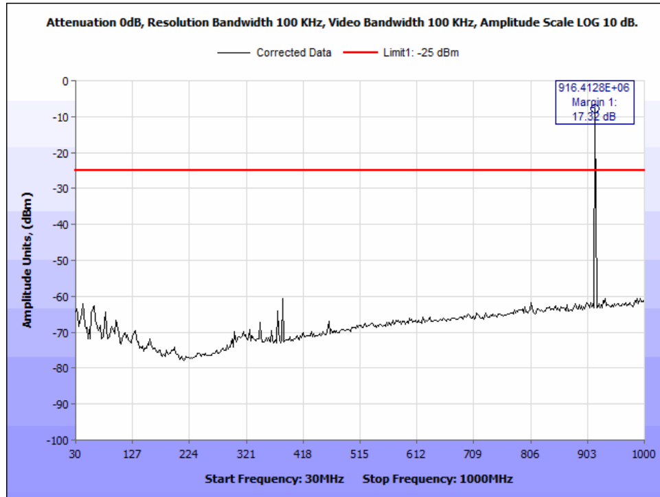
Figure 57.Cabinet Radiated Spurious Emissions_FCC Part90 dense_mid channel 915.75MHz_30-1000MHz
