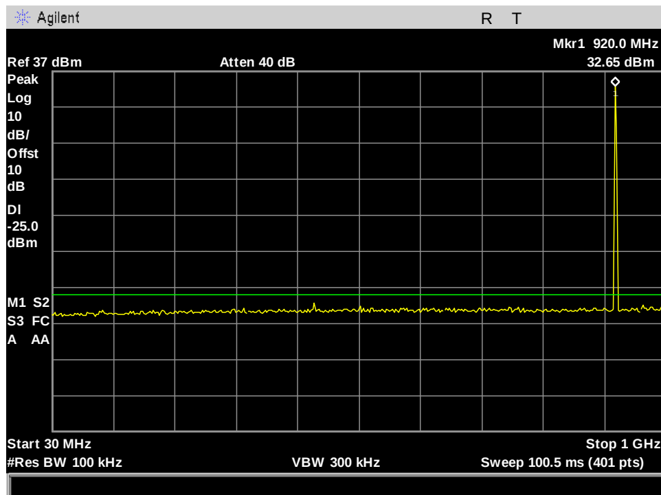
Figure 44. Part 90M_Dense_High Ch_920.25MHz_500KHz_25dBm_30MHz-1GHz_Port 2
