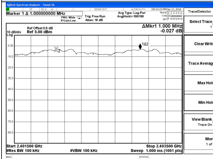
Channel 0 / 2402 MHz
