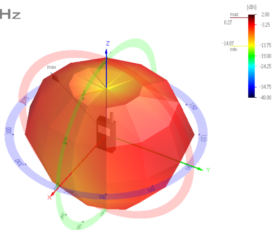
3D view (2.44GHz)
