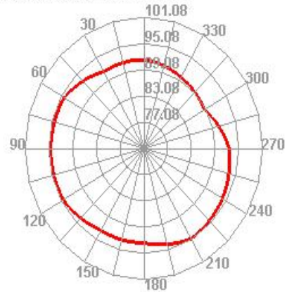
Bluetooth 0 TIS H
