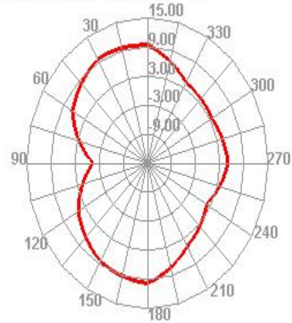
Bluetooth 0 TRP H
