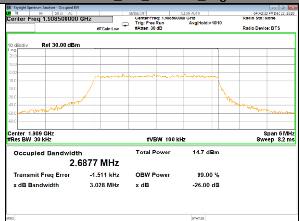
Band 2_3M_16QAM_High
