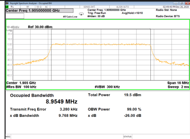
Band 2_10M_QPSK_High
