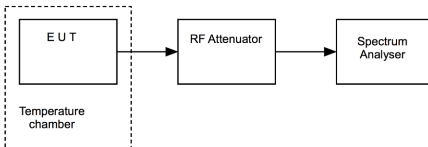
Figure v Test Setup
