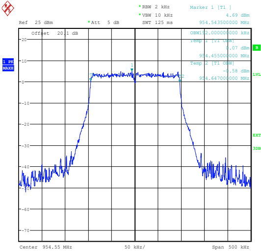
954.55 MHz
