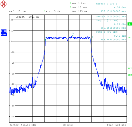
956.15 MHz
