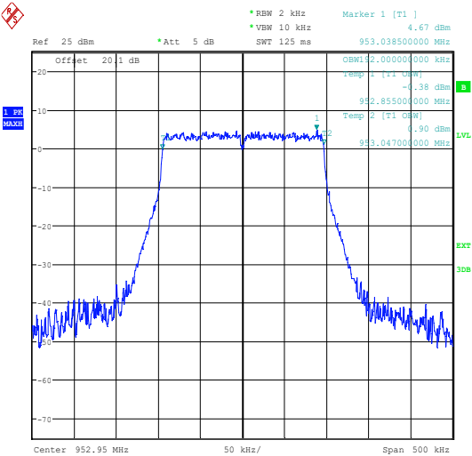
952.95 MHz
