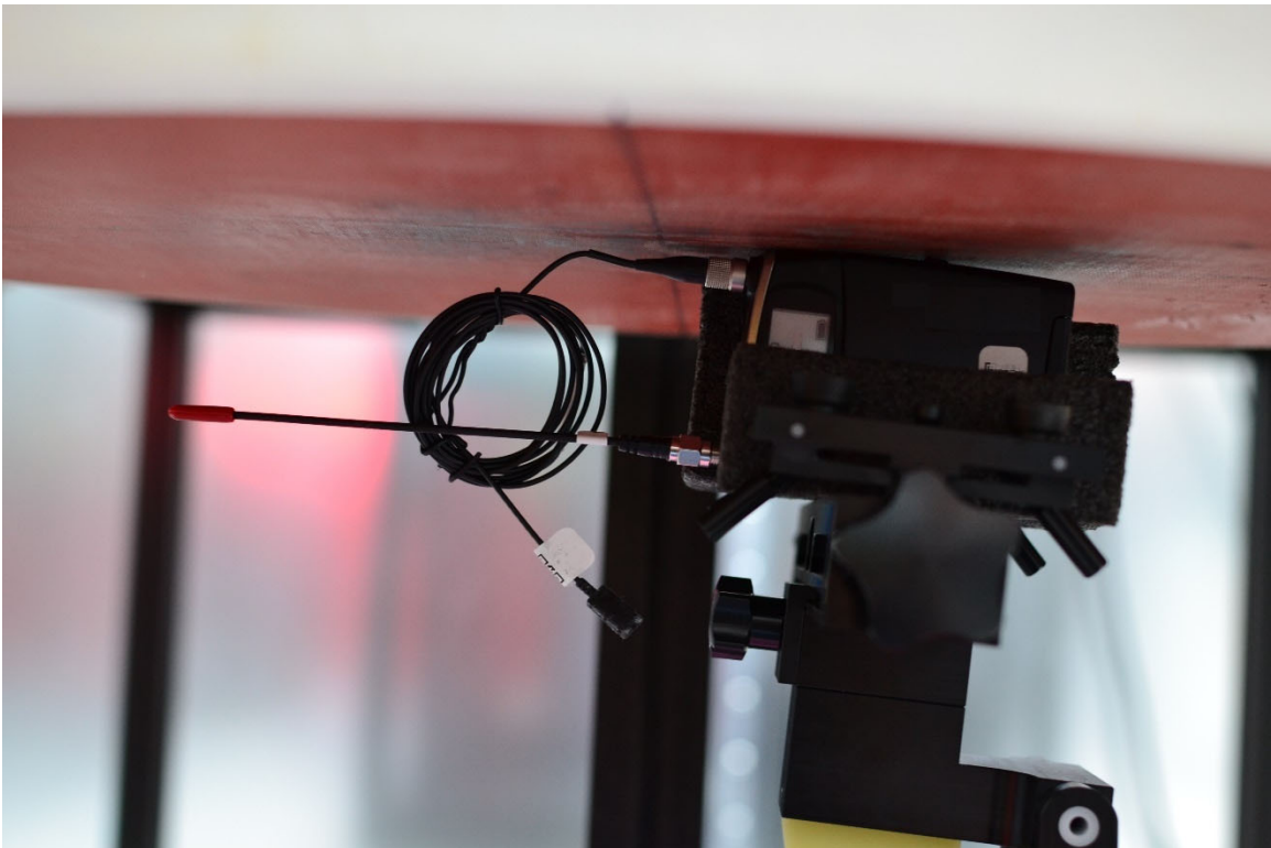
SAR Test Setup Photo 4 – Body/Extremity, Right Side at 0mm – Antenna 1
