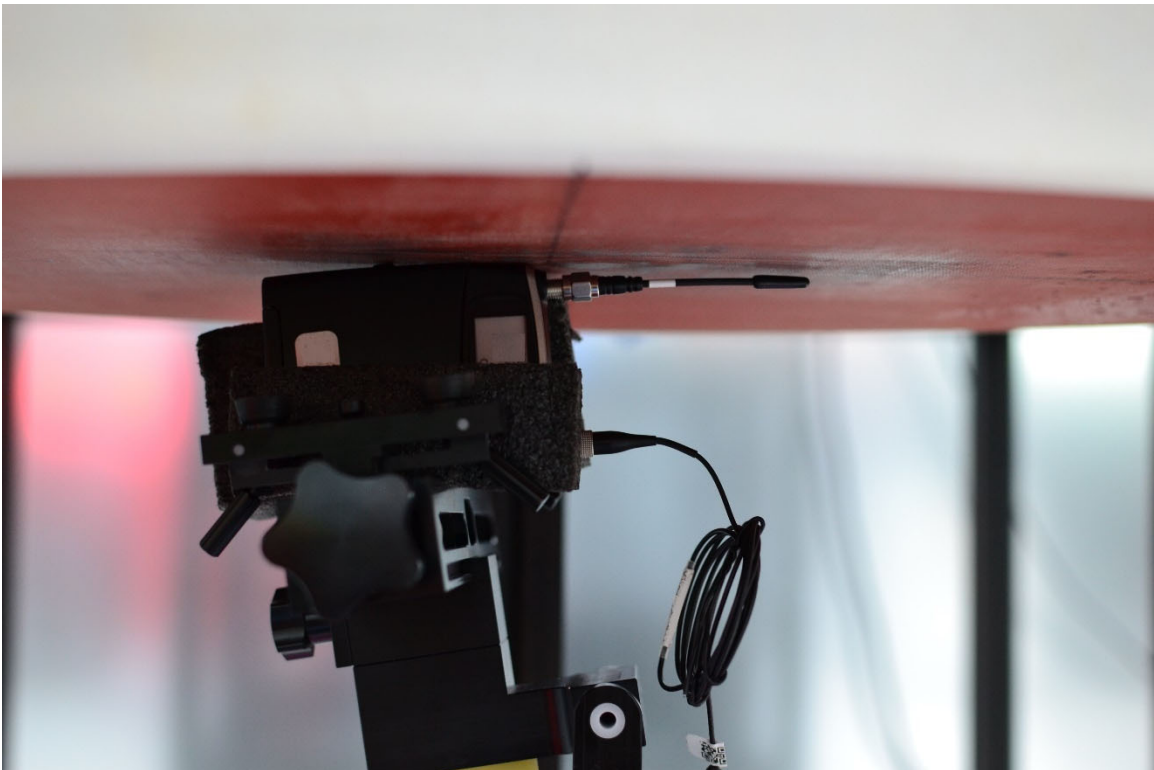
SAR Test Setup Photo 18 – Body/Extremity, Left Side at 0mm – Antenna 5
