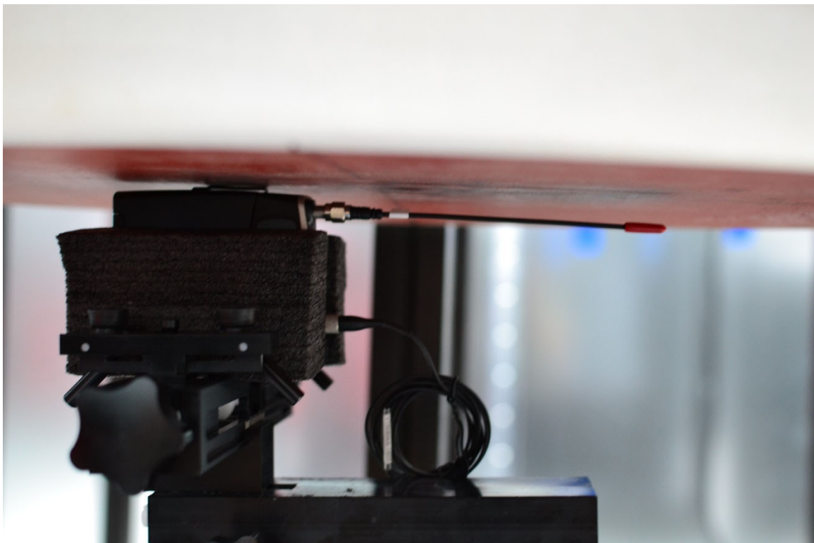
SAR Test Setup Photo 6 – Body/Extremity, Left Side at 0mm with Belt-clip installed – Antenna 1
