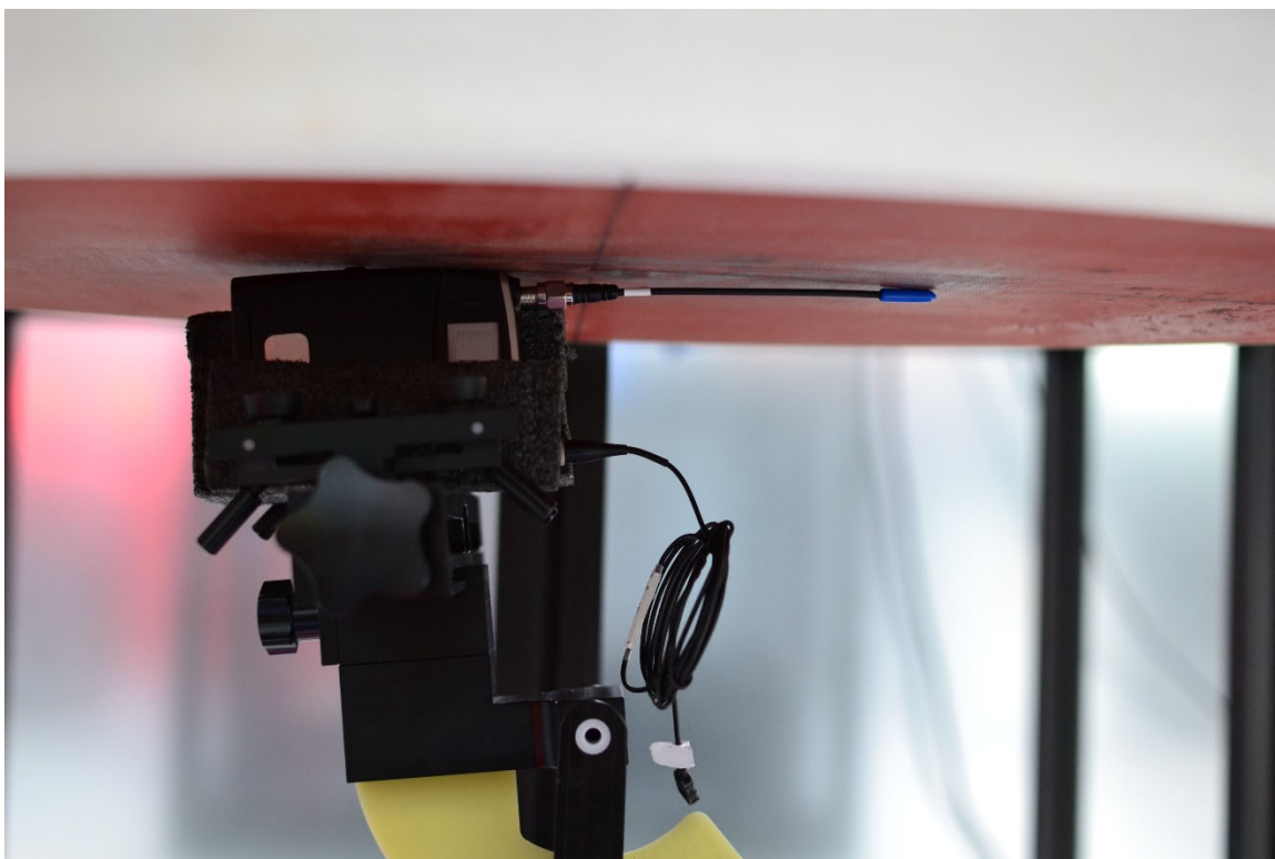
SAR Test Setup Photo 12 – Body/Extremity, Left Side at 0mm – Antenna 2
