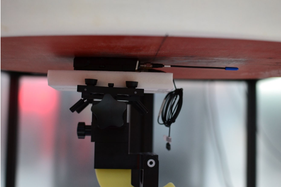
SAR Test Setup Photo 7 – Body/Extremity, Back Side at 0mm – Antenna 2
