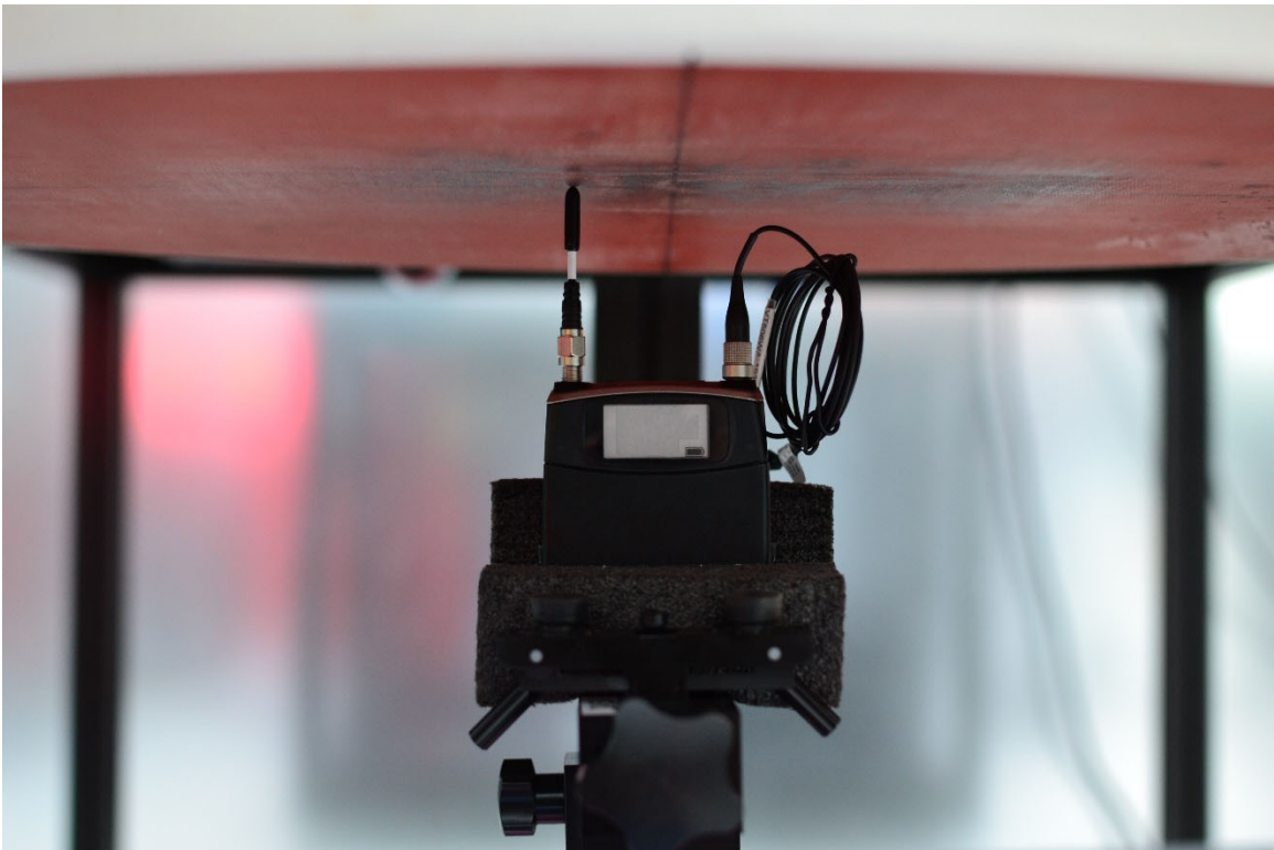
SAR Test Setup Photo 22 – Body/Extremity, Top Side at 0mm – Antenna 7
