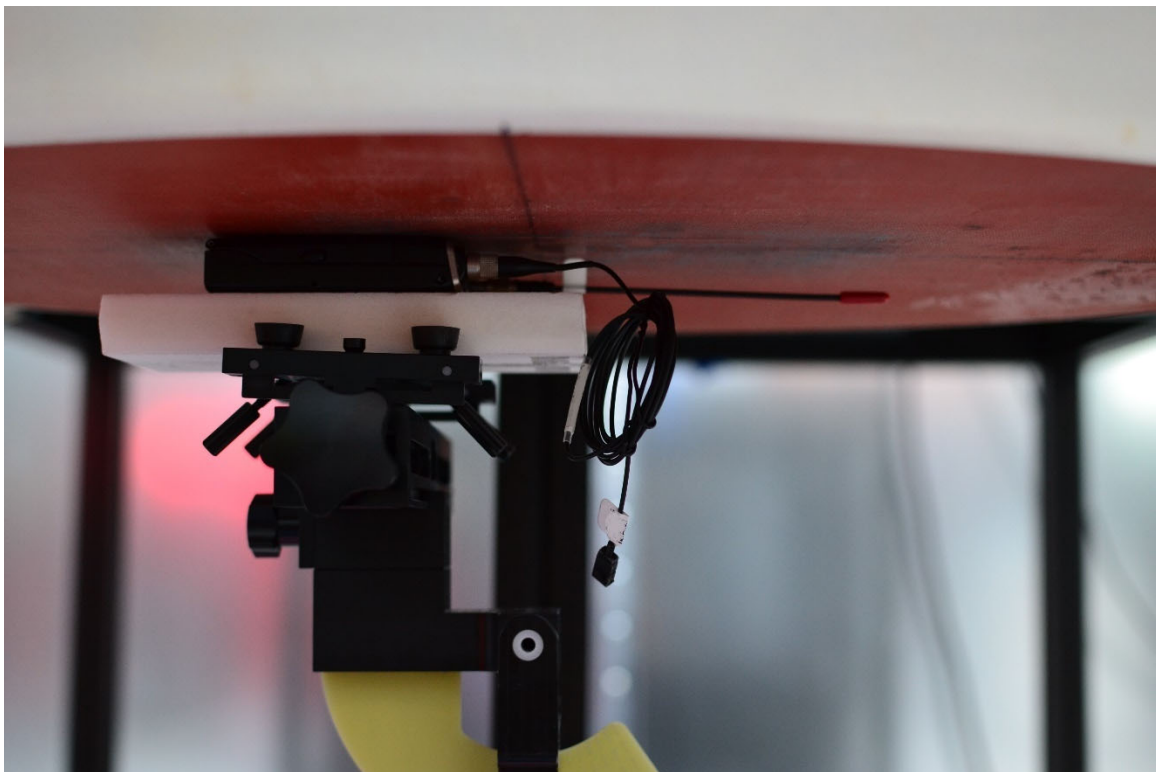
SAR Test Setup Photo 2 – Body/Extremity, Front Side at 0mm – Antenna 1
