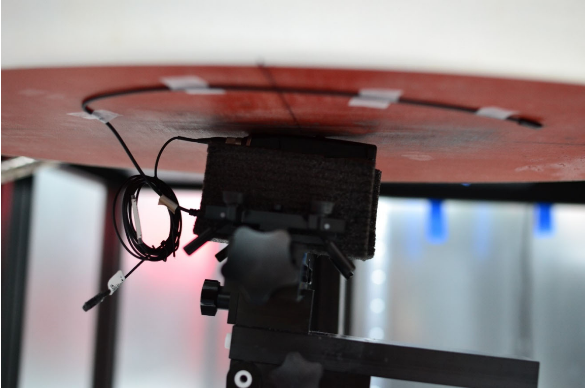
SAR Test Setup Photo 31 – Body/Extremity, Right Side at 0mm – Antenna 8
