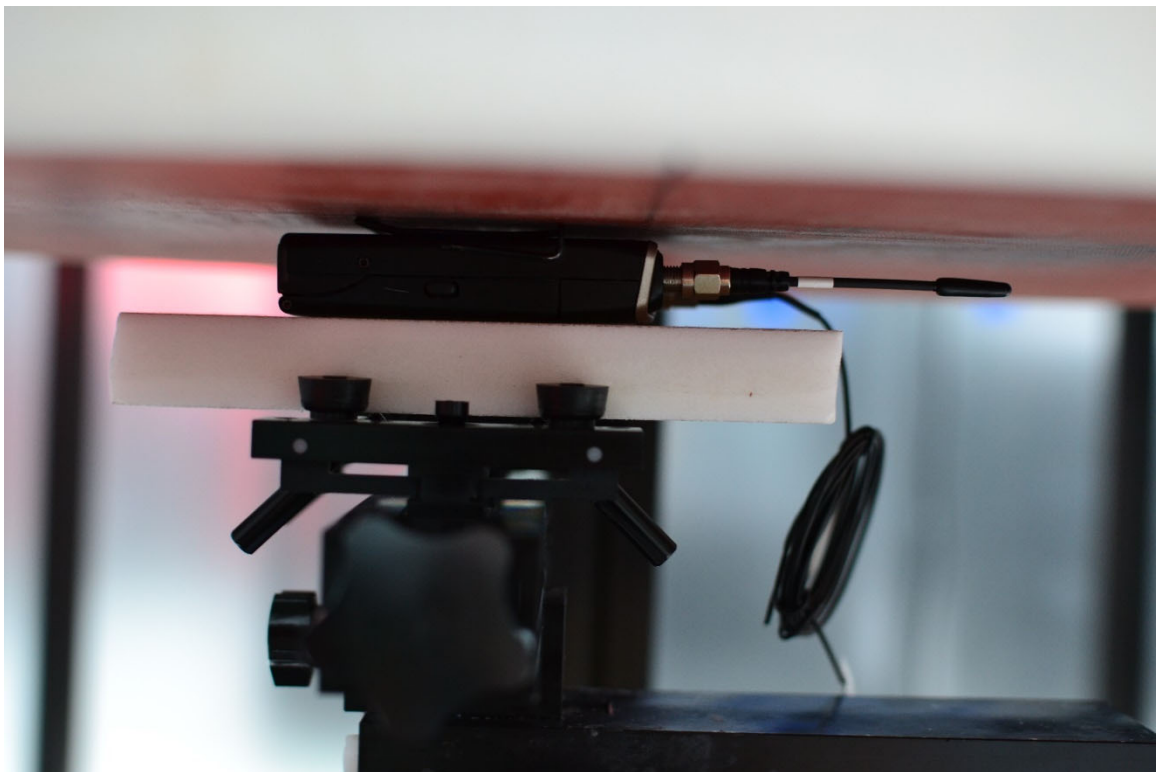
SAR Test Setup Photo 14 – Body/Extremity, Back Side at 0mm with Belt-clip installed – Antenna 5
