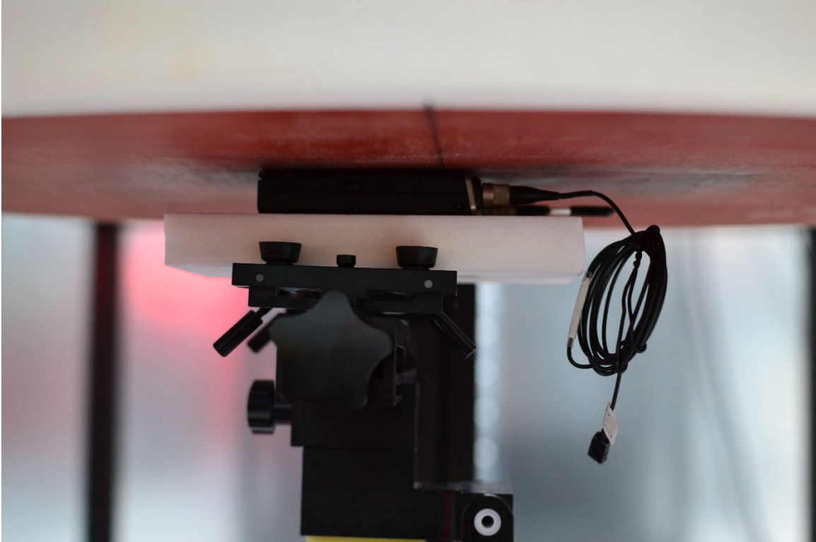
SAR Test Setup Photo 21 – Body/Extremity, Front Side at 0mm – Antenna 7, BT LE & NexLink
