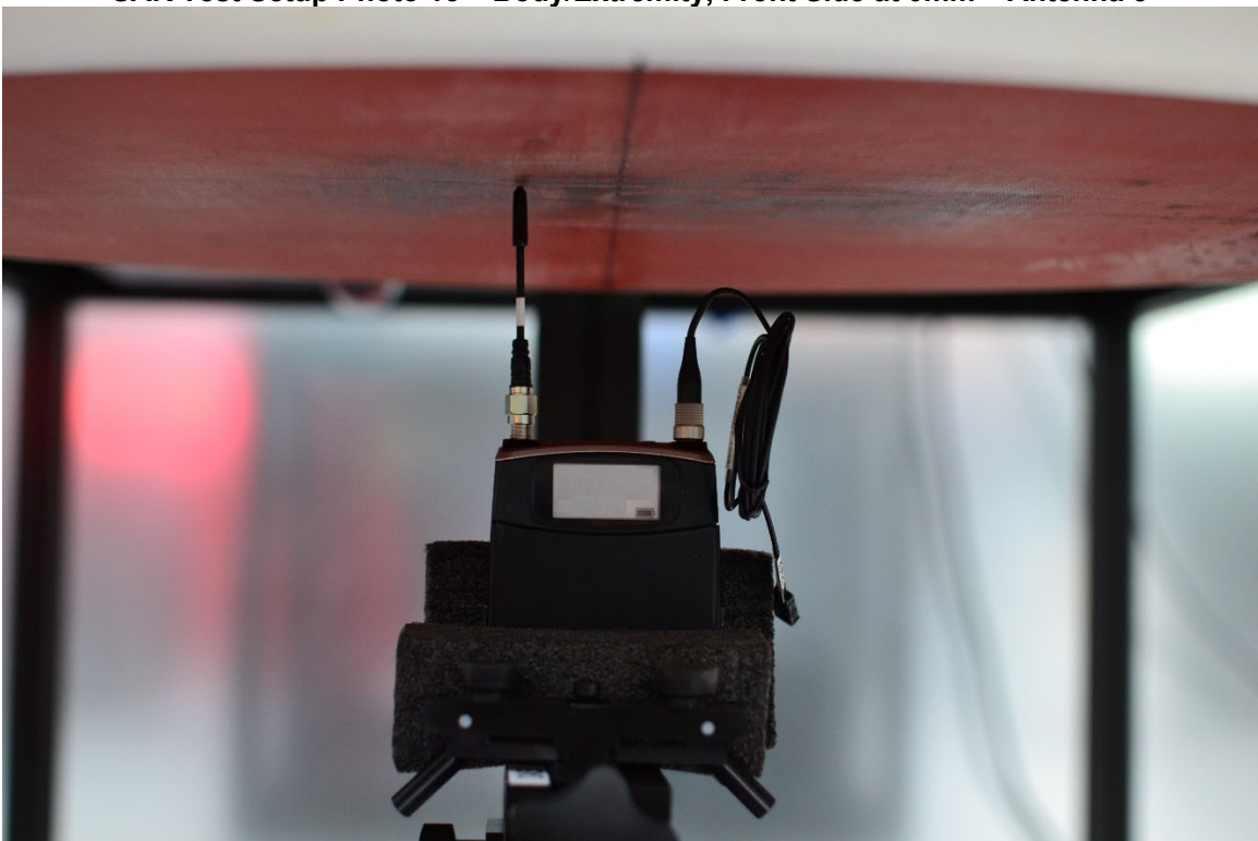
SAR Test Setup Photo 16 – Body/Extremity, Top Side at 0mm – Antenna 5
