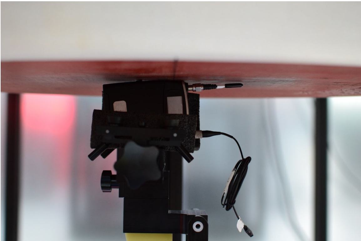
SAR Test Setup Photo 26 – Body/Extremity, Left Side at 0mm – Antenna 7
