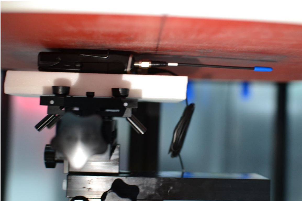
SAR Test Setup Photo 8 – Body/Extremity, Back Side at 0mm with Belt-clip installed – Antenna 2
