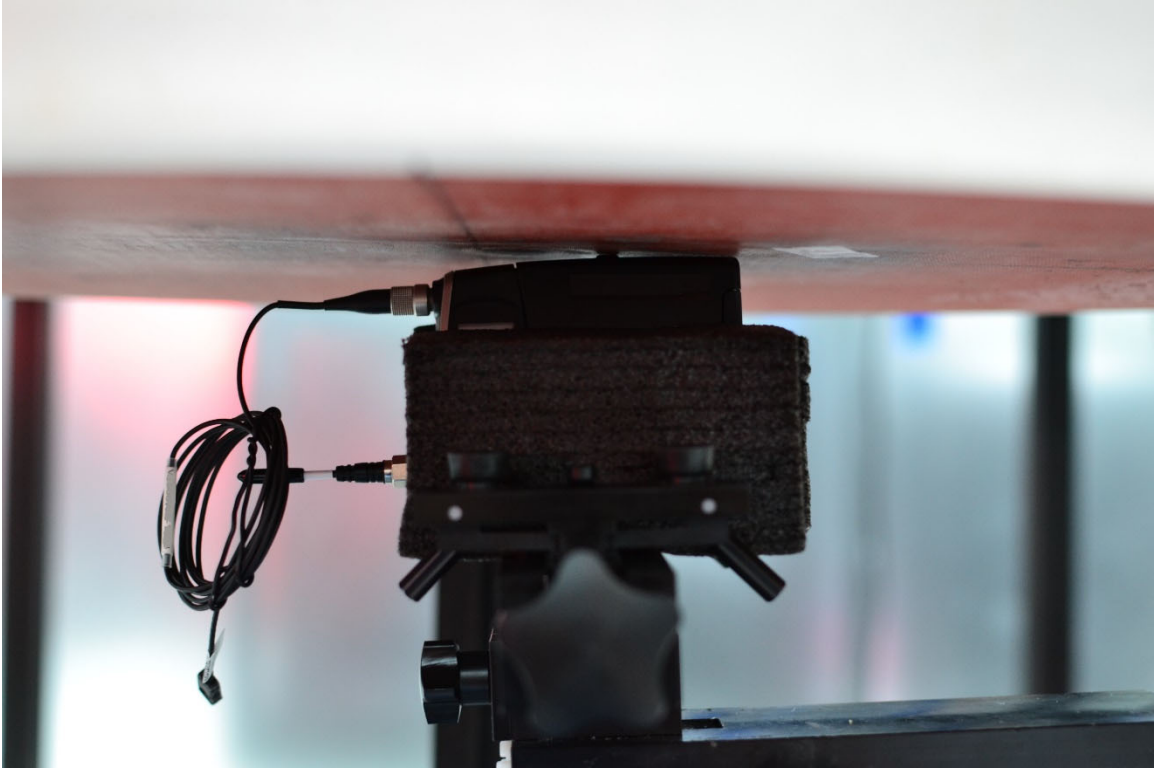
SAR Test Setup Photo 25 – Body/Extremity, Right Side at 0mm – BT LE & NexLink
