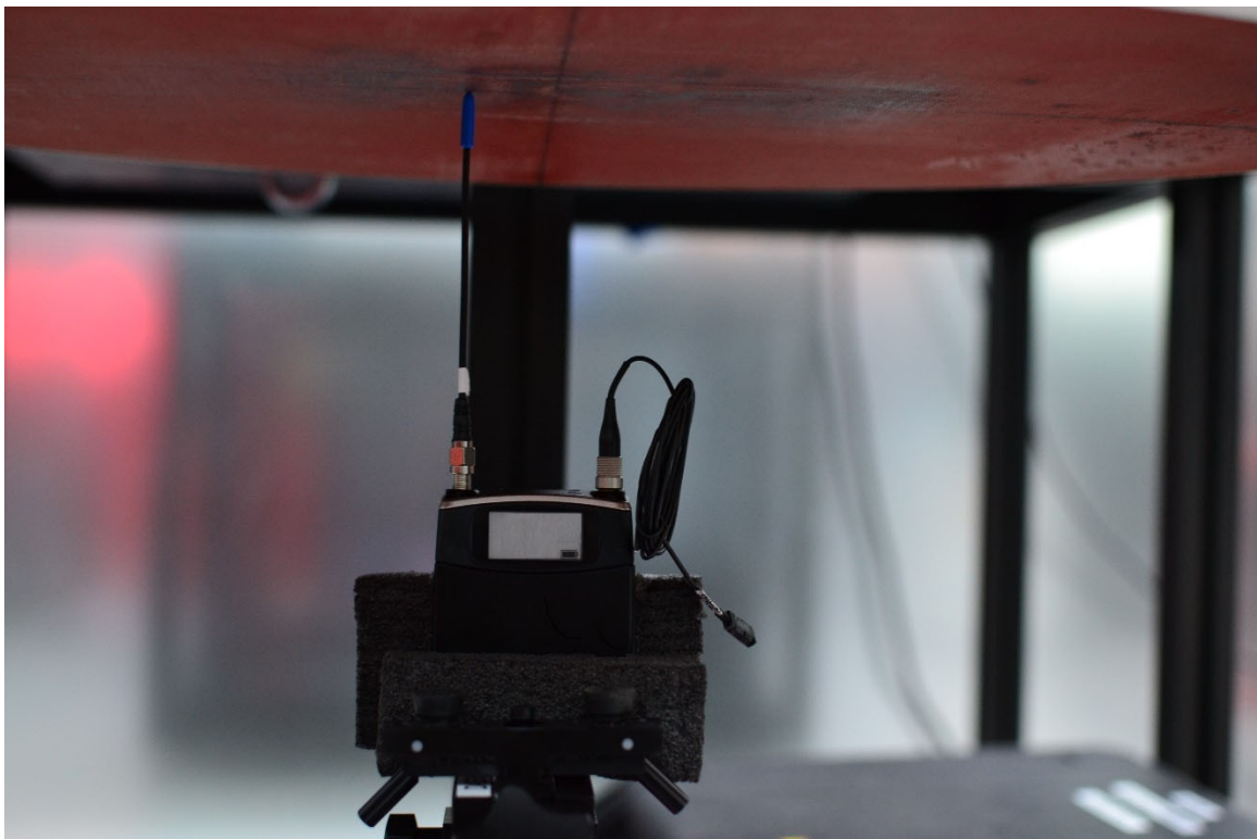
SAR Test Setup Photo 10 – Body/Extremity, Top Side at 0mm – Antenna 2
