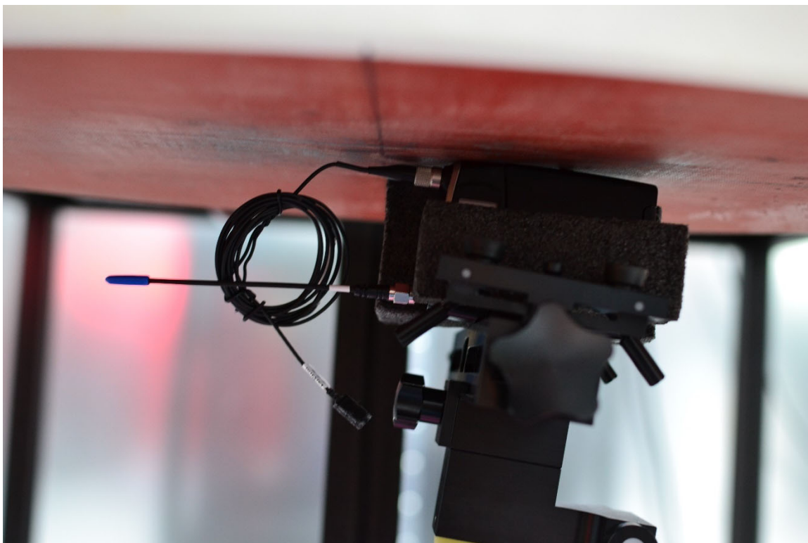
SAR Test Setup Photo 11 – Body/Extremity, Right Side at 0mm – Antenna 2
