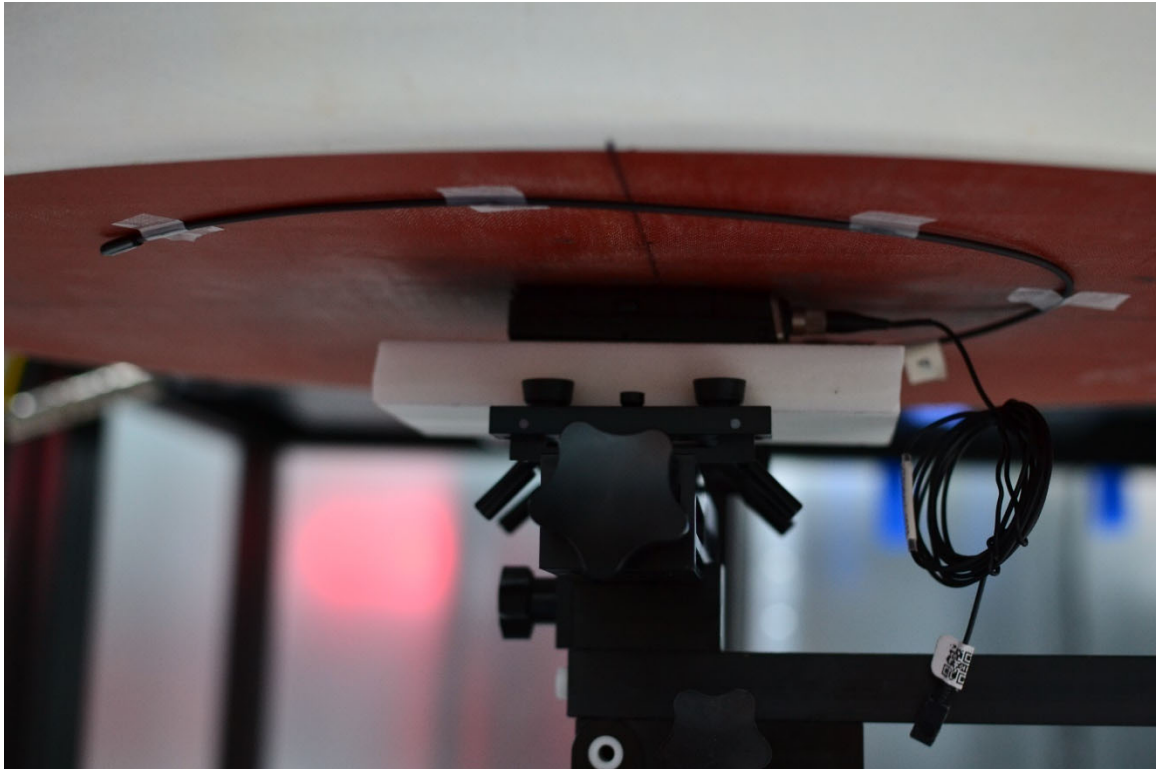
SAR Test Setup Photo 29 – Body/Extremity, Front Side at 0mm – Antenna 8
