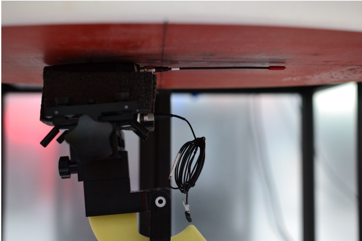
SAR Test Setup Photo 5 – Body/Extremity, Left Side at 0mm – Antenna 1
