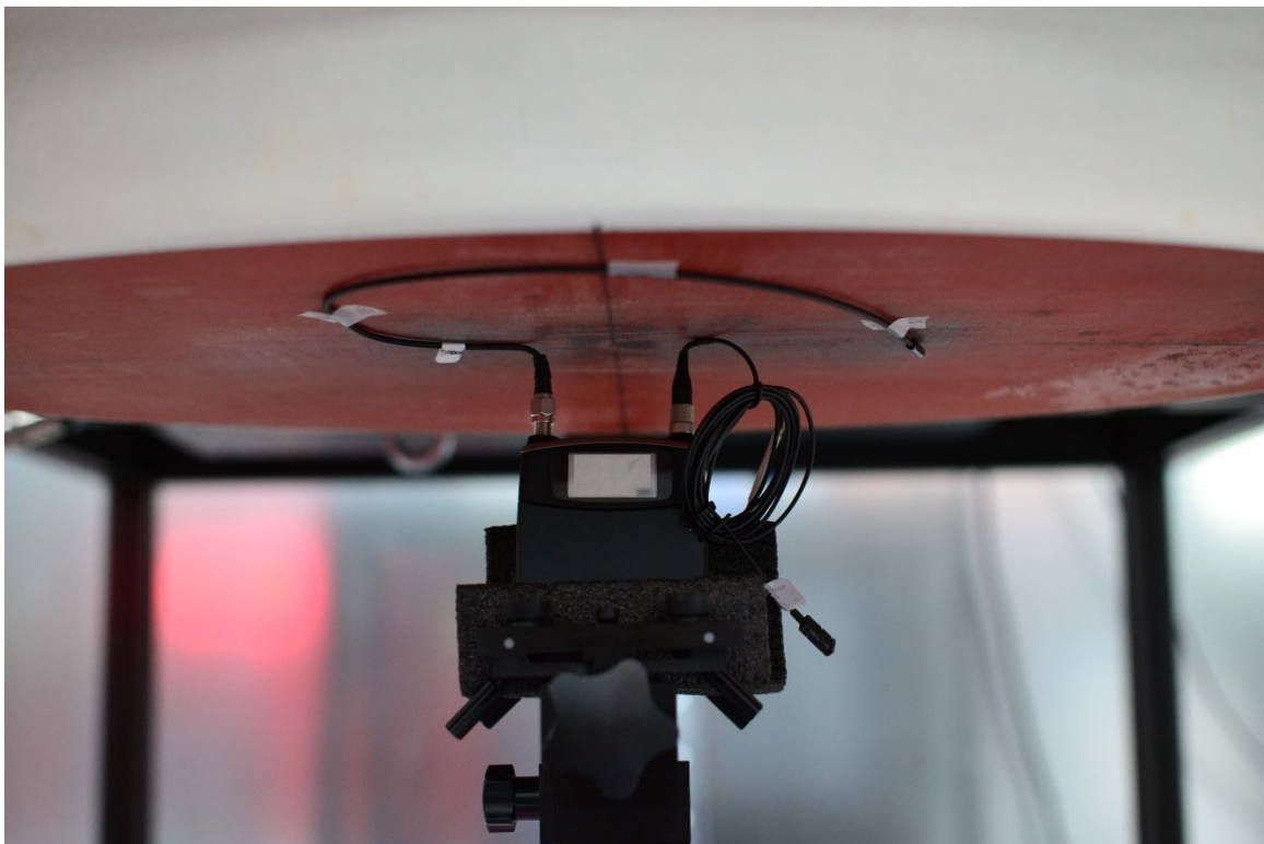
SAR Test Setup Photo 30 – Body/Extremity, Top Side at 0mm – Antenna 8
