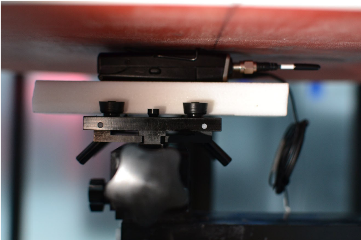
SAR Test Setup Photo 20 – Body/Extremity, Back Side at 0mm – Antenna 7, BT LE & NexLink with Belt-clip installed
