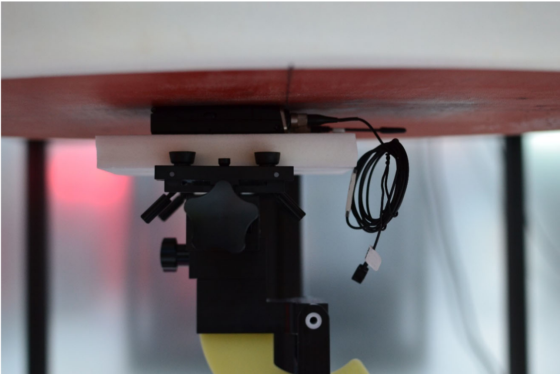
SAR Test Setup Photo 15 – Body/Extremity, Front Side at 0mm – Antenna 5
