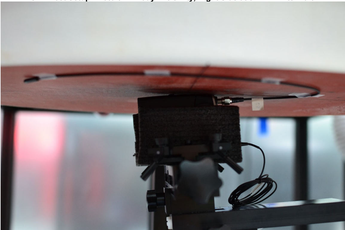
SAR Test Setup Photo 32 – Body/Extremity, Left Side at 0mm – Antenna 8
