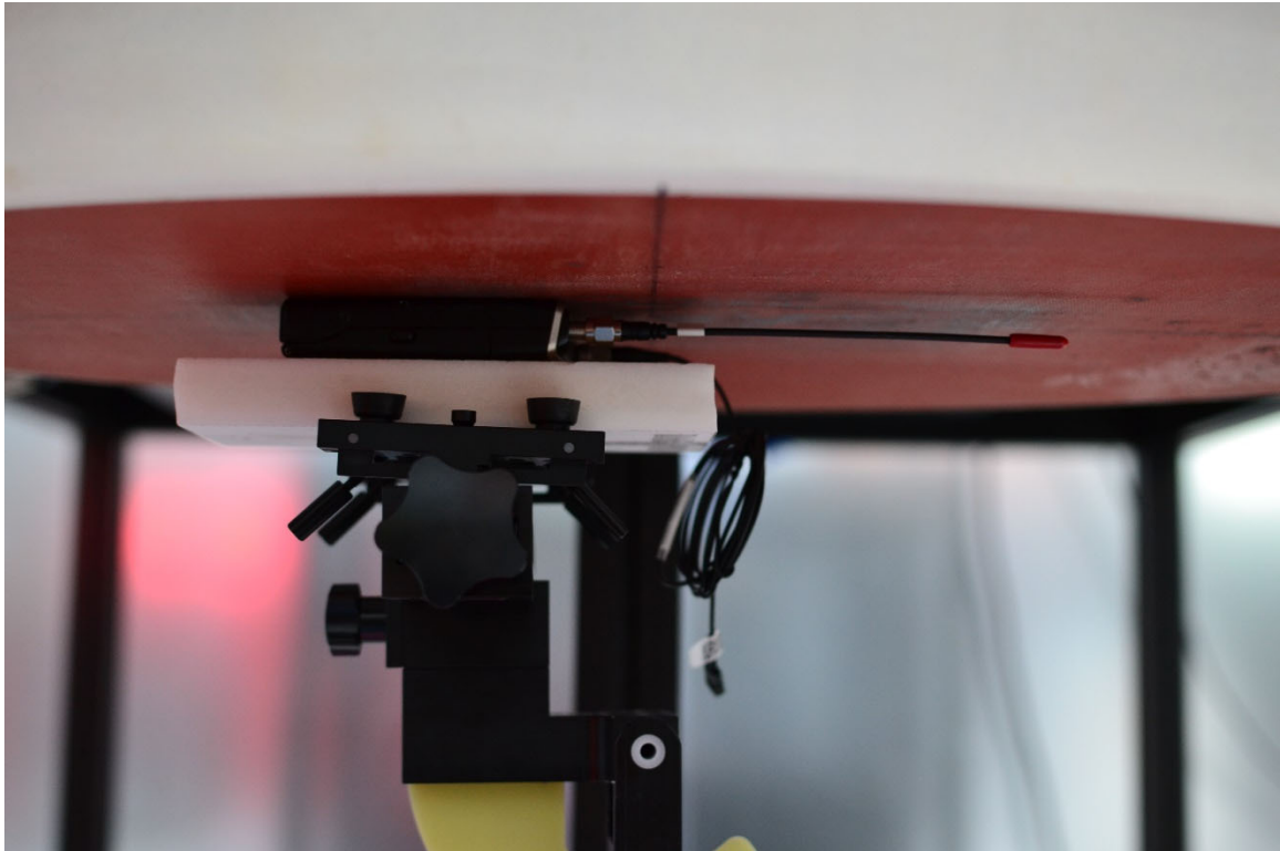
SAR Test Setup Photo 1 – Body/Extremity, Back Side at 0mm – Antenna 1
