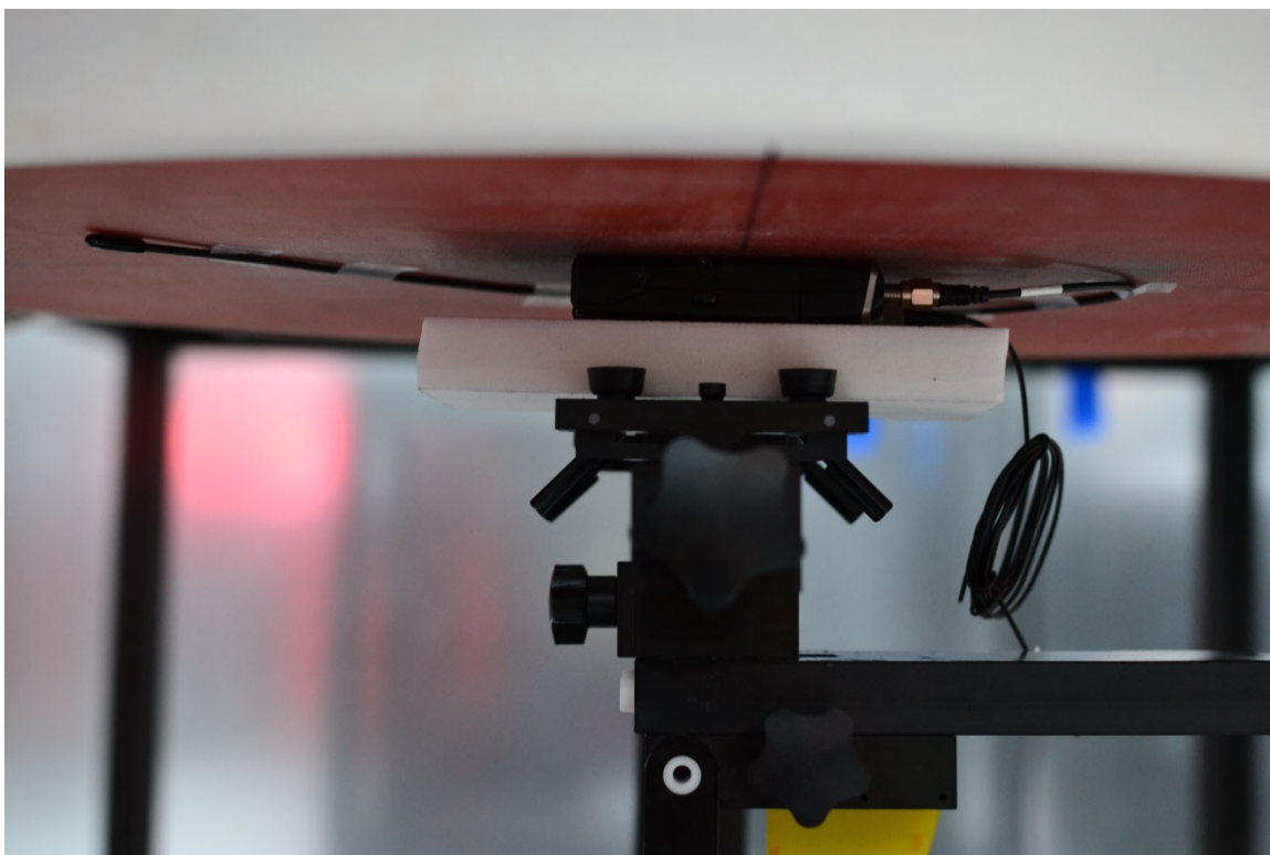
SAR Test Setup Photo 28 – Body/Extremity, Back Side at 0mm – Antenna 8
