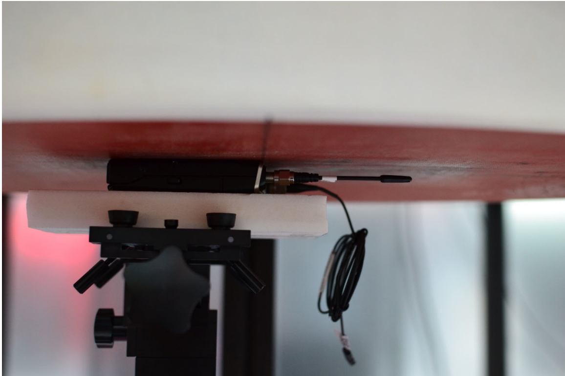
SAR Test Setup Photo 13 – Body/Extremity, Back Side at 0mm – Antenna 5
