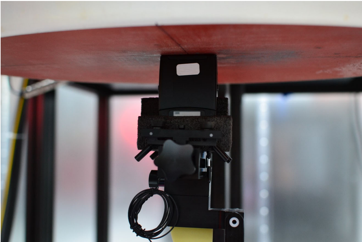
SAR Test Setup Photo 23 – Body/Extremity, Bottom Side at 0mm – BT LE & NexLink
