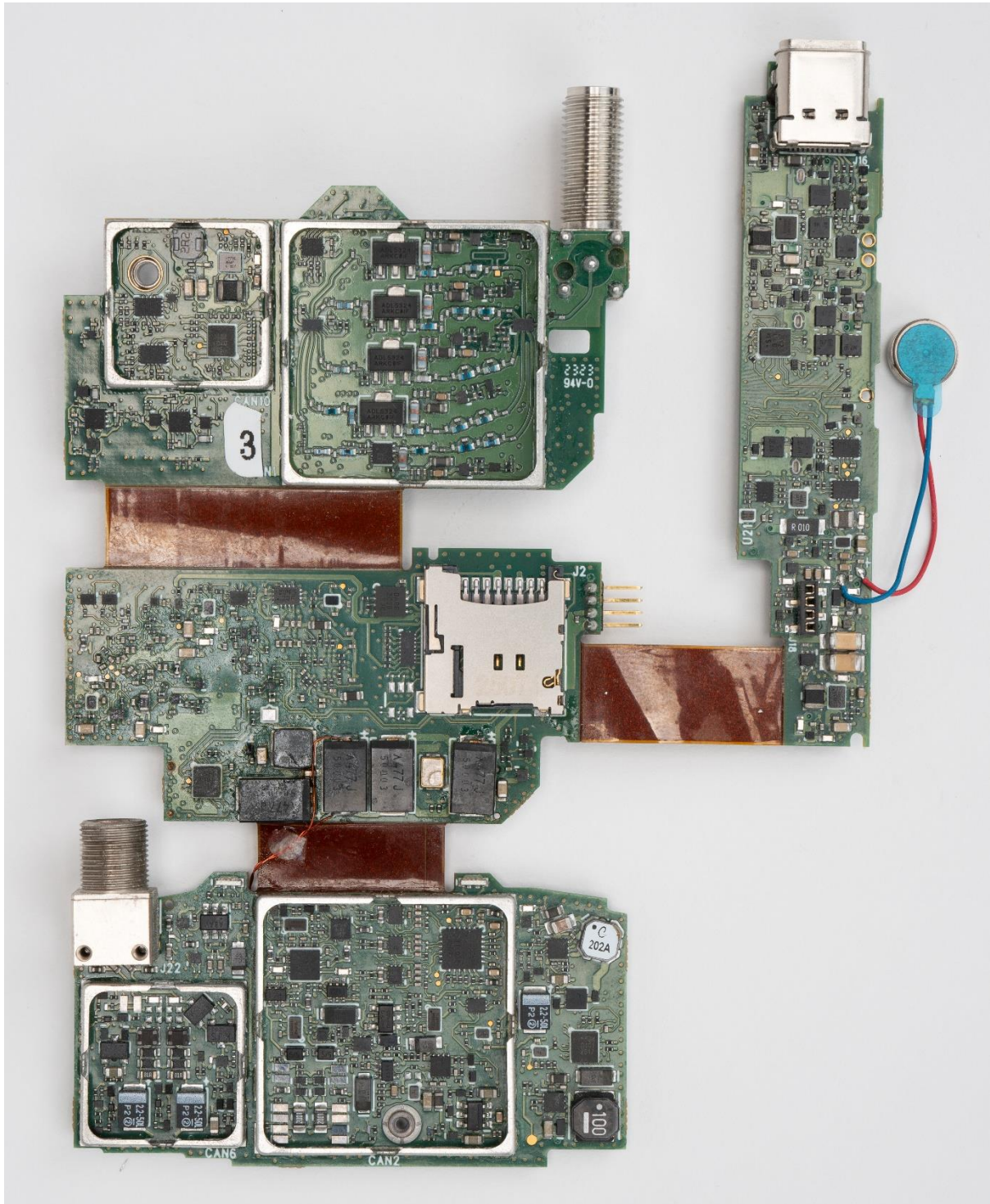
PCB-MAIN (REAR)
