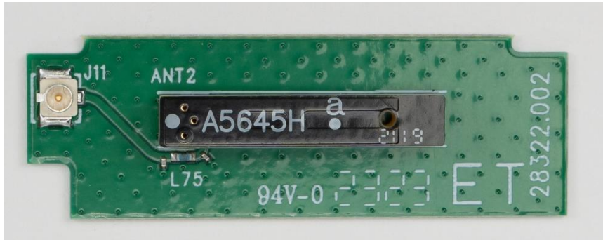
PCB-ANTENNA (FRONT)
