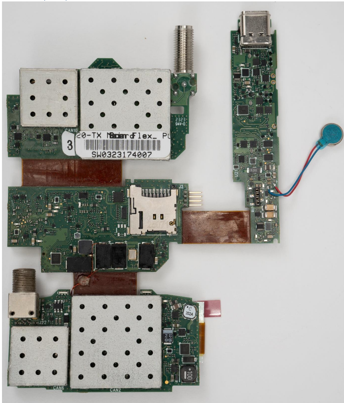
PCB-MAIN (REAR)
