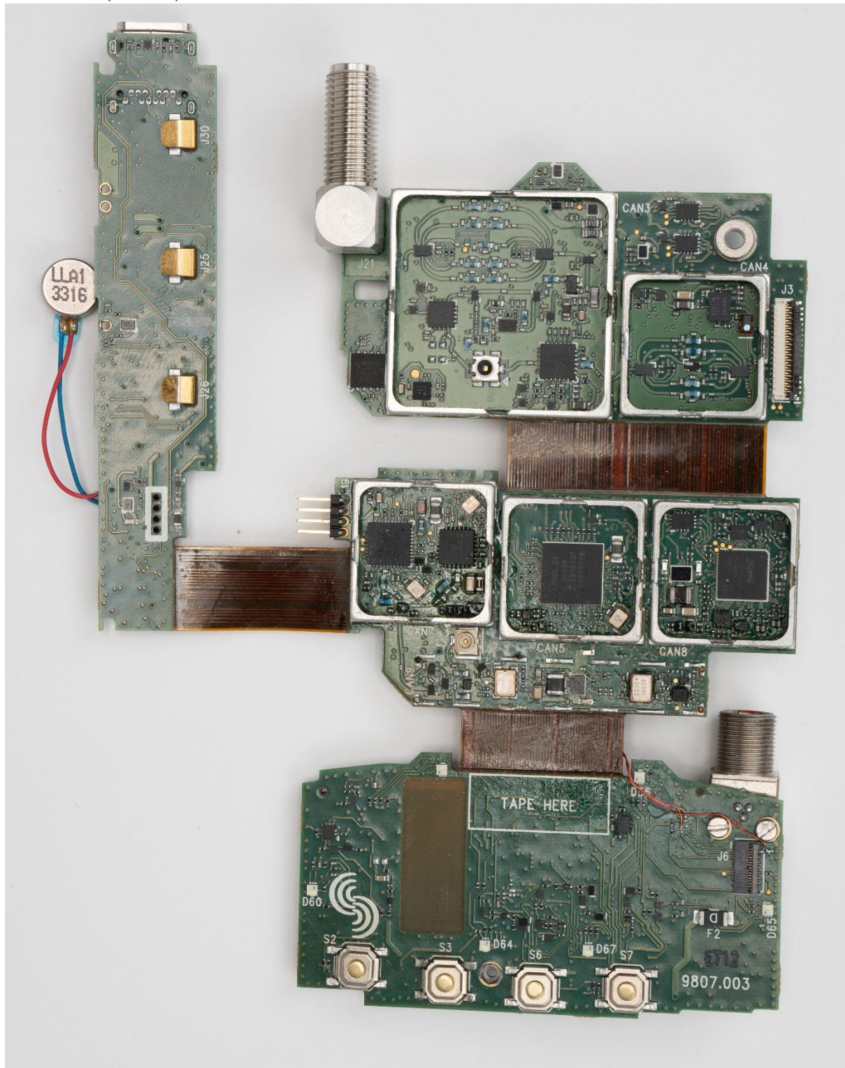
PCB-MAIN (FRONT)
