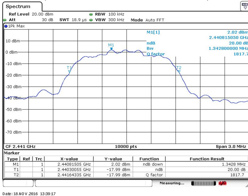
(Plot 4.4.2 B: Channel 39: 2441MHz @ 8DPSK)
