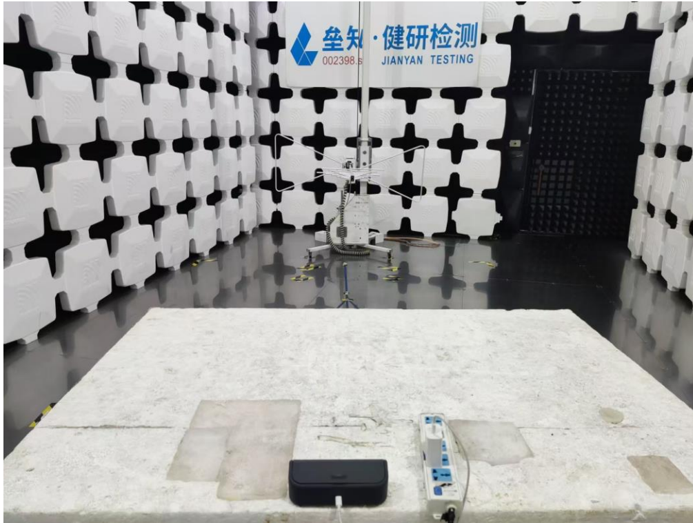
Charing mode Radiated Spurious Emission Below 1GHz
