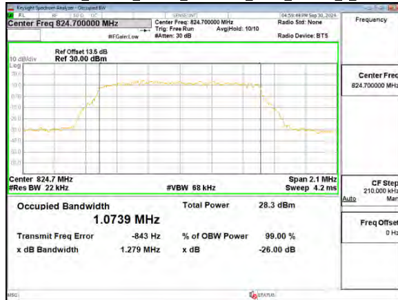
Band5_1.4MHz_Chain0_824.7MHz_NBI 0_QPSK_6_0
