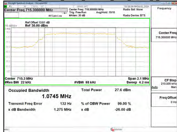
Band12_1.4MHz_Chain0_715.3MHz_NBI 0_QPSK_6_0
