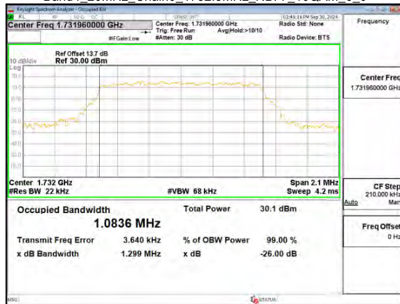
Band4_20MHz_Chain0_1732.5MHz_NBI_7_16QAM_6_0
