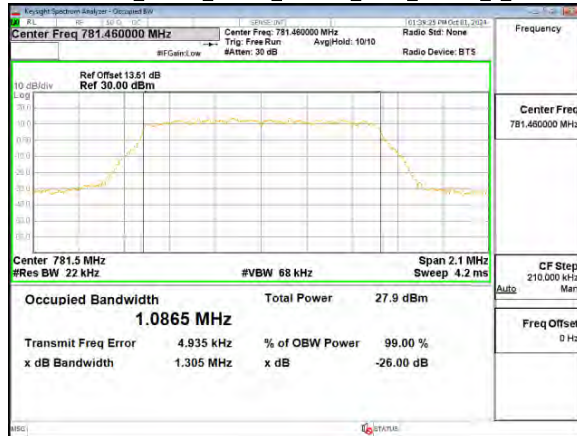
Band13_10MHz_Chain0_782MHz_NBI_3_QPSK_6_0
