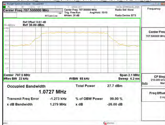
Band12_1.4MHz_Chain0_707.5MHz_NBI 0_16QAM_6_0
