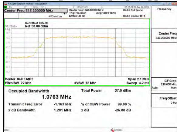
Band5_1.4MHz_Chain0_848.3MHz_NBI 0_QPSK_6_0
