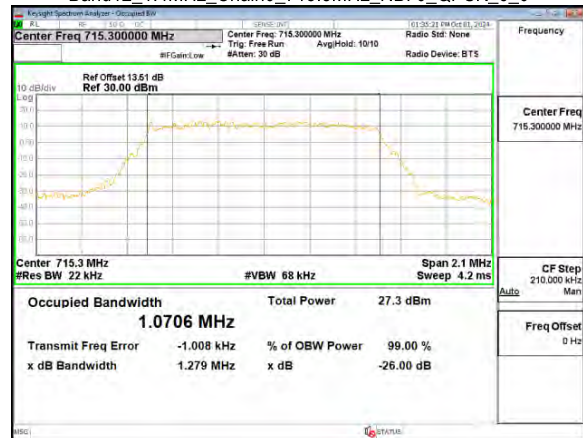
Band12_1.4MHz_Chain0_715.3MHz_NBI 0_QPSK_6_0
