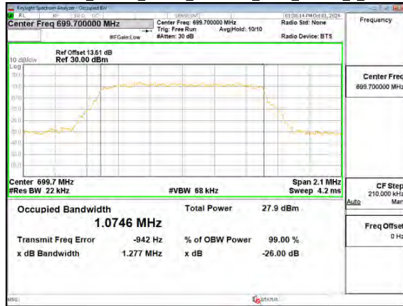
Band12_1.4MHz_Chain0_699.7MHz_NBI 0_QPSK_6_0
