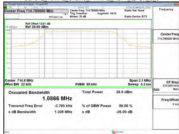
Band12_10MHz_Chain0_711MHz_NBI_7_QPSK_6_0
