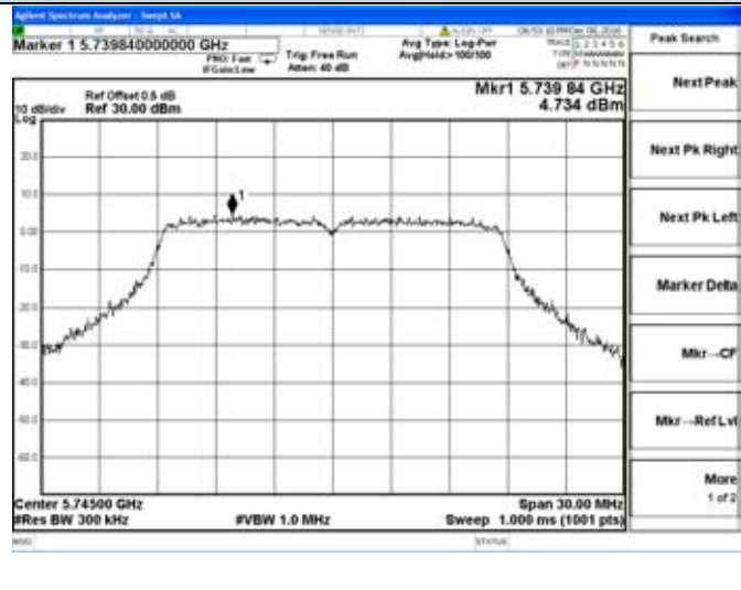
Chain 1-802.11n20-5745MHz
