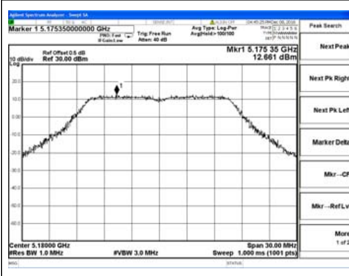
Chain 0-802.11a-5180MHz
