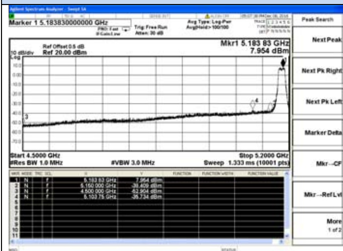
802.11n20-5180MHz-Lower
