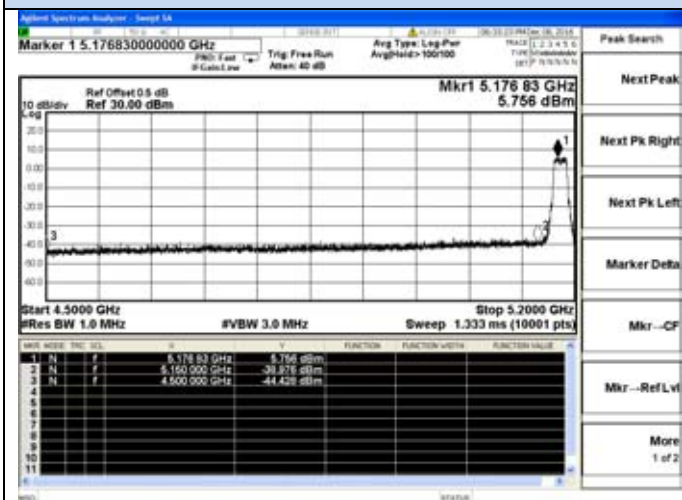
802.11n20-5180MHz-Lower
