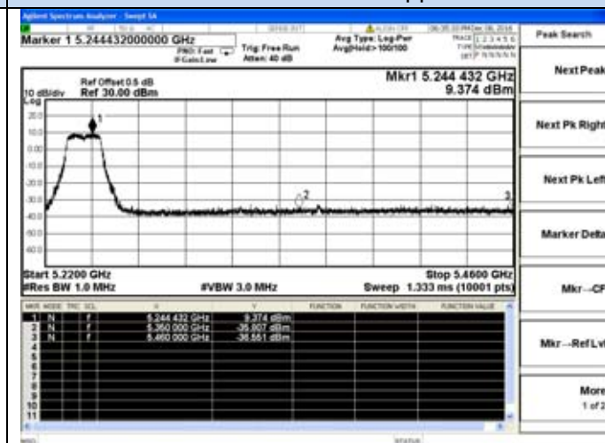
802.11n20-5240MHz-Upper
