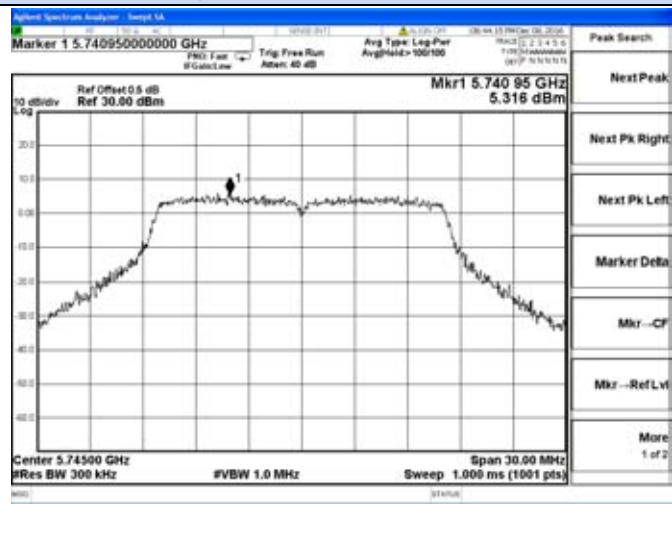
Chain 1-802.11a-5745MHz
