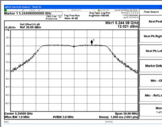
Chain 0-802.11a-5240MHz
