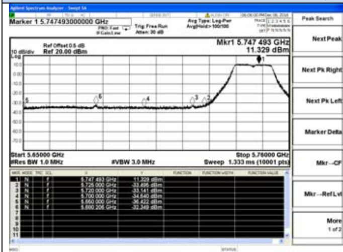
802.11a-5745MHz-Lower
