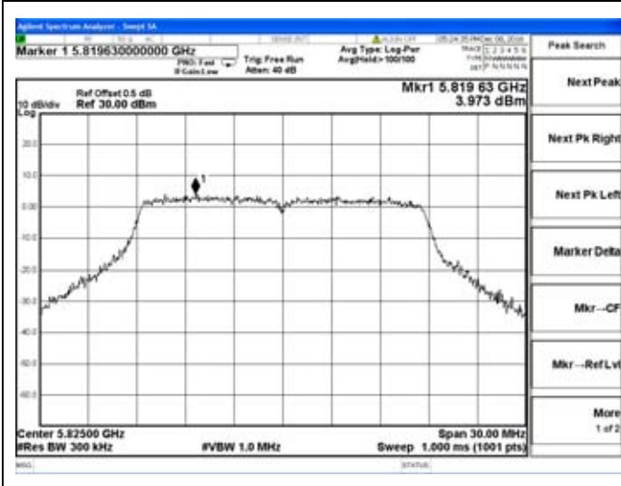
Chain 0-802.11n20-5825MHz
