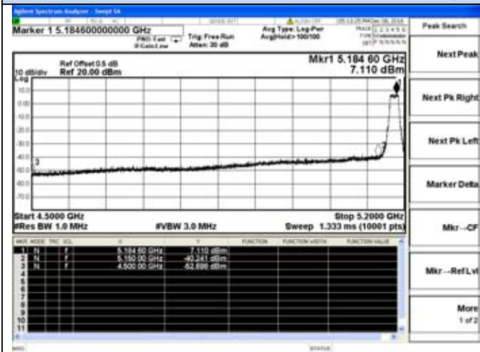
802.11a-5180MHz-Lower
