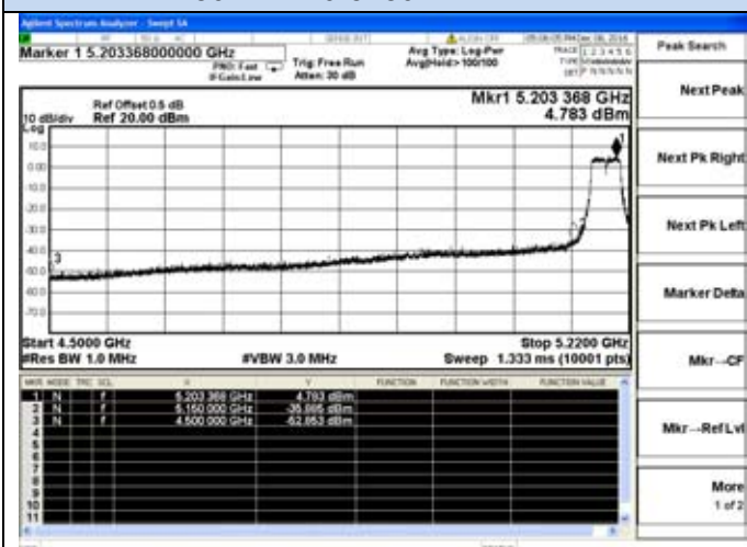
802.11n40-5190MHz-Lower
