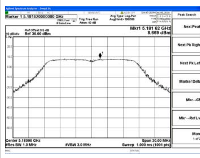
Chain 0-802.11n20-5180MHz
