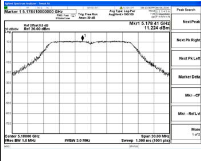
Chain 1-802.11a-5180MHz
