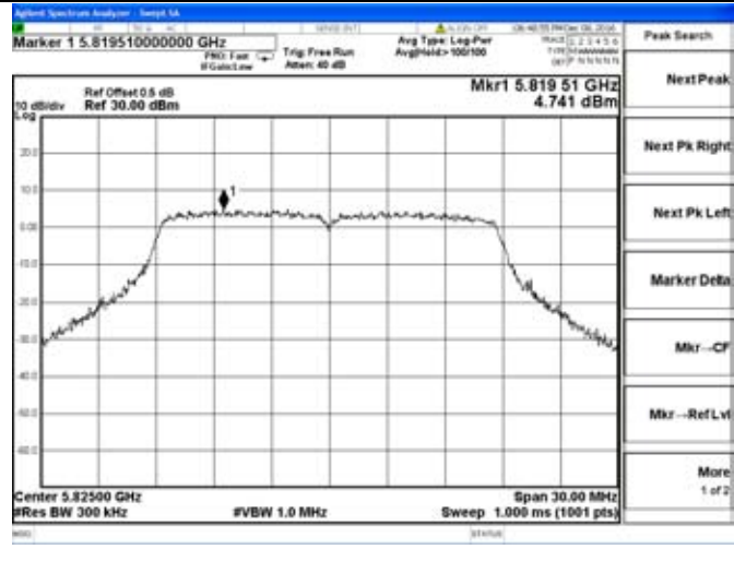
Chain 1-802.11n20-5825MHz
