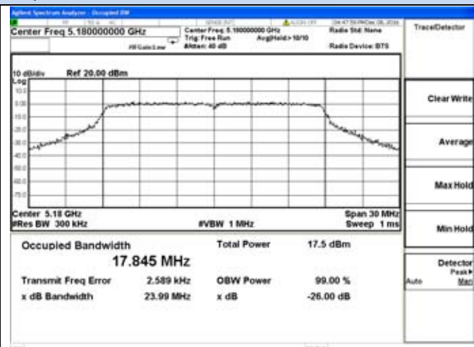
802.11n20-5180MHz
