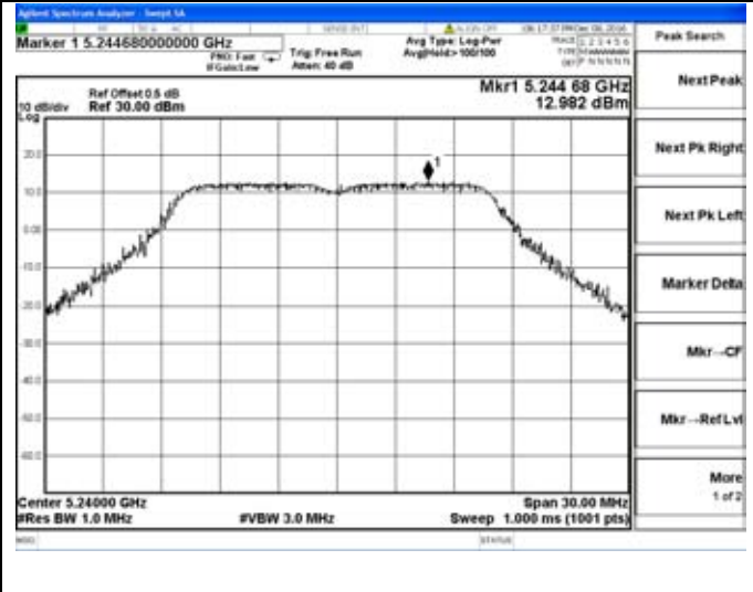
Chain 1-802.11a-5240MHz
