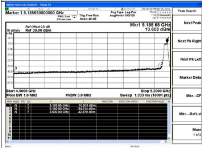
802.11a-5180MHz-Lower
