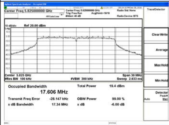
802.11n20-5825MHz
