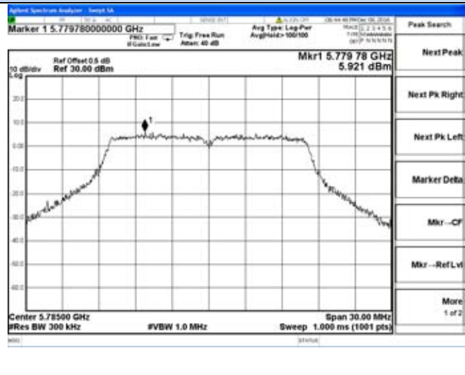
Chain 1-802.11a-5785MHz
