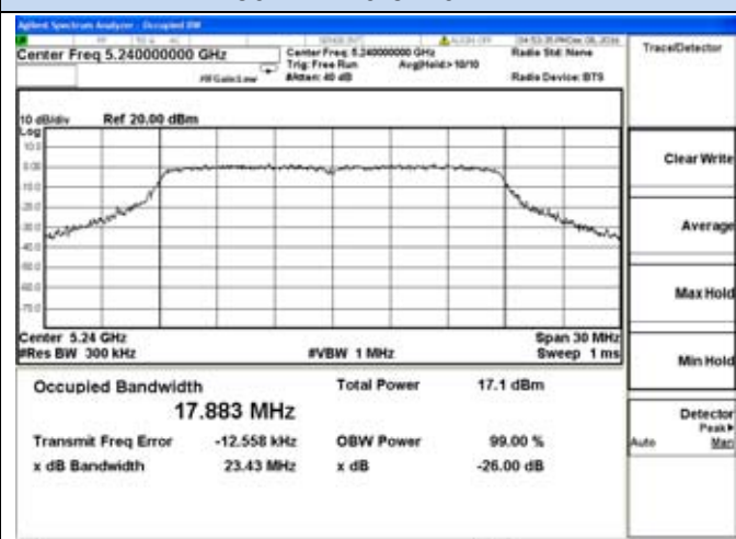
802.11n20-5240MHz
