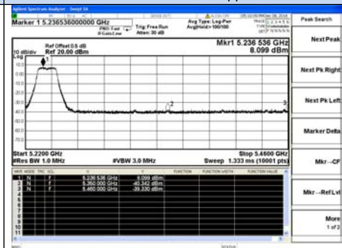
802.11n20-5240MHz-Upper
