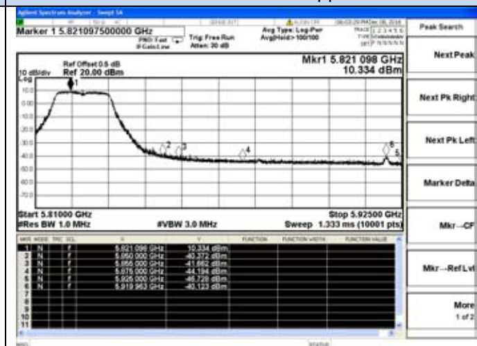
802.11n20-5825MHz-Upper
