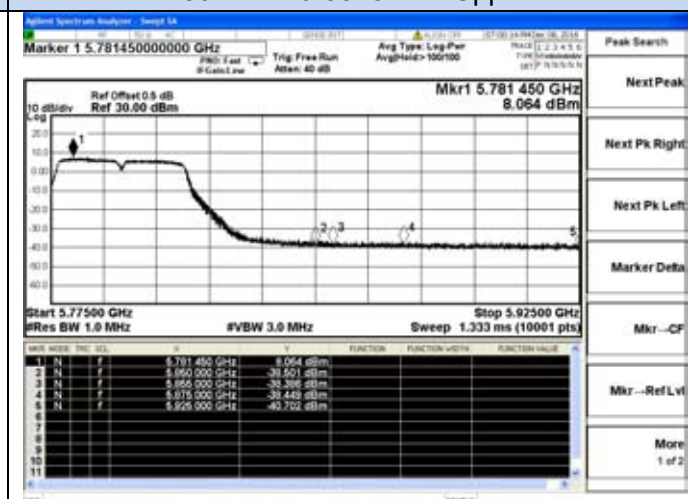
802.11n40-5795MHz-Upper
