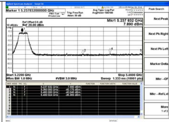
802.11a-5240MHz-Upper
