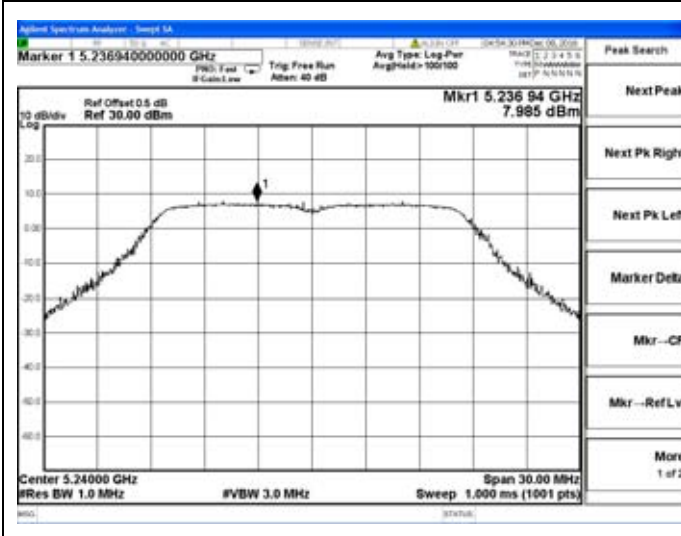
Chain 0-802.11n20-5240MHz
