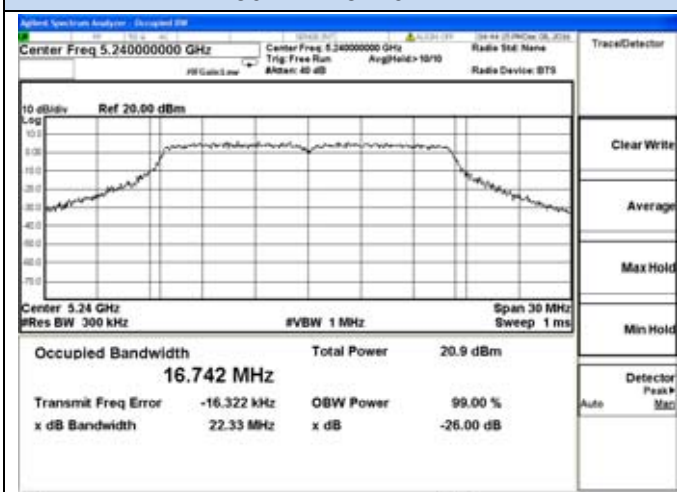
802.11a-5240MHz
