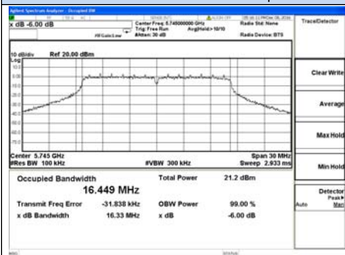
802.11a-5745MHz
