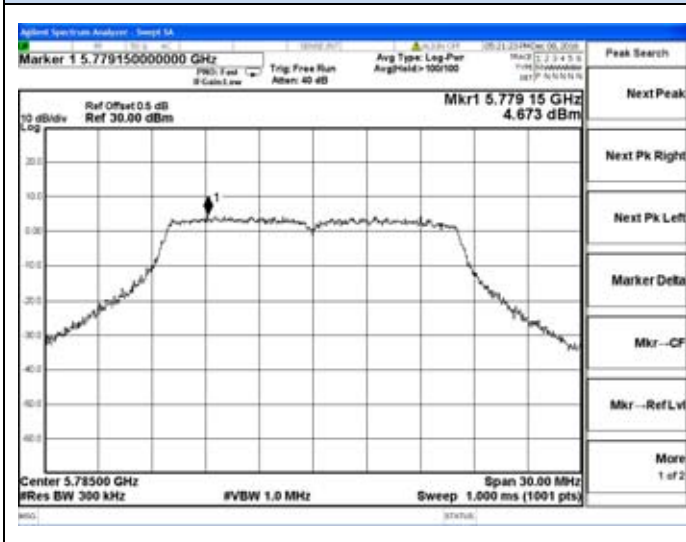
Chain 0-802.11a-5785MHz
