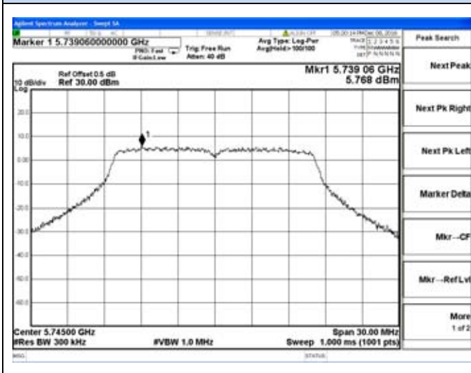
Chain 0-802.11a-5745MHz
