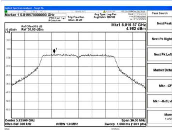
Chain 0-802.11a-5825MHz
