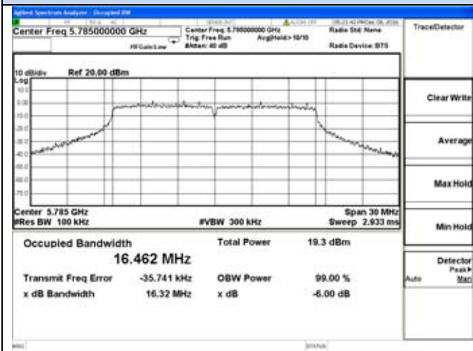
802.11a-5785MHz
