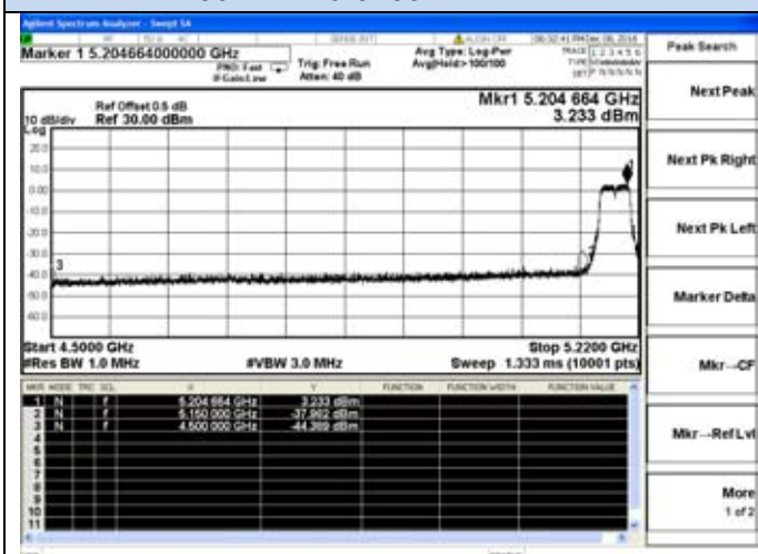
802.11n40-5190MHz-Lower
