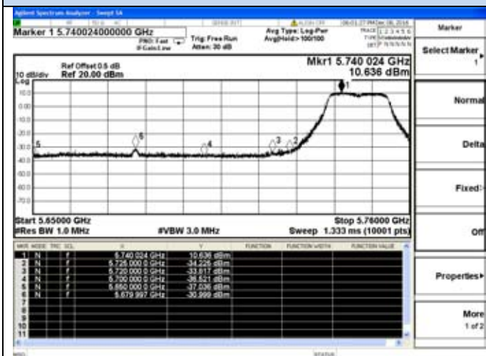
802.11n20-5745MHz-Lower
