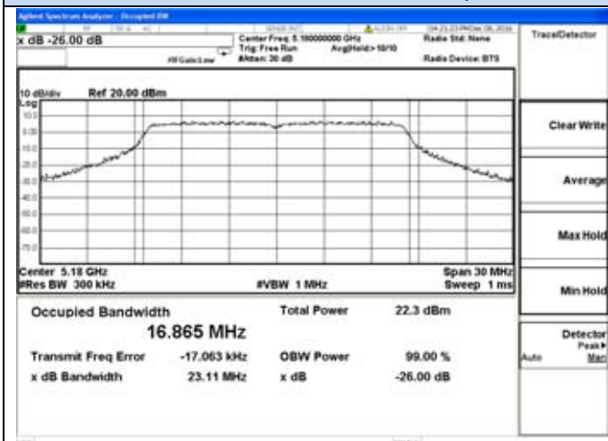
802.11a-5180MHz
