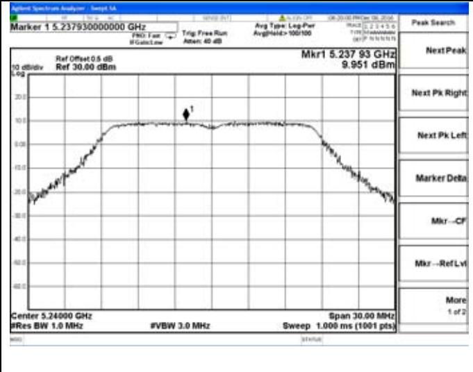
Chain 1-802.11n20-5240MHz
