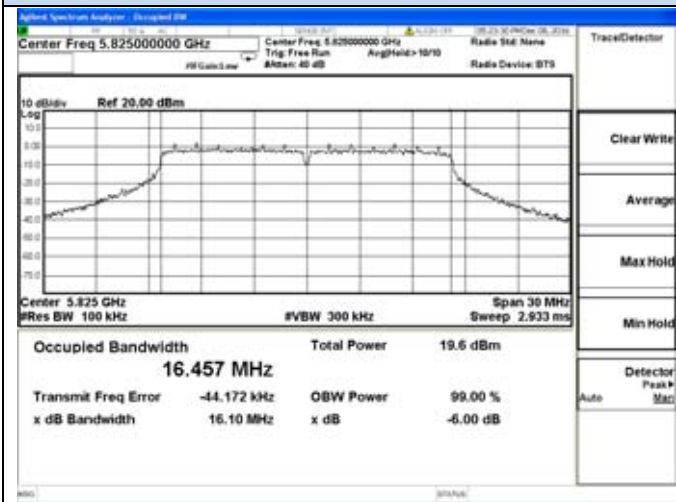
802.11a-5825MHz
