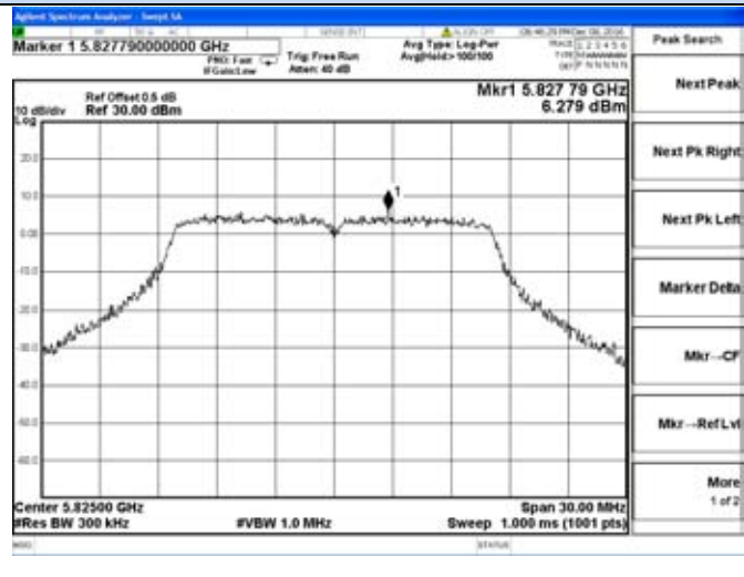
Chain 1-802.11a-5825MHz
