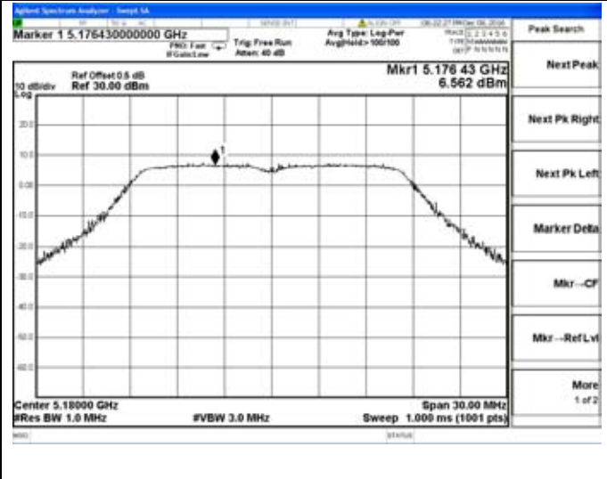
Chain 1-802.11n20-5180MHz
