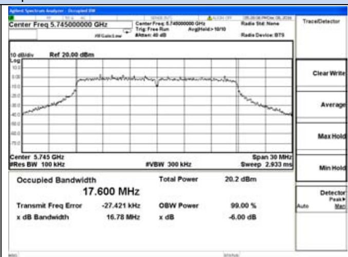
802.11n20-5745MHz
